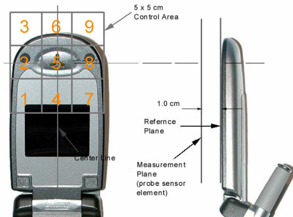
Figure 12 E/H-Field Emissions Test Setup Diagram
