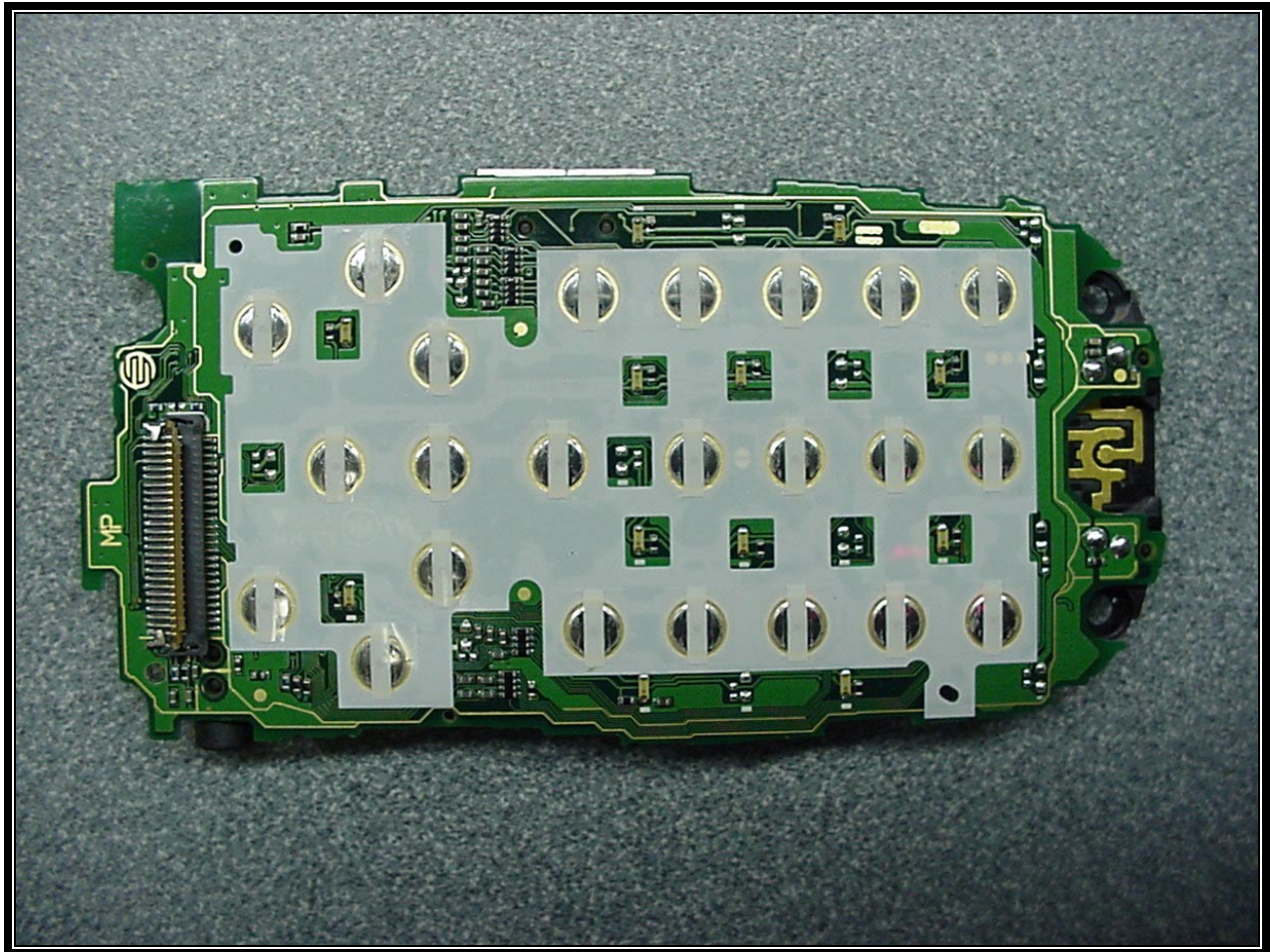
PHOTOGRAPH 32: FRONT OF PCB
