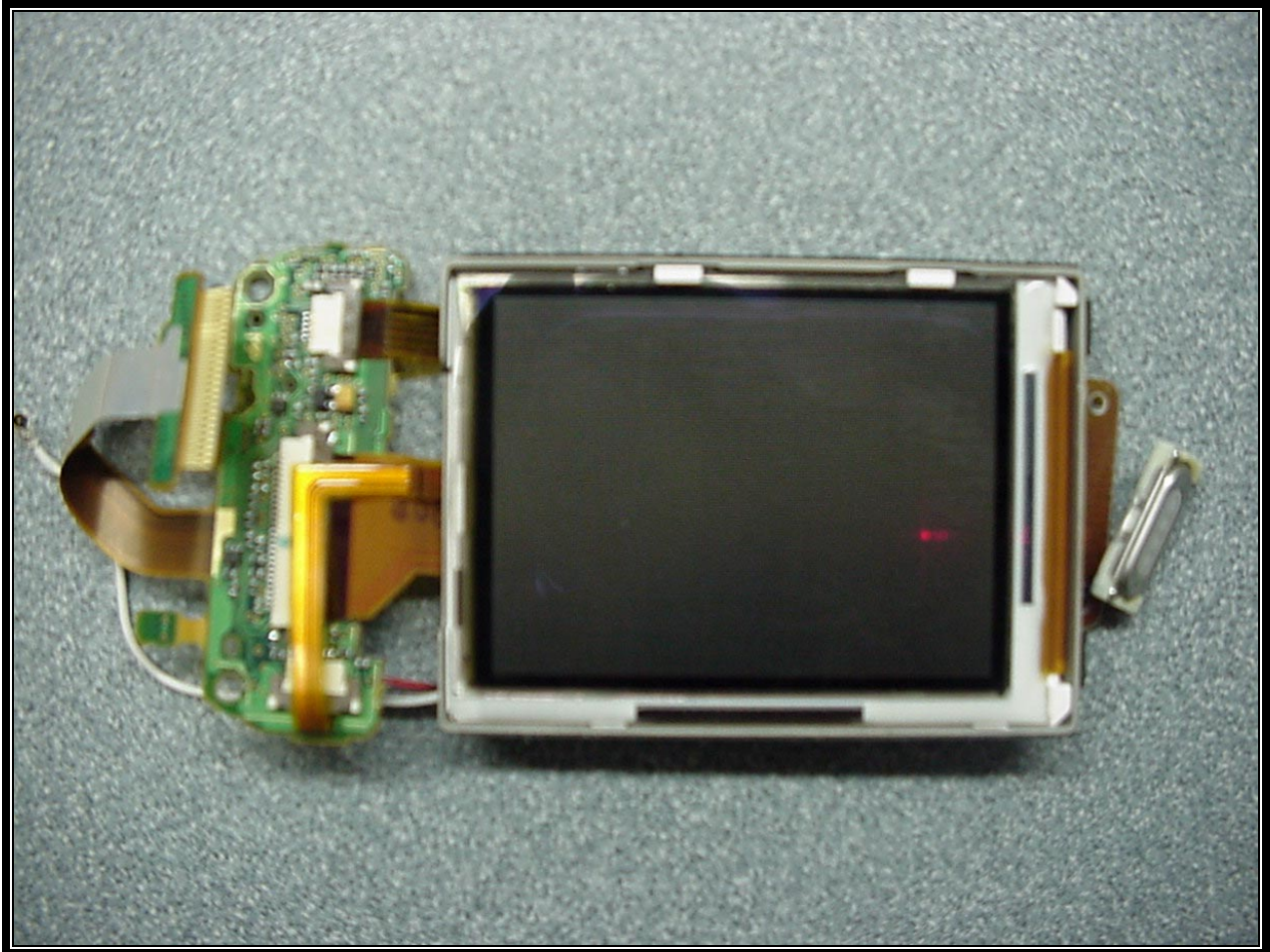
PHOTOGRAPH 37: FRONT OF LCD ASSEMBLY
