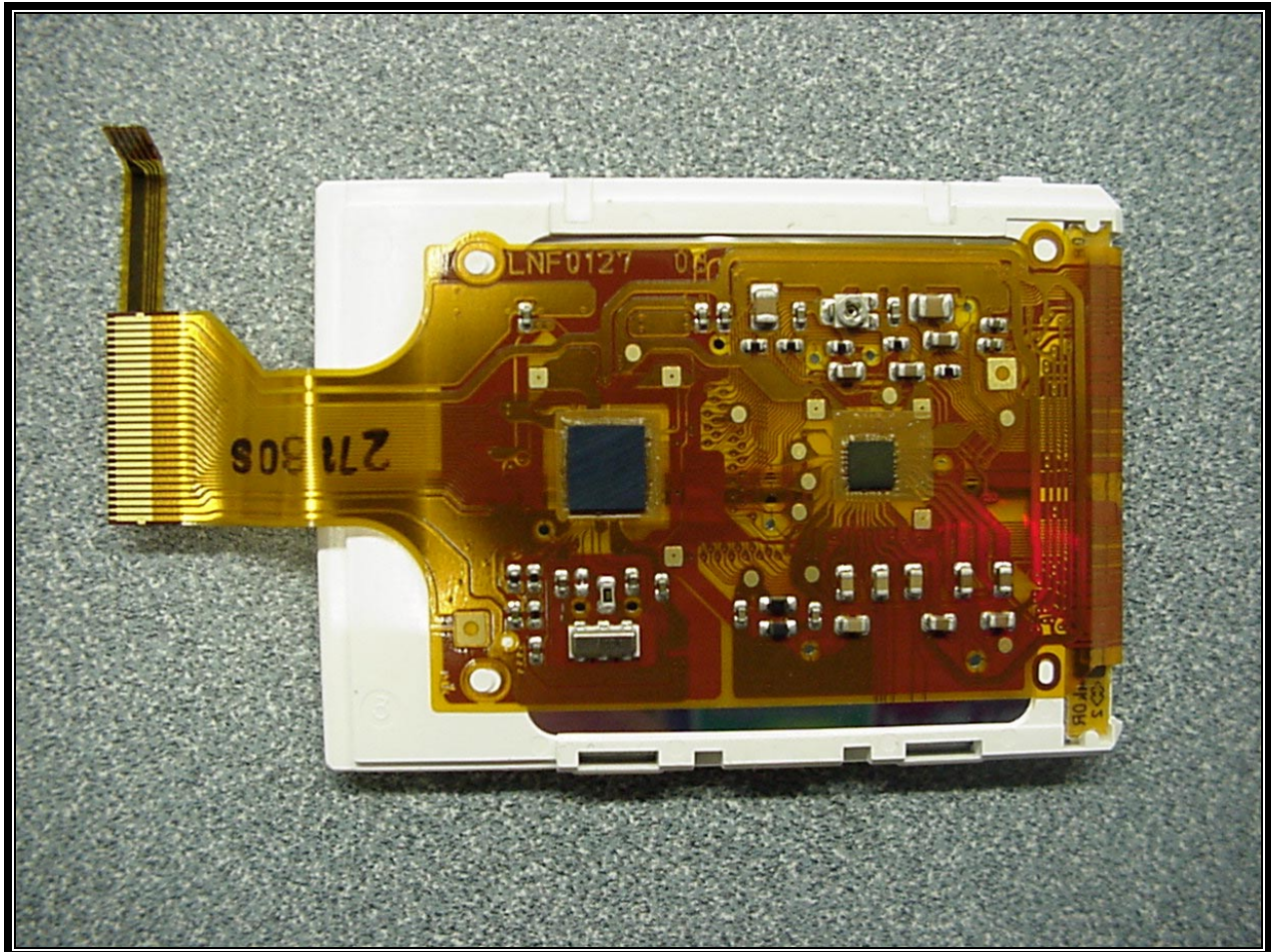
PHOTOGRAPH 36: BOTTOM OF LCD
