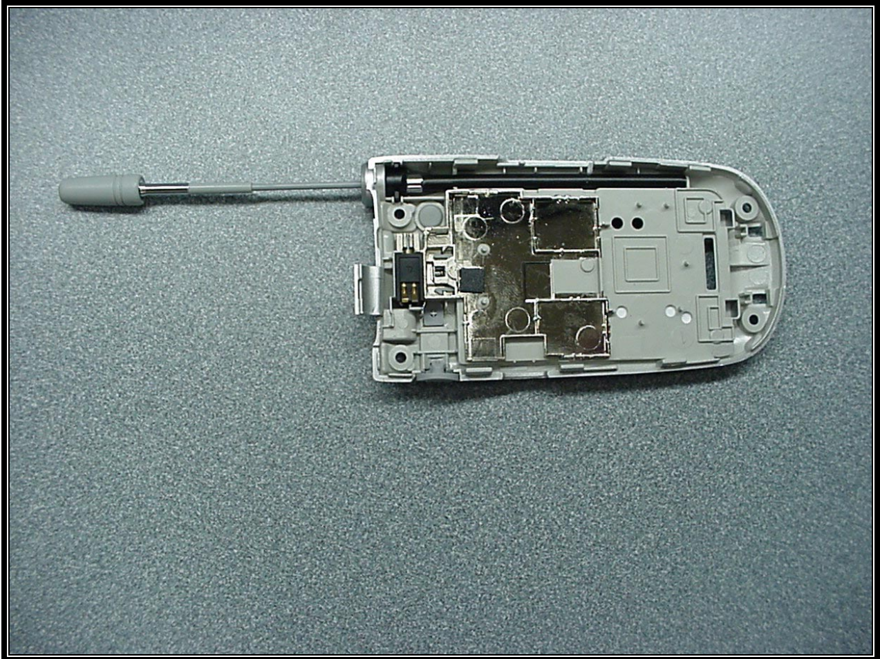
PHOTOGRAPH 26: INSIDE BACK BEZEL
