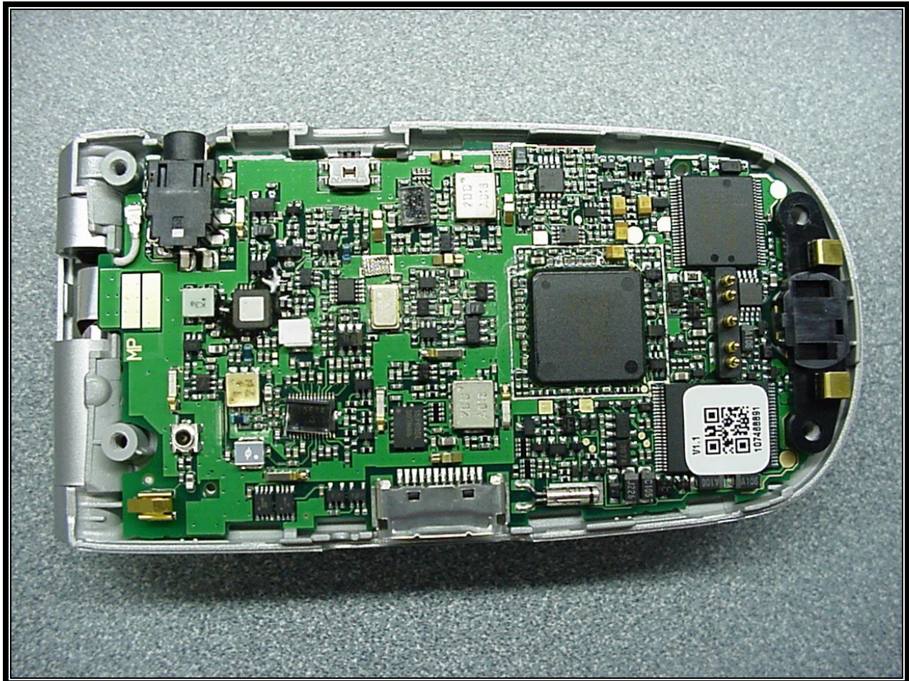
PHOTOGRAPH 31: BACK OF PCB INSIDE CASE
