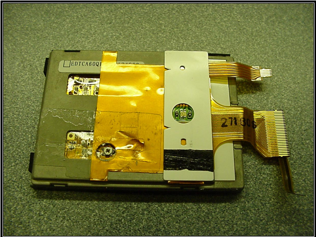
PHOTOGRAPH 35: BACK OF LCD WITH SHIELD
