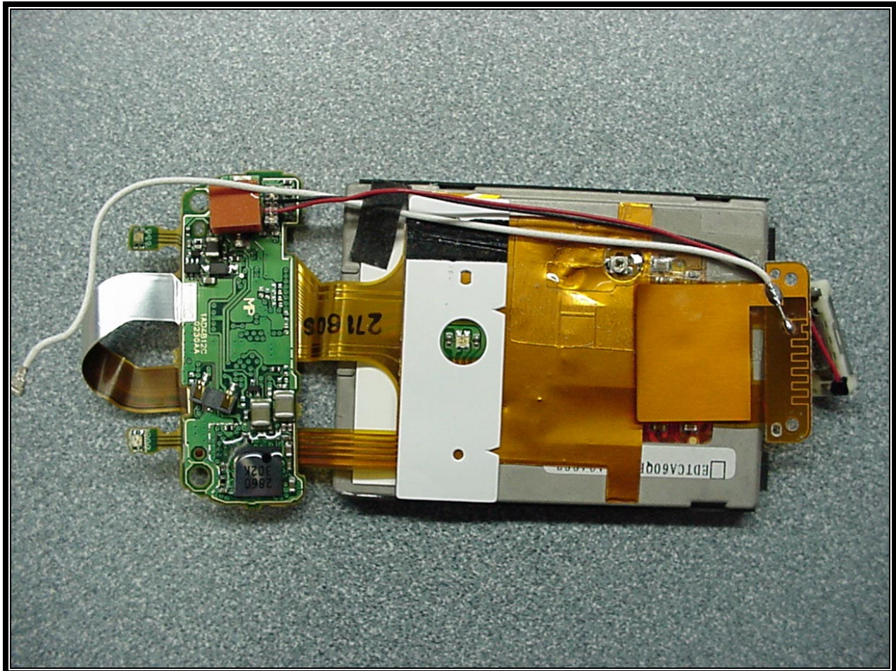
PHOTOGRAPH 38: BACK OF LCD ASSEMBLY
