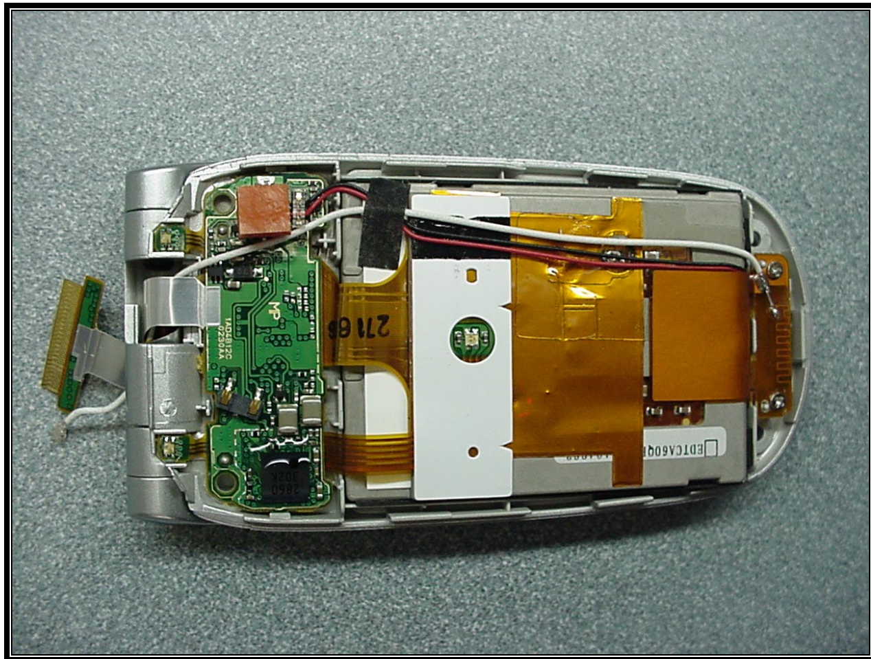
PHOTOGRAPH 24: INSIDE FRONT COMPARTMENT
