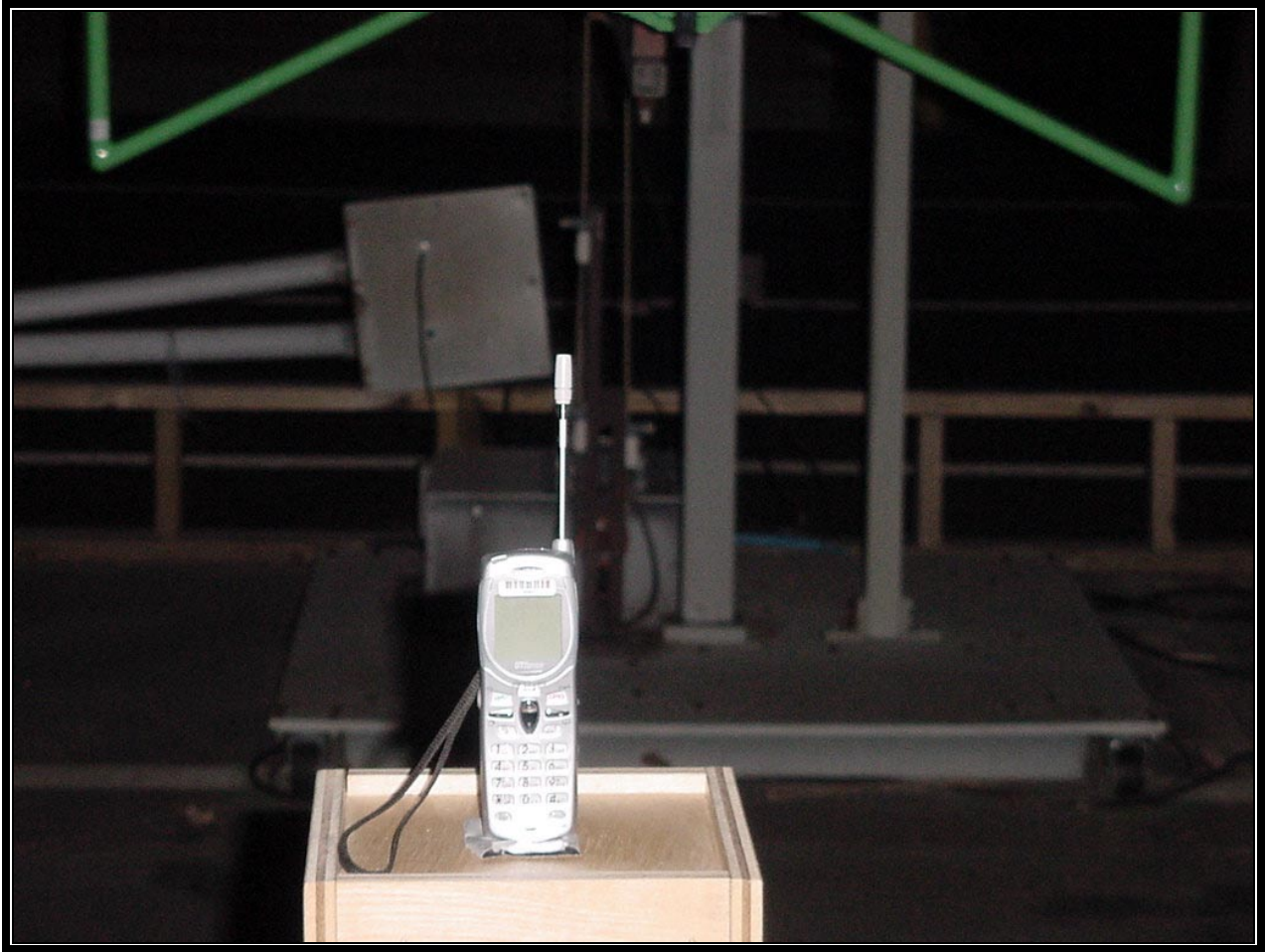
PHOTOGRAPH 2: RADIATED FRONT VIEW
