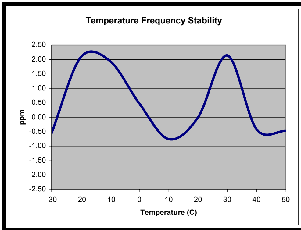
PLOT 9-1: TEMPERATURE FREQUENCY STABILITY - §2.1055
