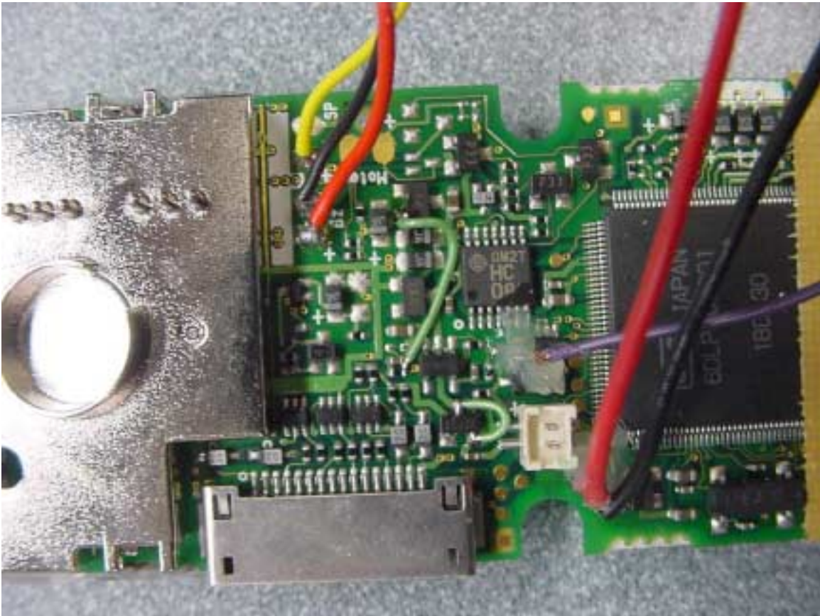
PHOTOGRAPH 25: CONNECTIONS ON MID RF PCB
