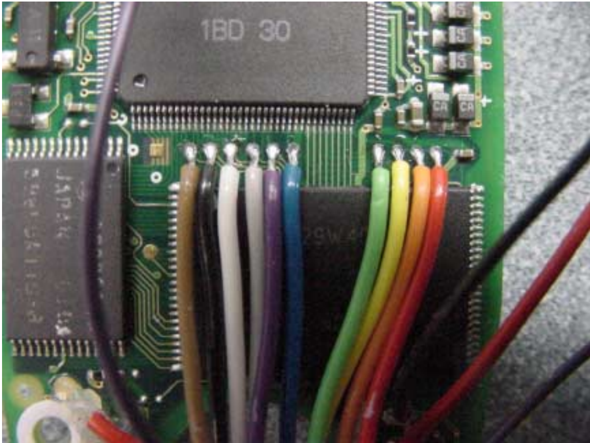
PHOTOGRAPH 28: CONNECTIONS AT LOWER SIDE OF RF PCB
