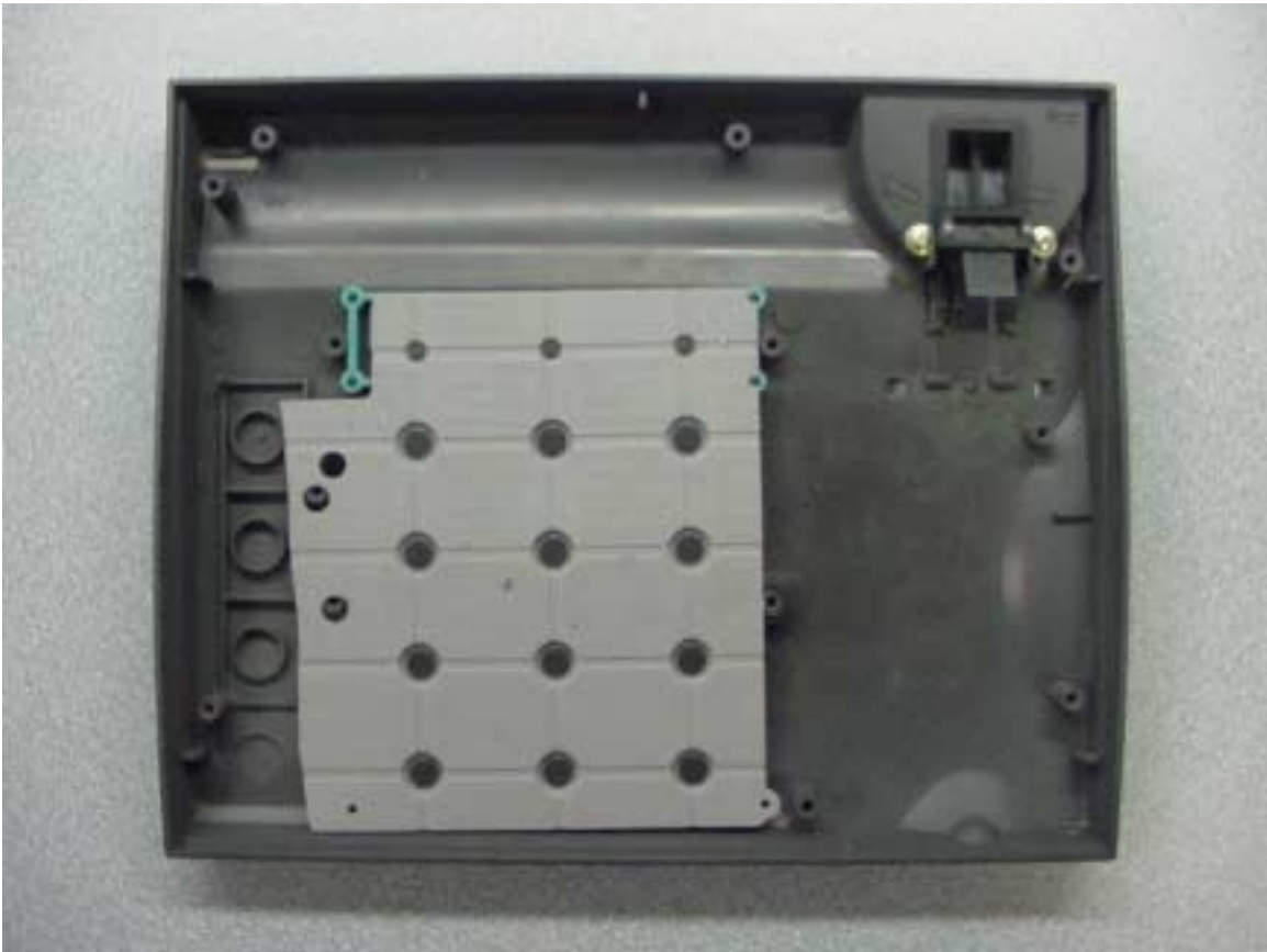
PHOTOGRAPH 16: INSIDE TOP CASE WITH BOTTOM OF KEYPAD
