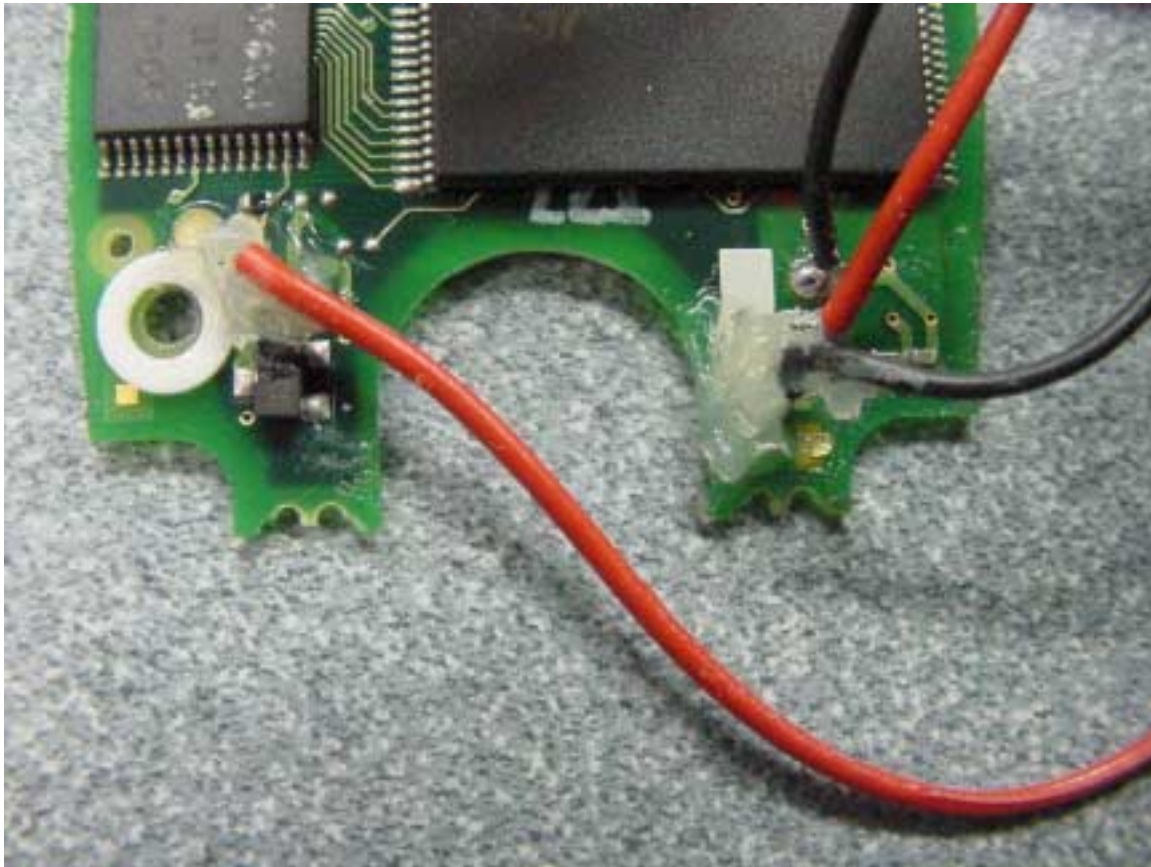
PHOTOGRAPH 29: CONNECTIONS AT LOWER END OF RF PCB
