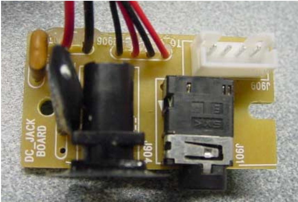
PHOTOGRAPH 22: TOP OF DC POWER PCB
