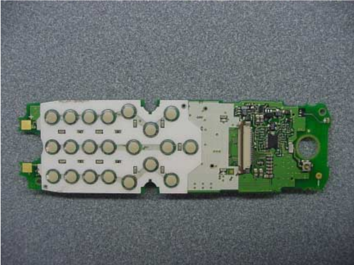
PHOTOGRAPH 43: KEYPAD SIDE OF RF PCB WITHOUT LCD
