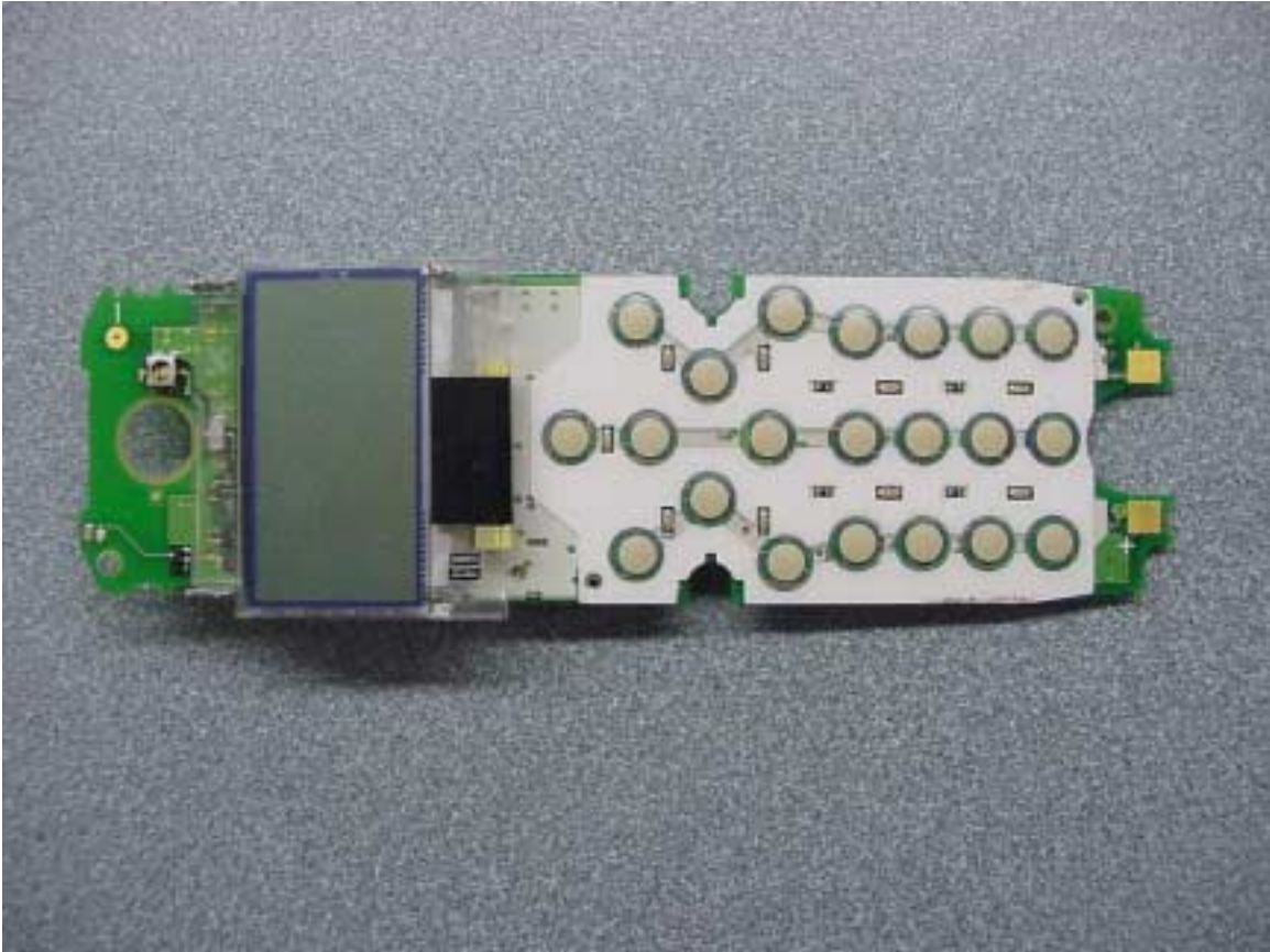
PHOTOGRAPH 42: LCD/KEYPAD SIDE OF RF PCB
