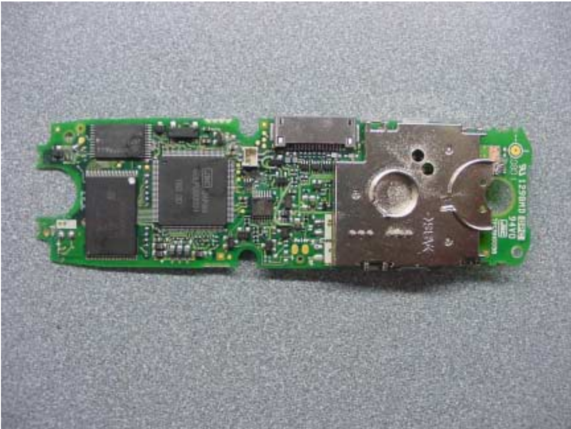
PHOTOGRAPH 41: COMPONENT SIDE OF RF PCB
