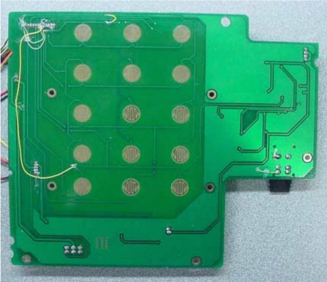
PHOTOGRAPH 21: TOP OF KEYPAD PCB
