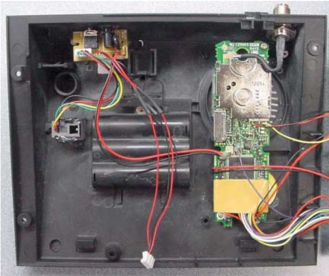
PHOTOGRAPH 18: INSIDE BOTTOM OF CASE WITH RF, POWER PCB'S, AND CONNECTOR
