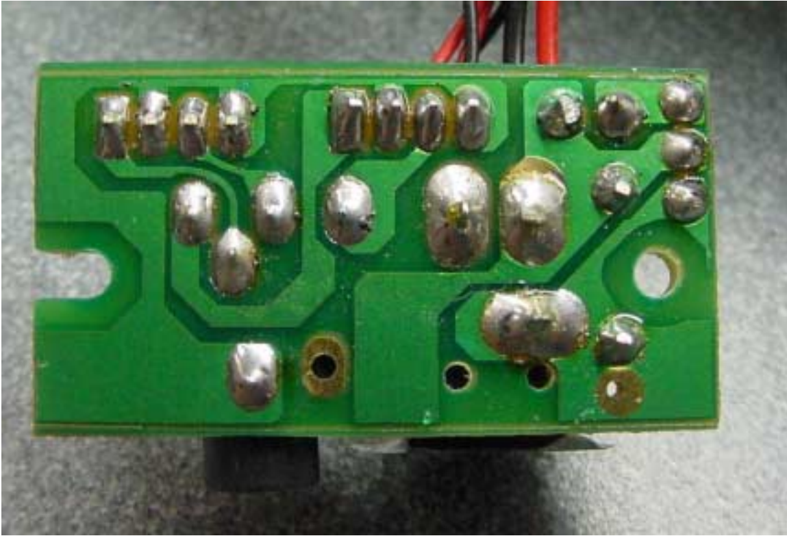
PHOTOGRAPH 23: BOTTOM OF DC POWER PCB
