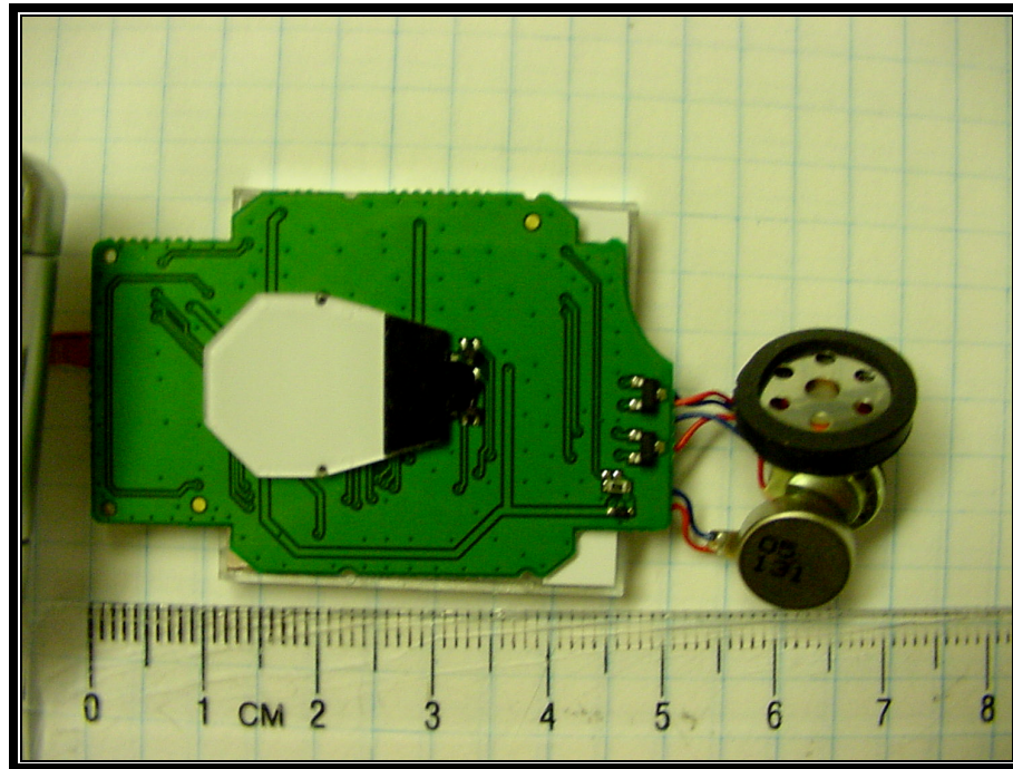
PHOTOGRAPH 27: BACK OF LCD PCB
