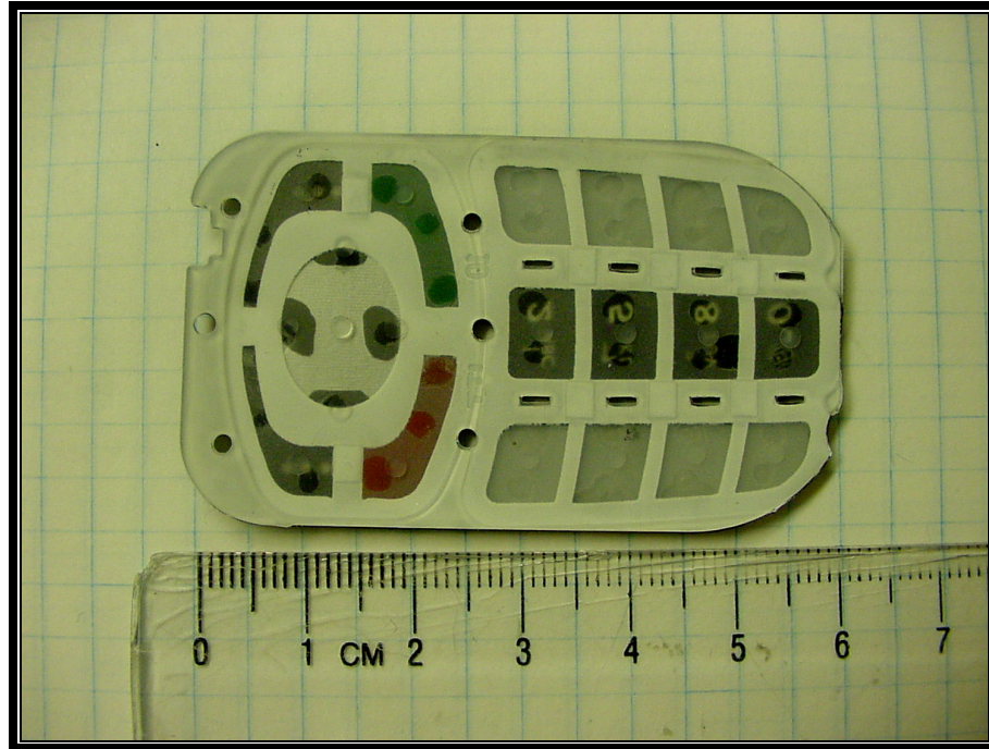
PHOTOGRAPH 25: BACK OF KEYPAD
