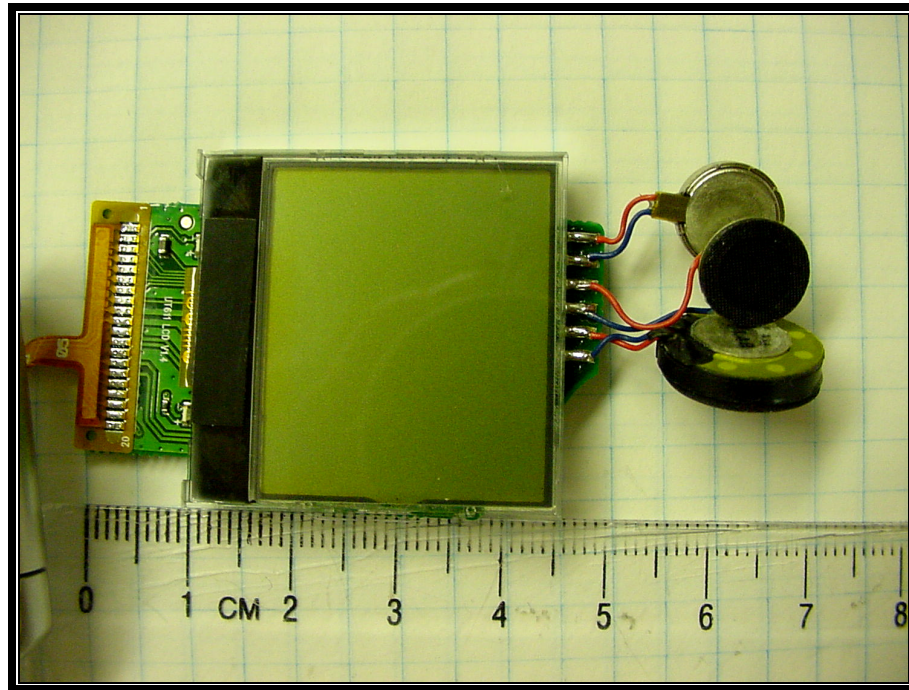
PHOTOGRAPH 26: FRONT OF LCD PCB
