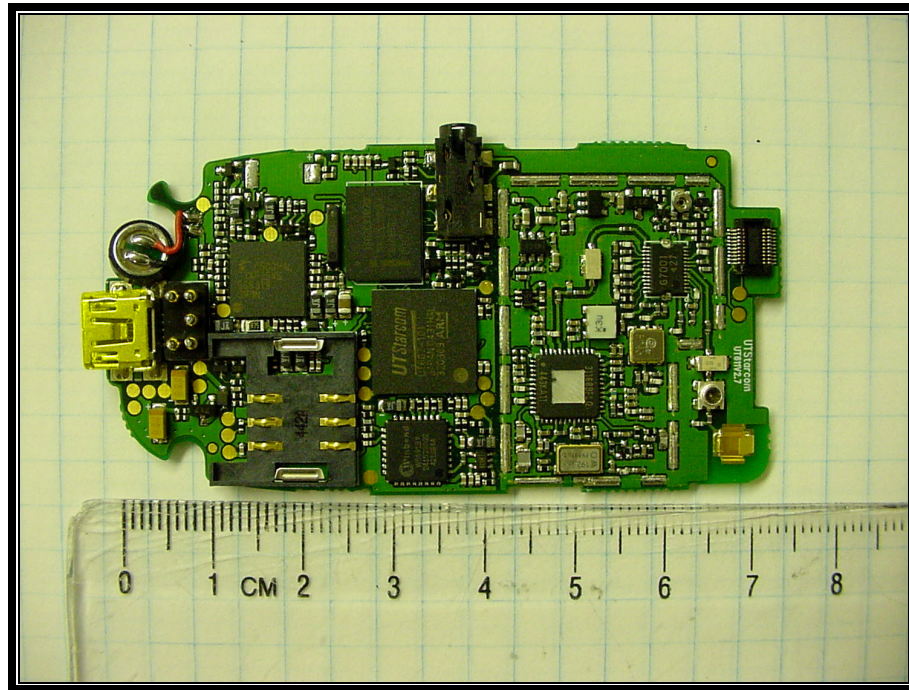
PHOTOGRAPH 23: BACK OF PCB WITHOUT SHIELDS
