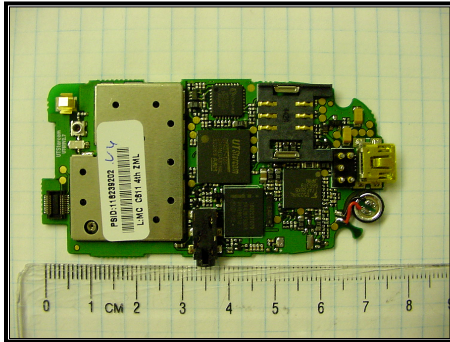
PHOTOGRAPH 22: BACK OF PCB
