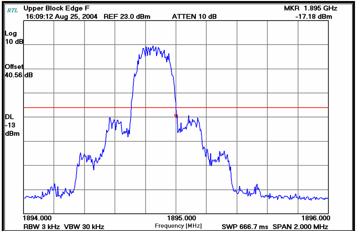
PLOT 7-4: UPPER BAND EDGE BLOCK F
