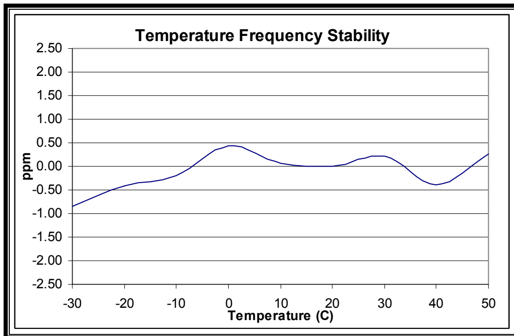
PLOT 8-1: TEMPERATURE FREQUENCY STABILITY DATA - §2.1055
