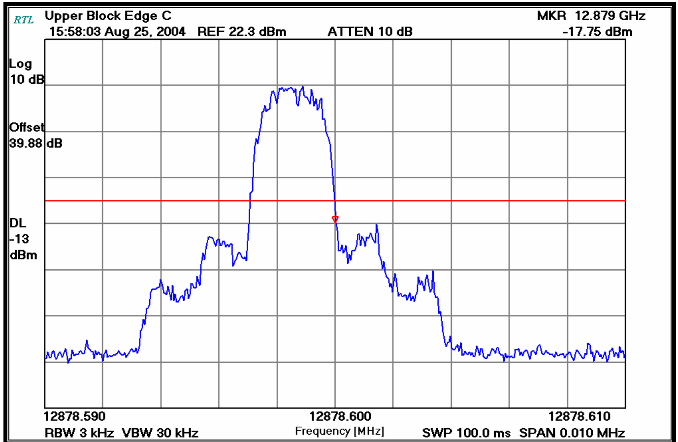
PLOT 7-6: UPPER BAND EDGE BLOCK C
