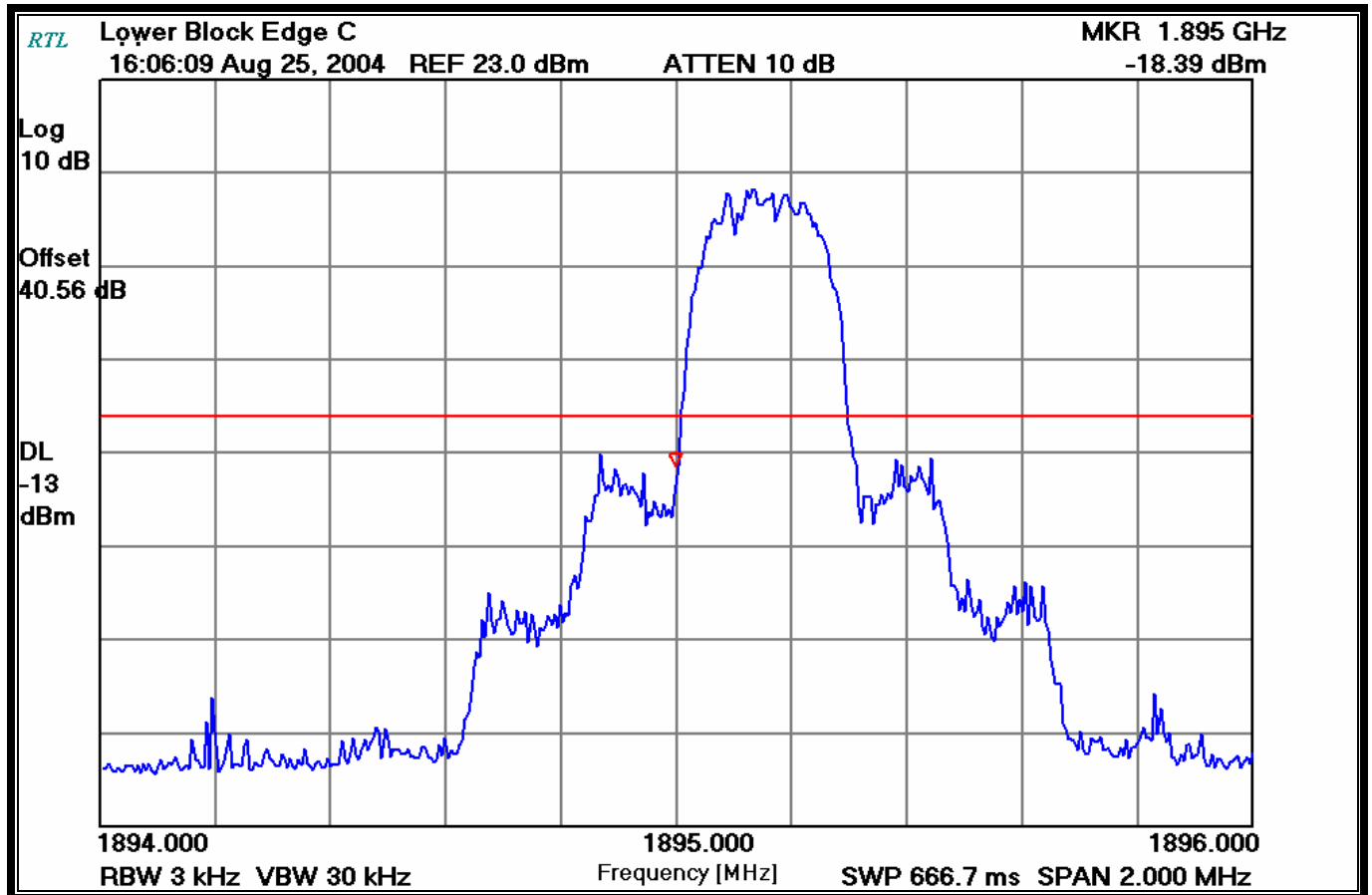
PLOT 7-5: LOWER BAND EDGE BLOCK C
