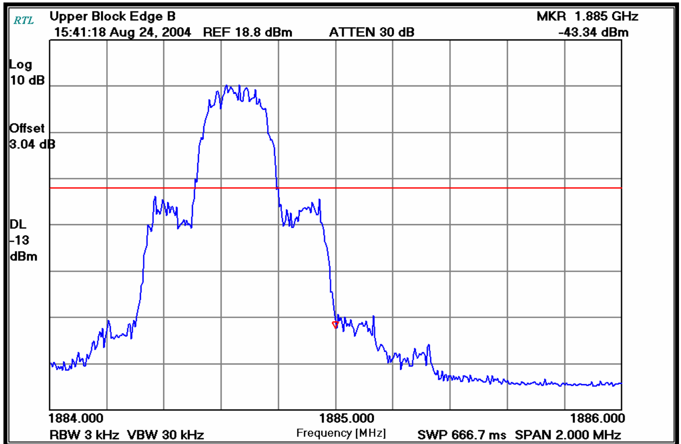
PLOT 7-2: UPPER BAND EDGE BLOCK B
