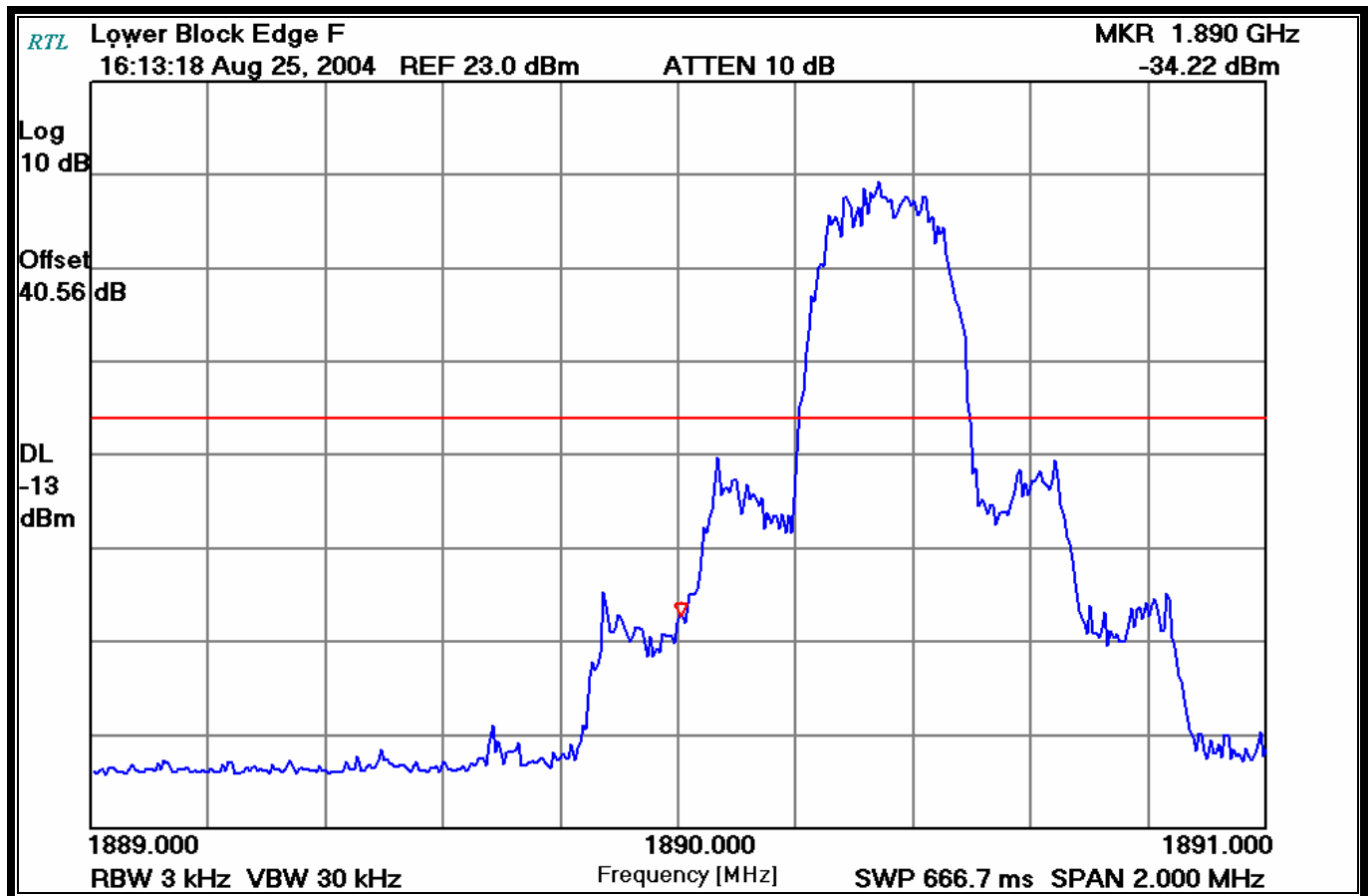
PLOT 7-3: LOWER BAND EDGE BLOCK F
