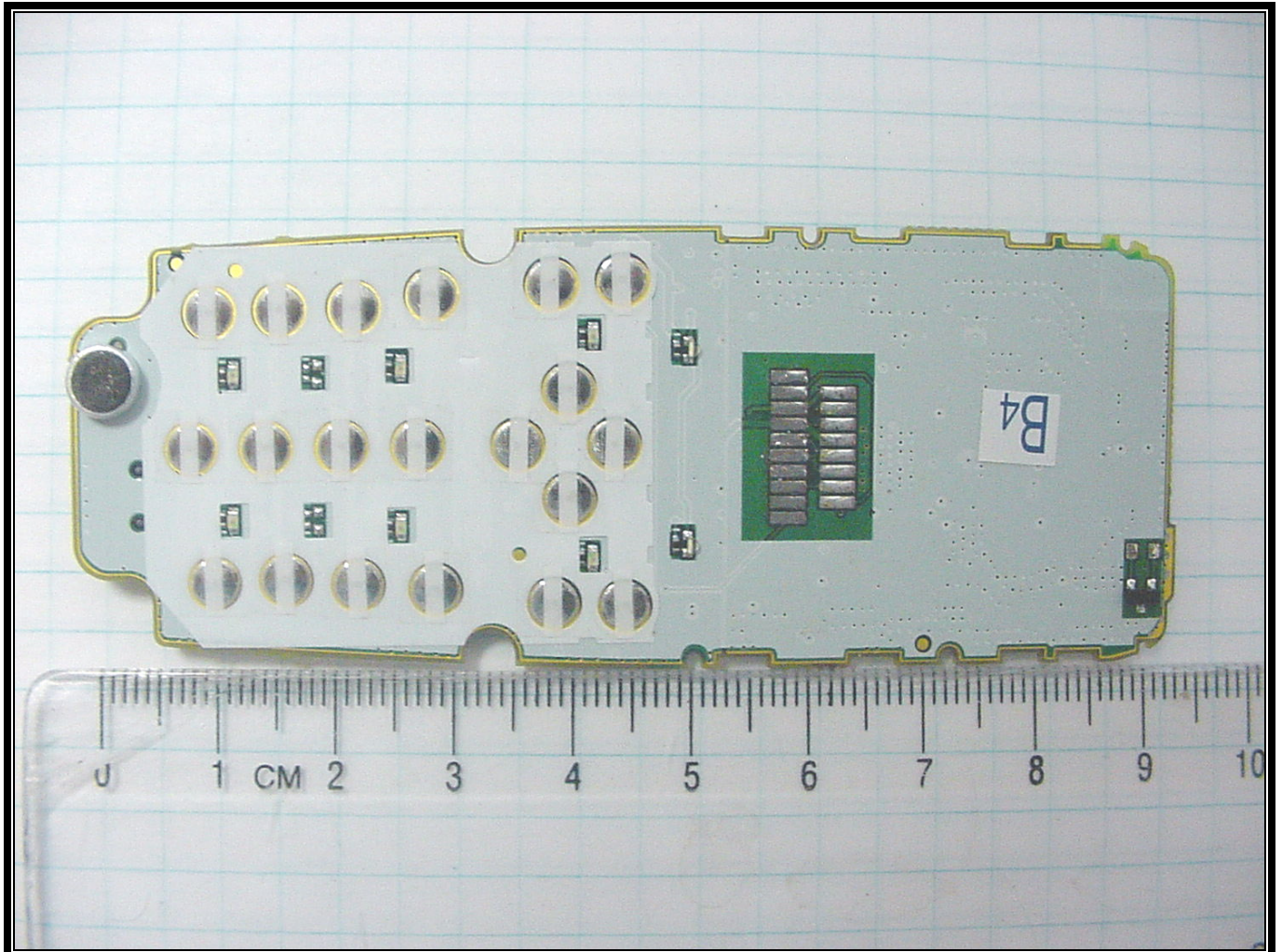
PHOTOGRAPH 19: FRONT OF PCB
