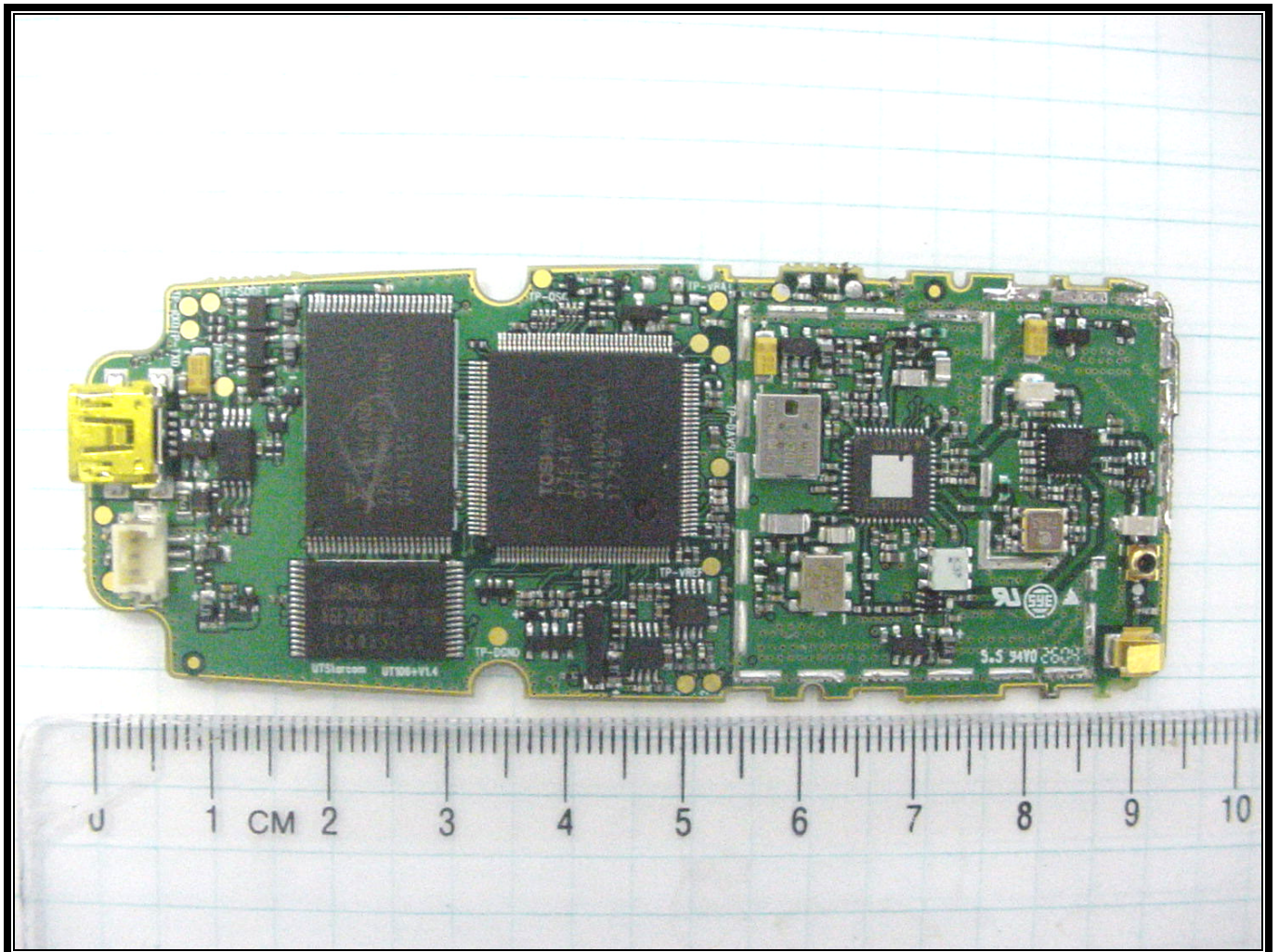
PHOTOGRAPH 18: BACK OF PCB
