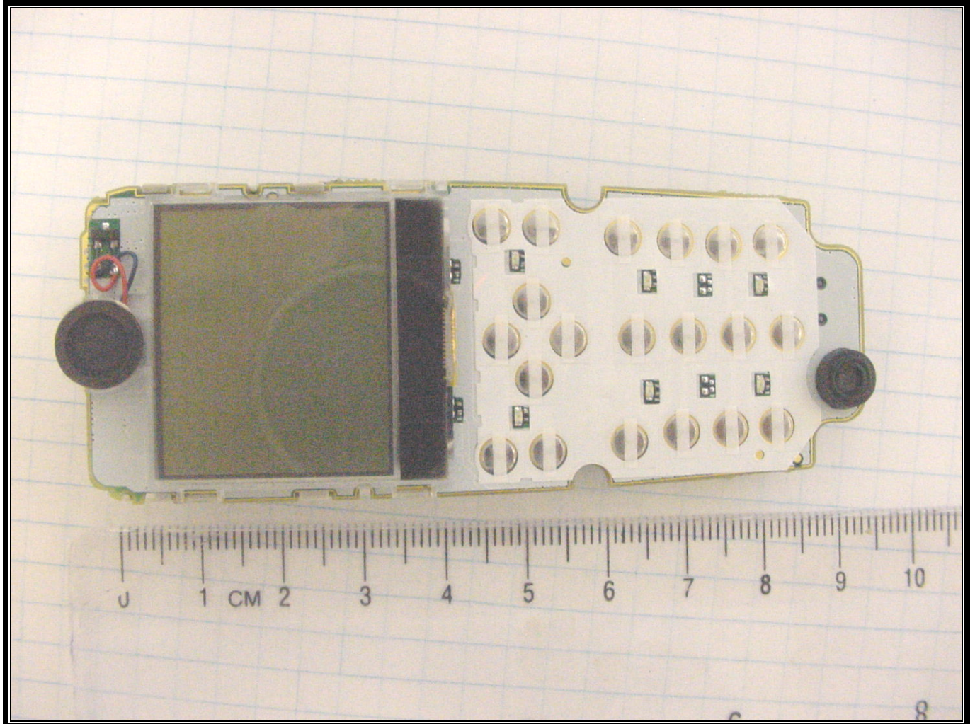
PHOTOGRAPH 17: FRONT OF PCB WITH LCD
