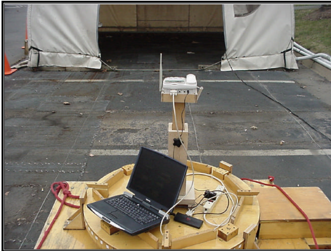
PHOTOGRAPH 3: RADIATED EMISSIONS – BACK VIEW
