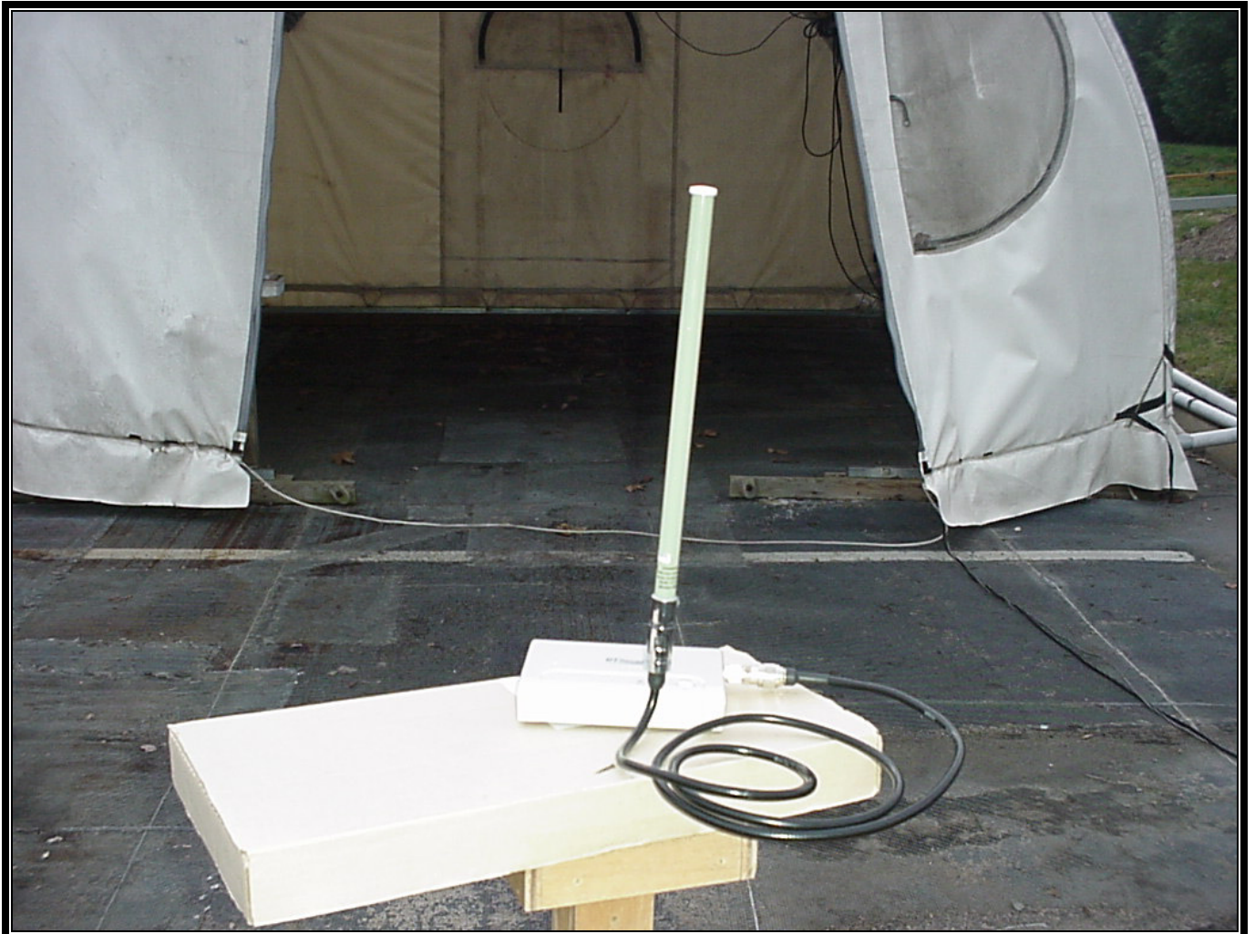
PHOTOGRAPH 7: RADIATED BACK VIEW WITH ROD ANTENNA
