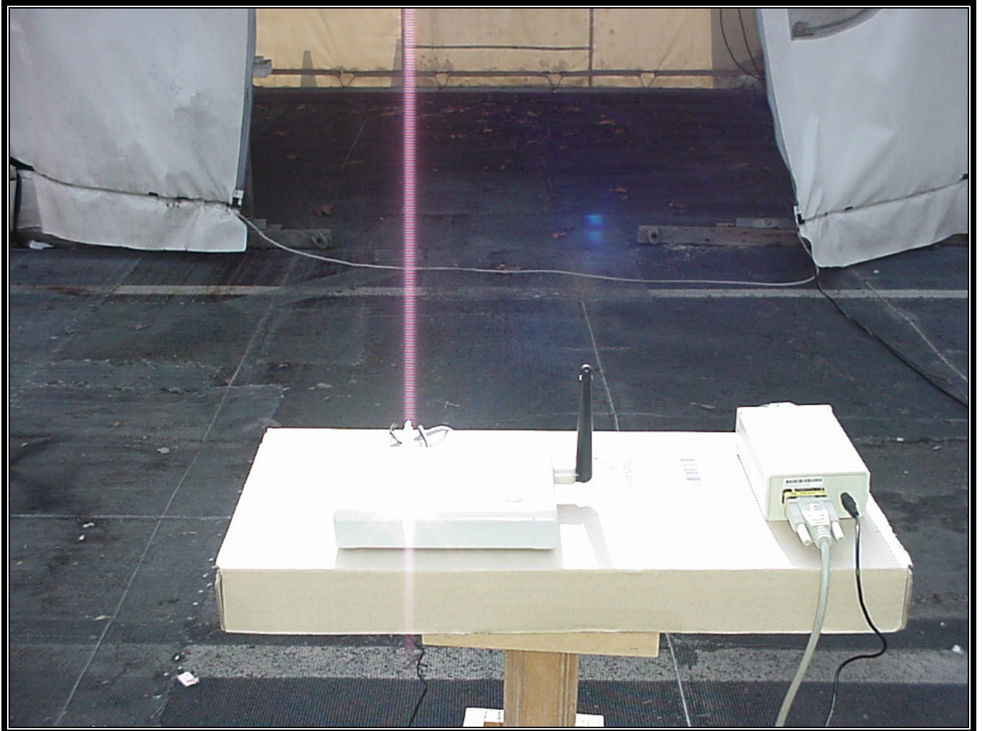
PHOTOGRAPH 2: RADIATED FRONT VIEW WITH WHIP ANTENNA
