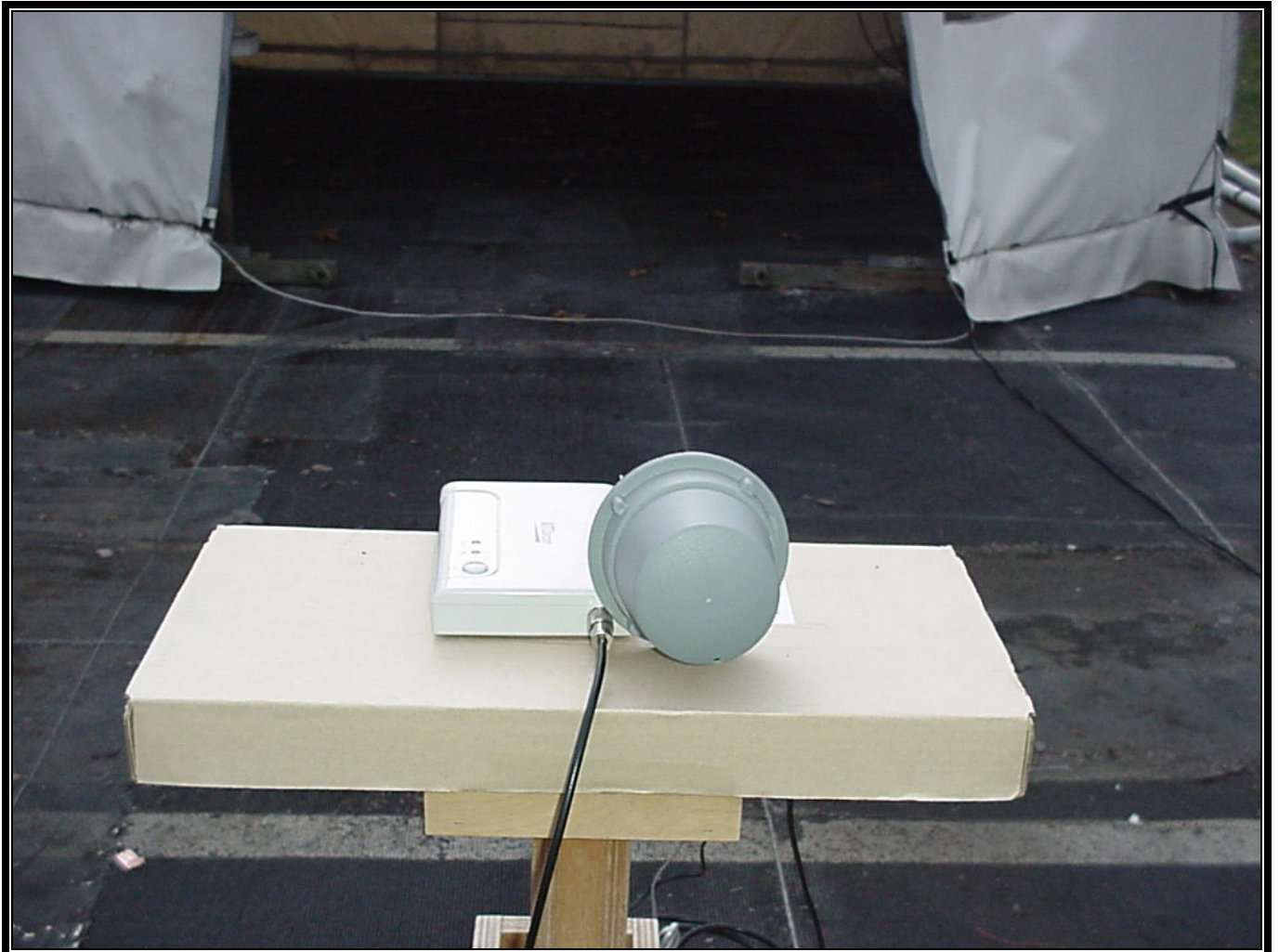
PHOTOGRAPH 4: RADIATED FRONT VIEW WITH PATCH ANTENNA
