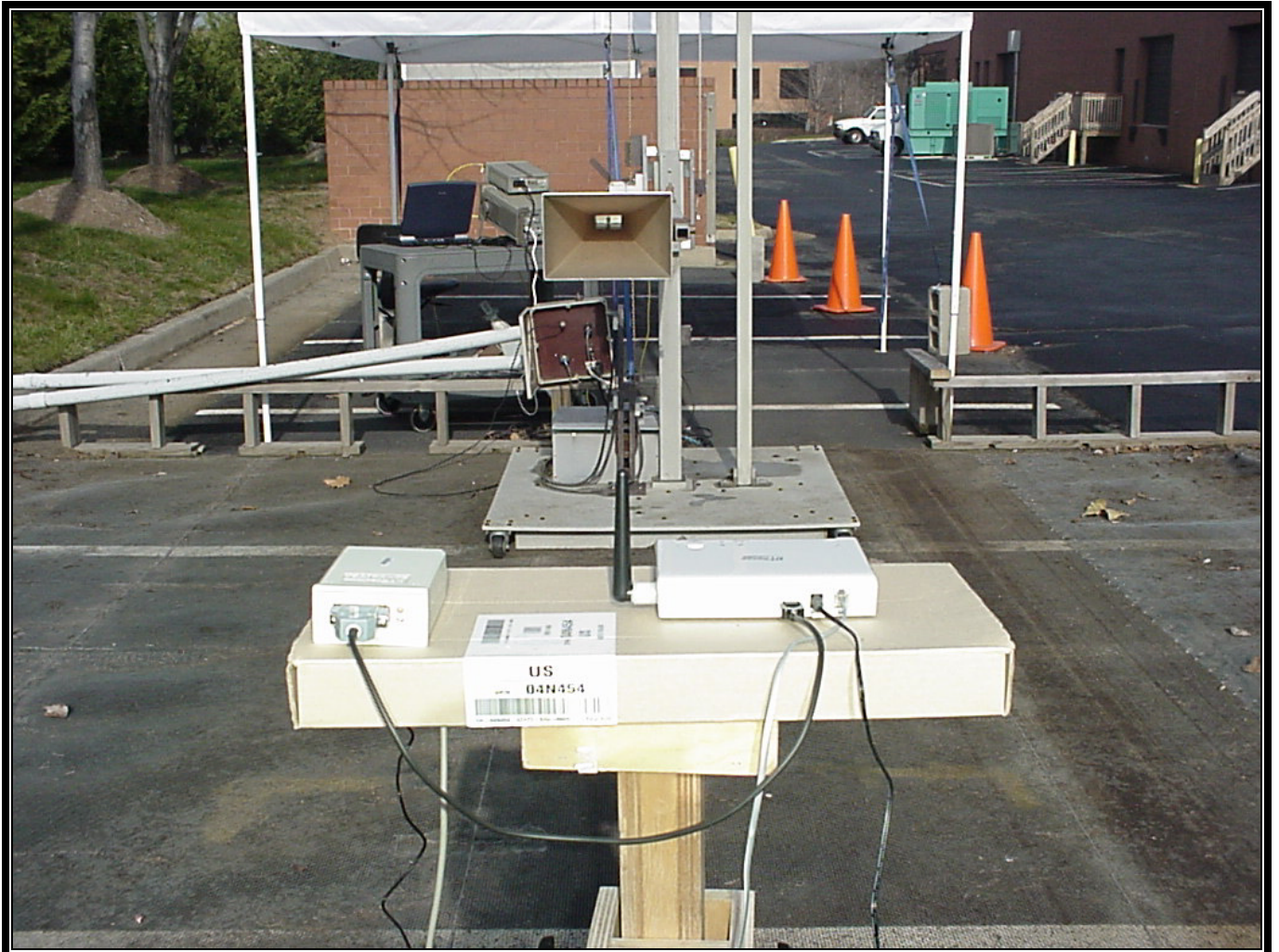
PHOTOGRAPH 3: RADIATED BACK VIEW WITH WHIP ANTENNA
