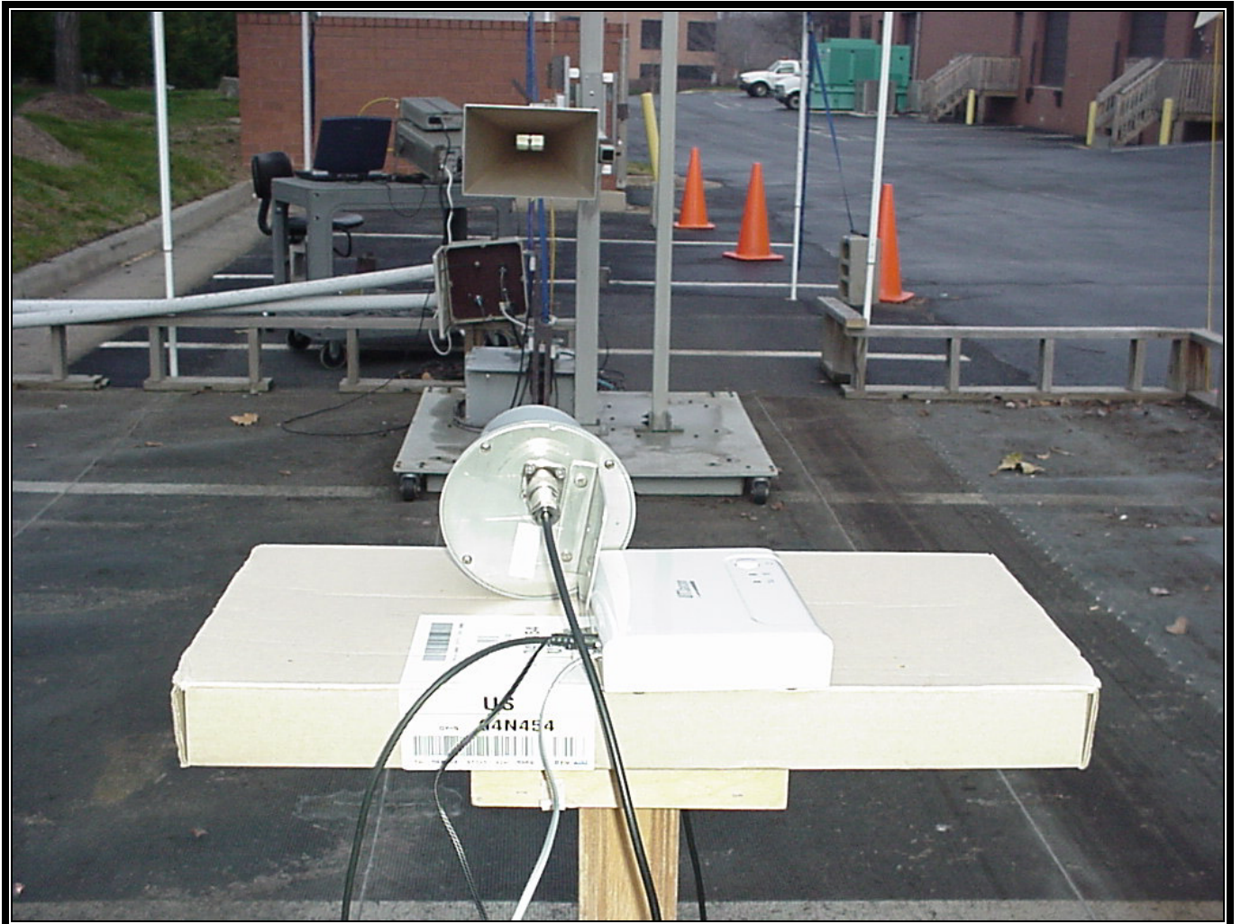
PHOTOGRAPH 5: RADIATED BACK VIEW WITH PATCH ANTENNA
