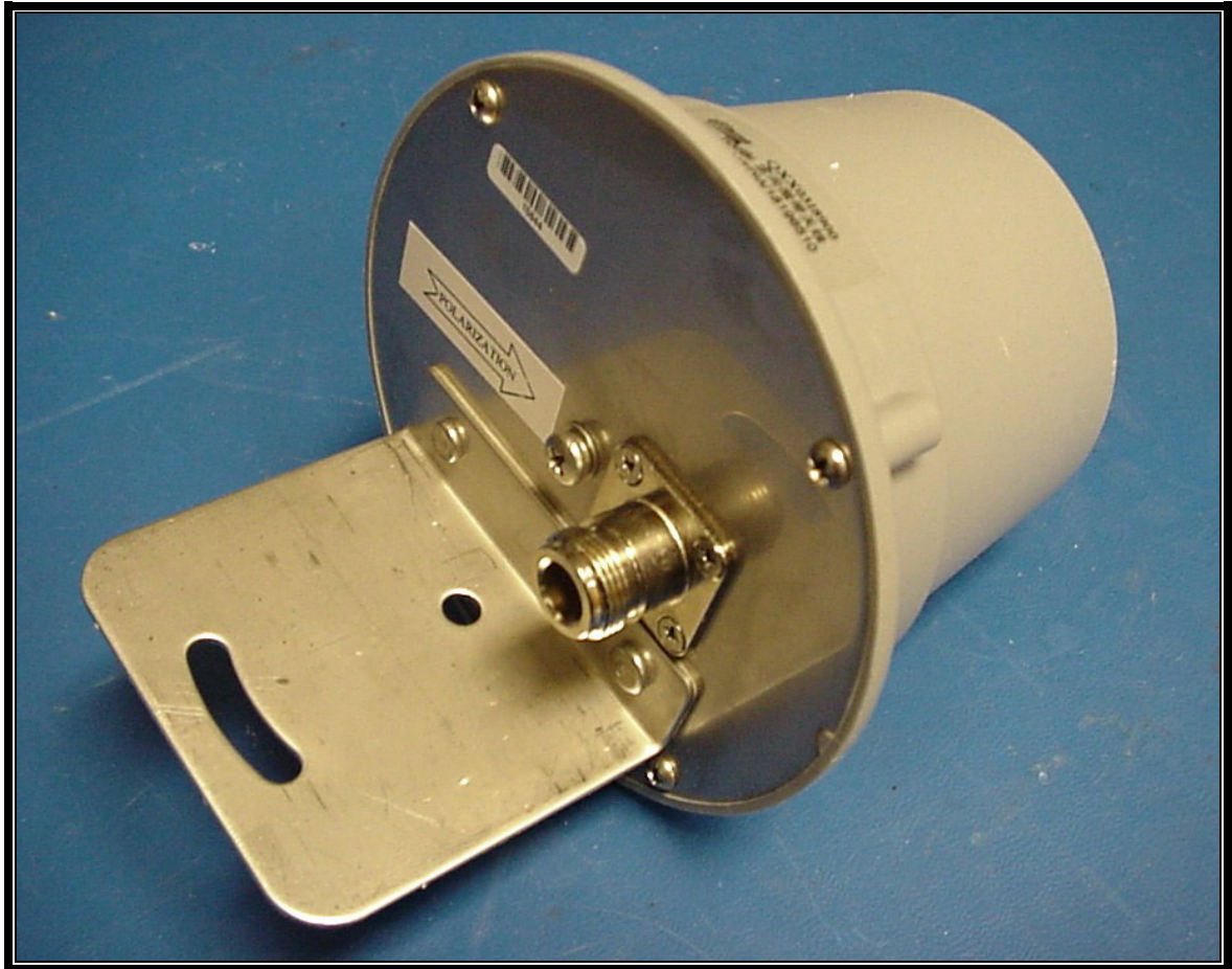
PHOTOGRAPH 13: PATCH ANTENNA
