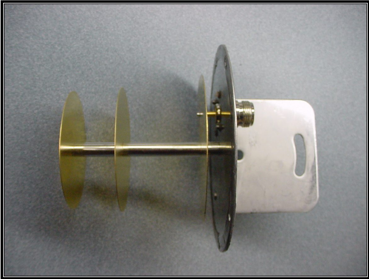
PHOTOGRAPH 13A: INSIDE PATCH ANTENNA
