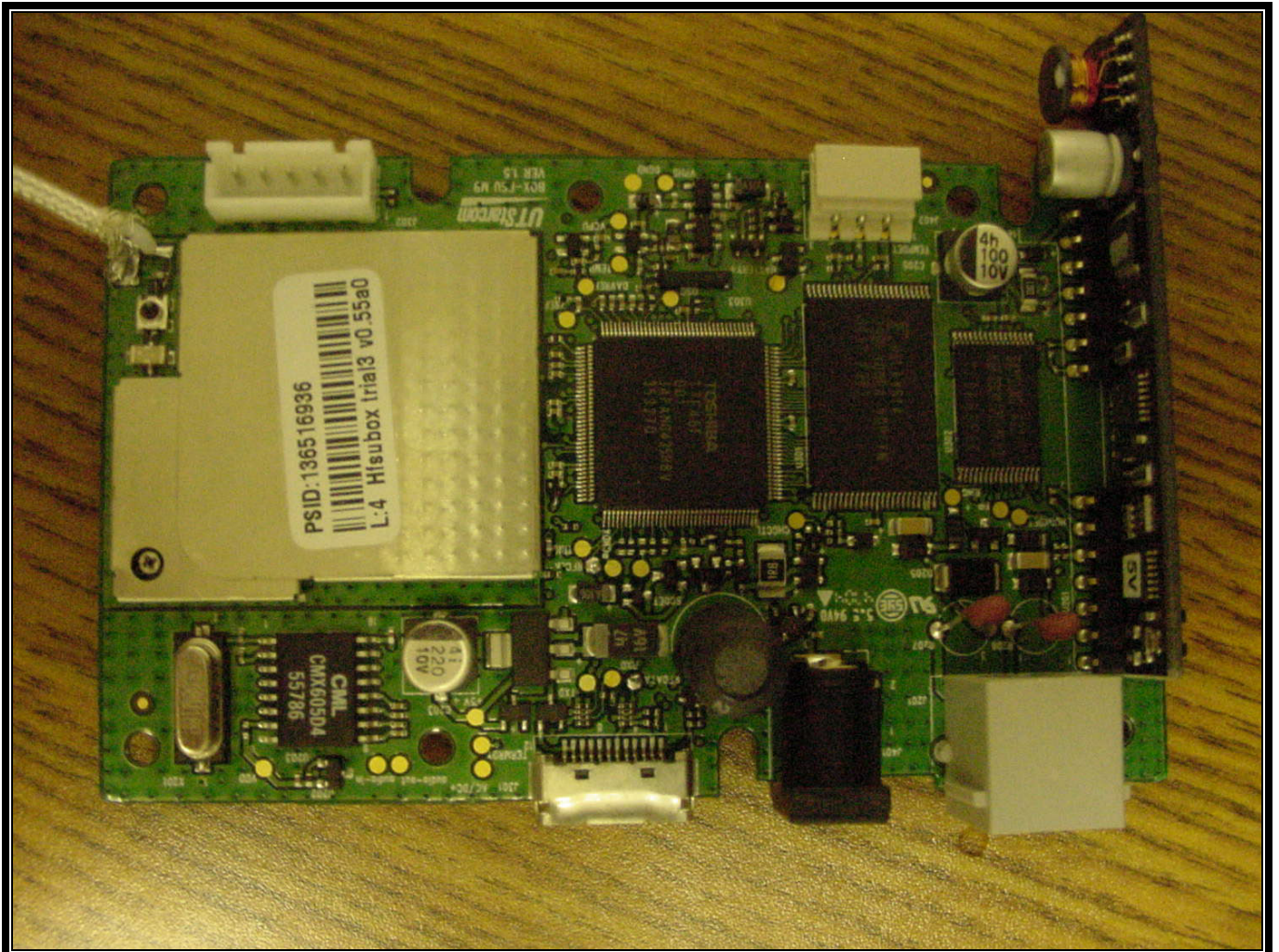
PHOTOGRAPH 19: TOP OF PCB
