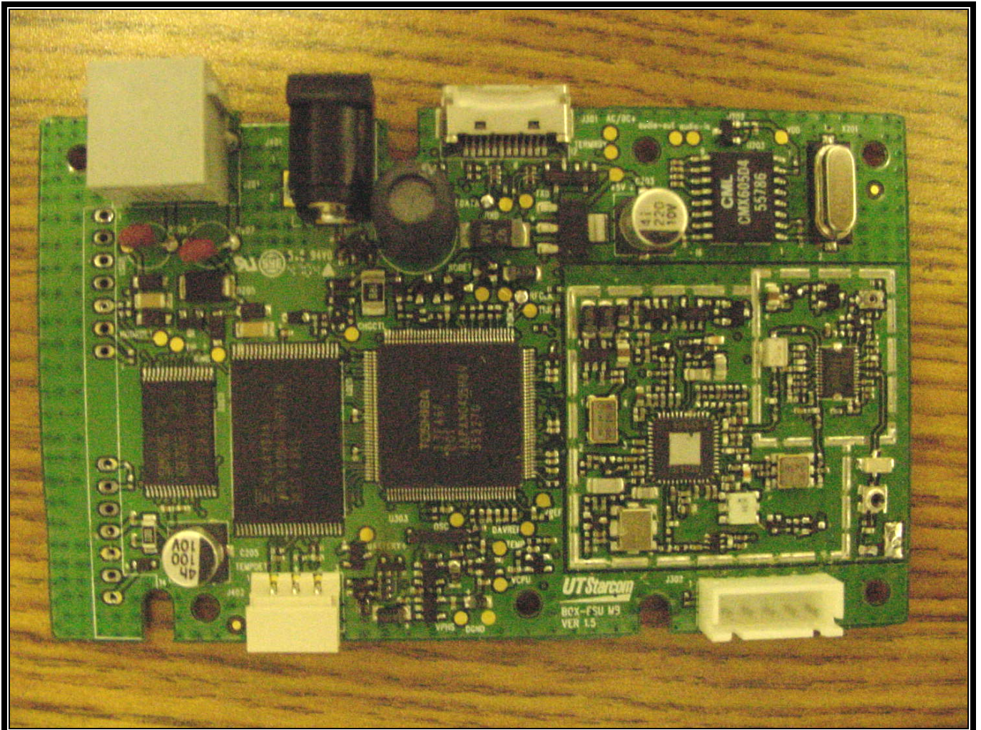
PHOTOGRAPH 20: TOP OF PCB WITH SHIELDS REMOVED
