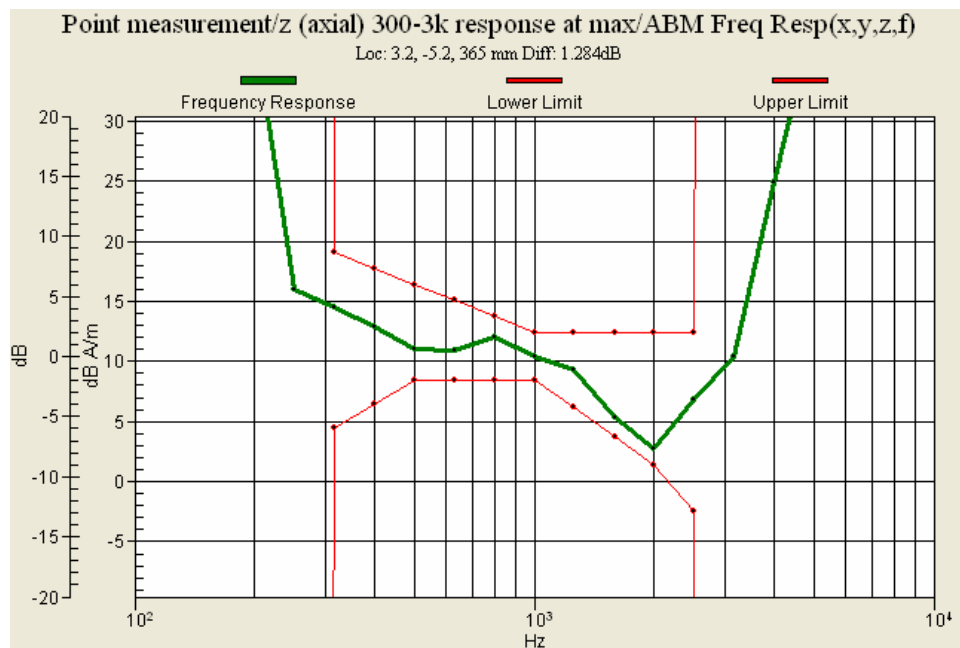
Figure 10.12 : AWS CDMA (CH 25) Frequency Response (T-coil Center)
