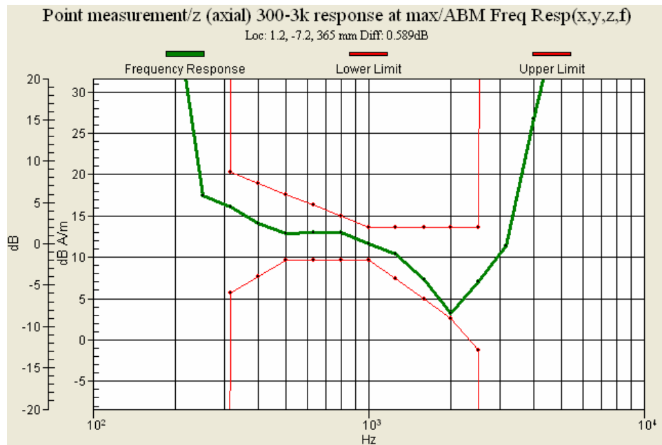
Figure 10.11 : AWS CDMA (CH 875) Frequency Response
