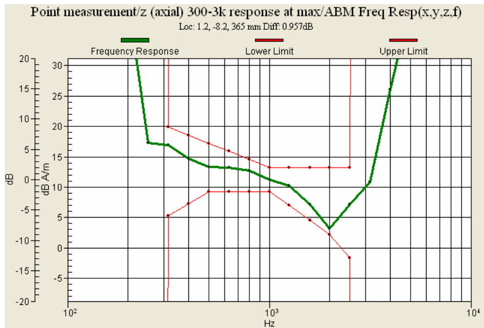
Figure 10.10 : AWS CDMA (CH 425) Frequency Response
