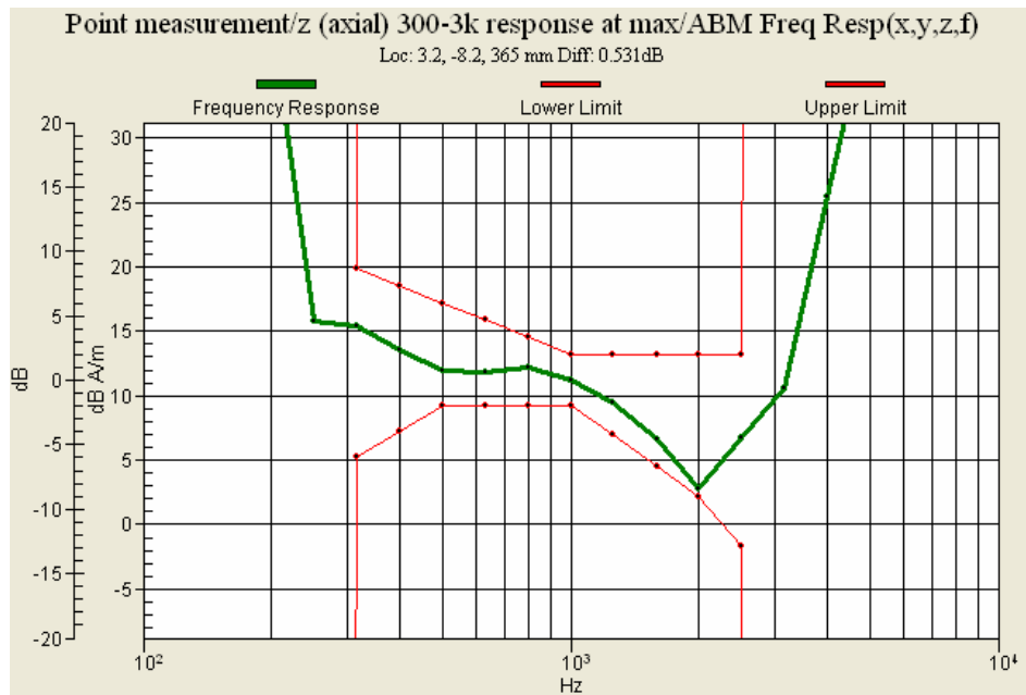
Figure 10.9 : AWS CDMA (CH 25) Frequency Response
