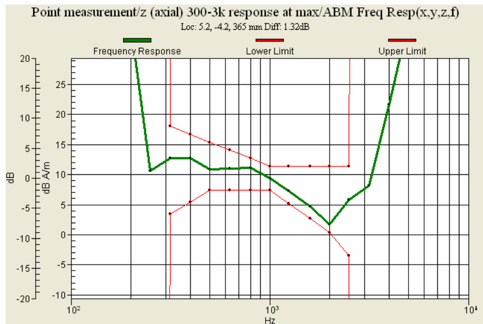
Figure 10.4 : CDMA (CH 1013) Frequency Response (T-coil Center)
