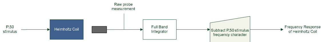
Figure C ITU-T P.50 Signal Processing Block Diagram (Frequency Response Validation)
