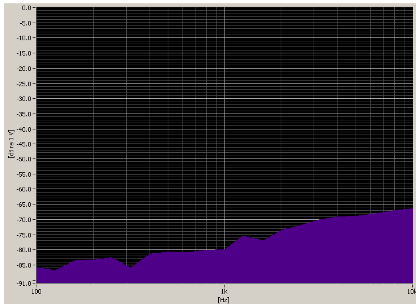
Figure E ABM2 Spectrum Plot
