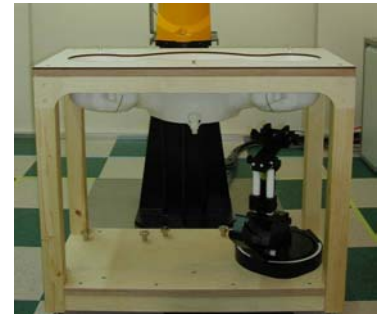
Figure 11. SAM Phantom
