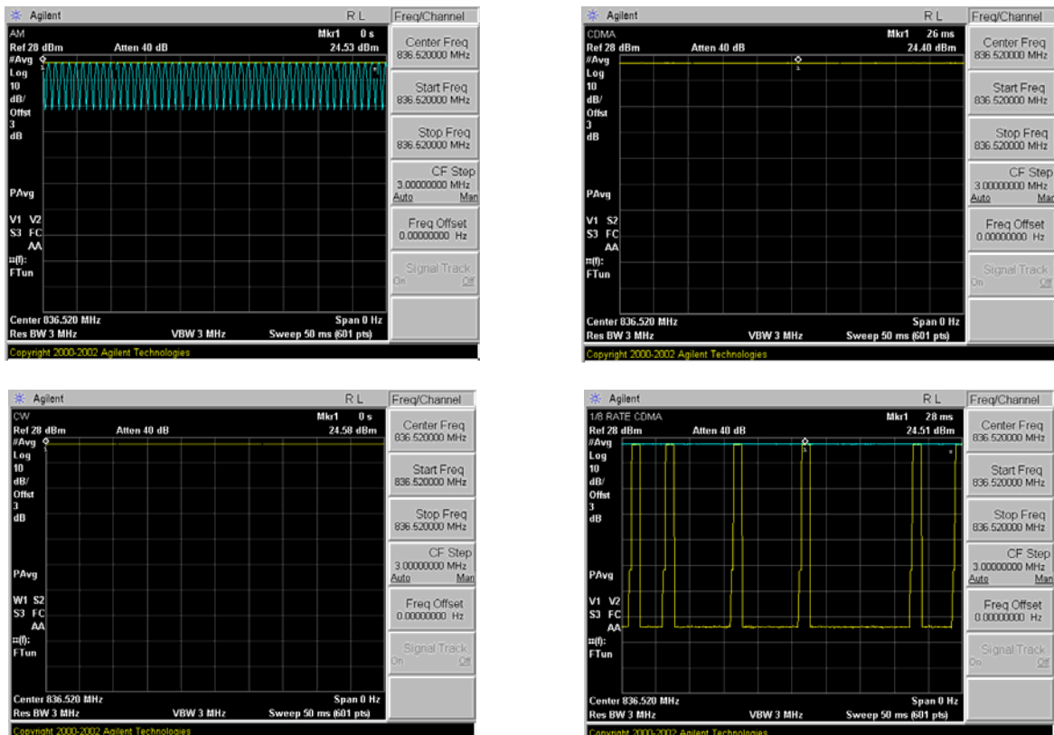
Figure 26 Zero-Span Plots
