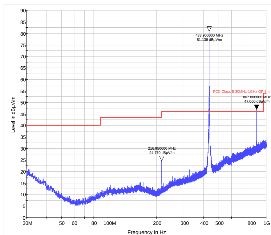
Radiated spurious emissions 30 MHz to 1 GHz
