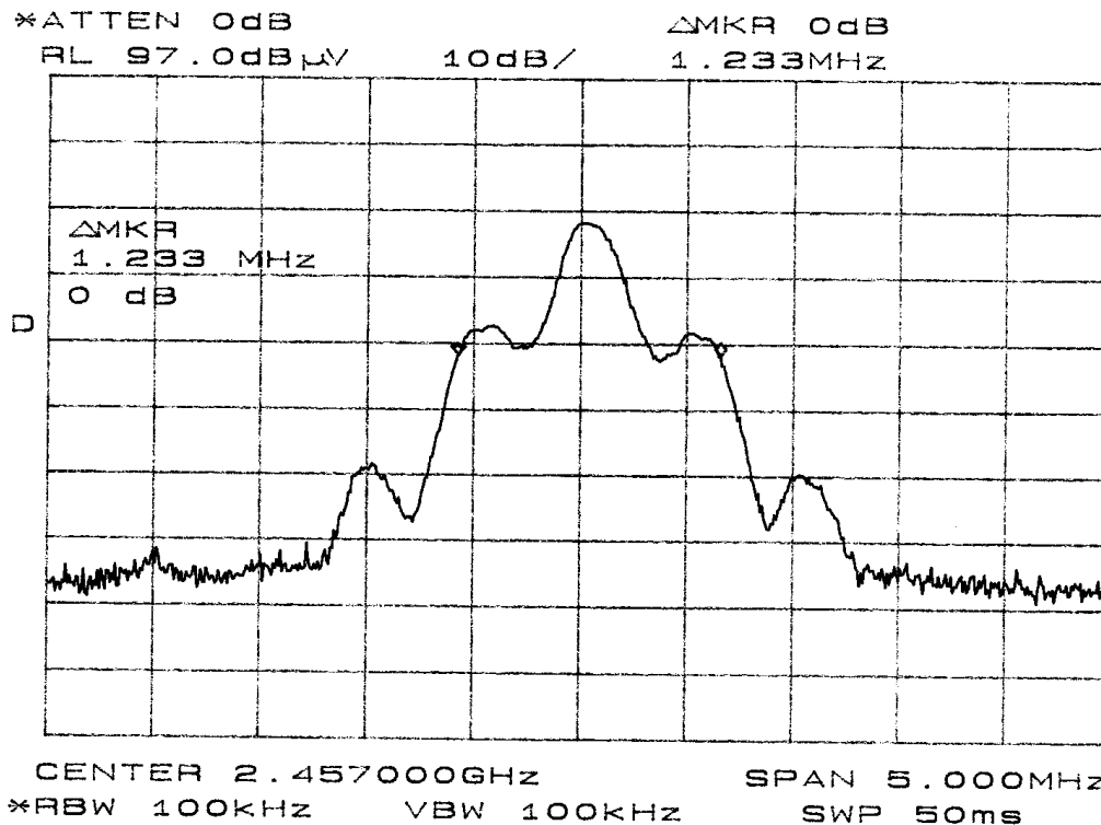
Figure seven Occupied Bandwidth and Operation in Frequency Band
