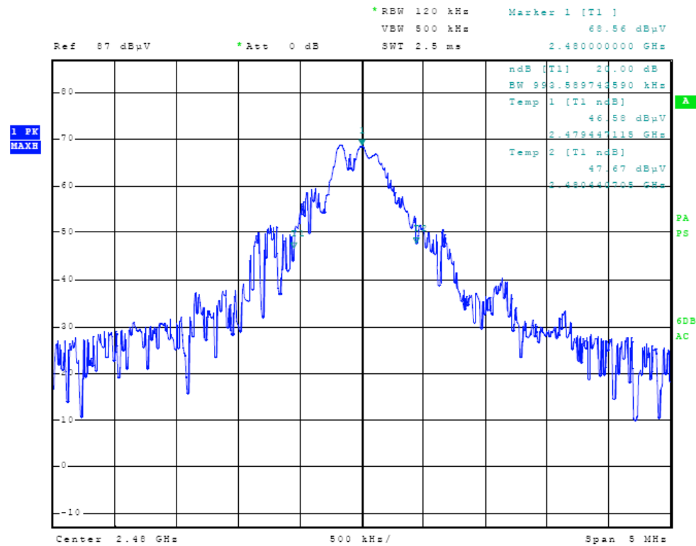
Figure Eleven Transmitter Occupied Bandwidth (High channel)
