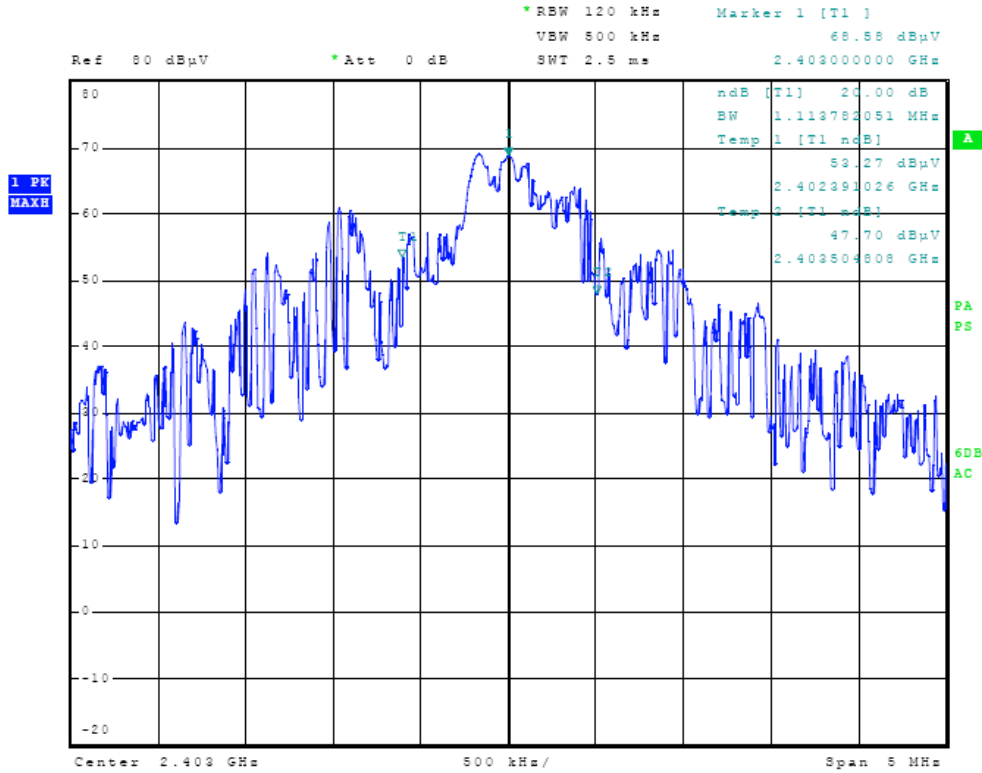
Figure Ten Transmitter Occupied Bandwidth (Low channel)
