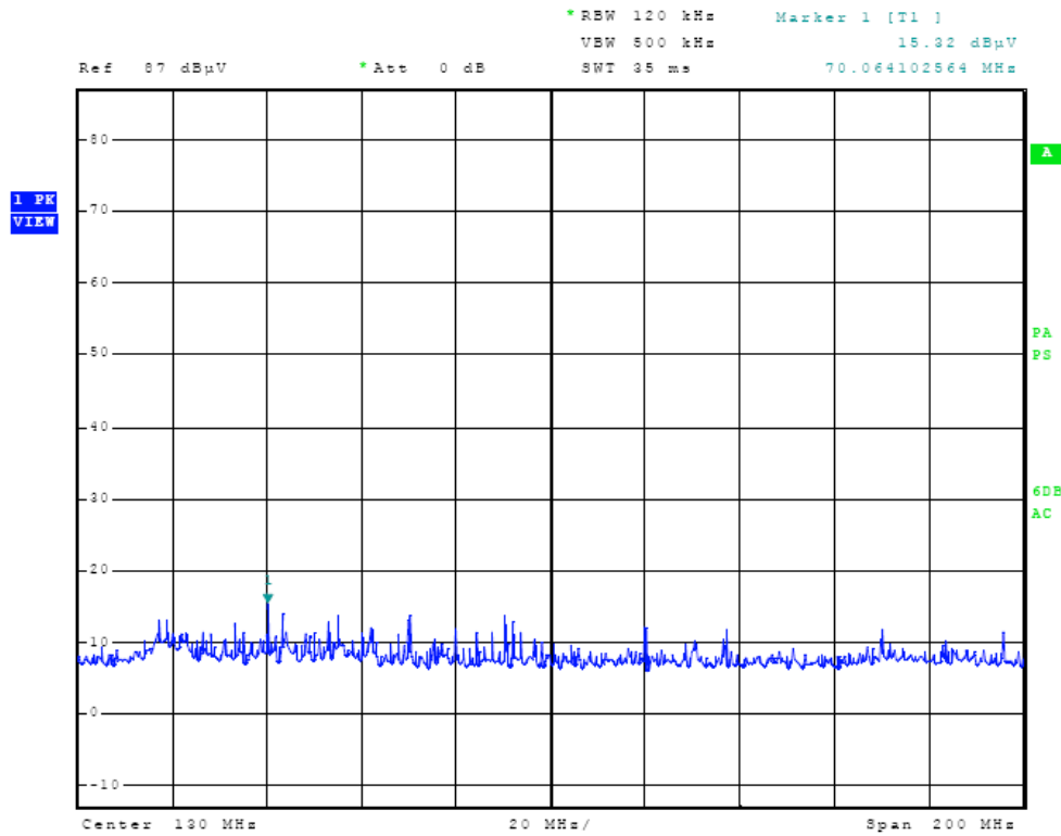
Figure One Radiated Emissions in screen room
