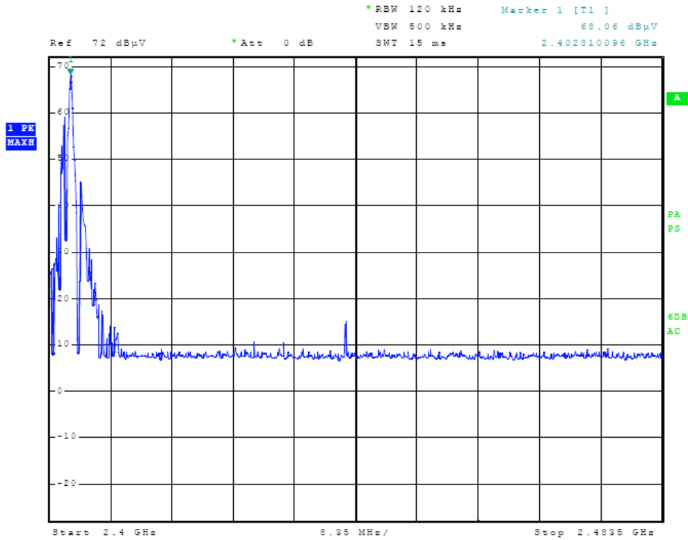
Figure Eight Transmitter Radiated Emissions Plot (Low channel)
