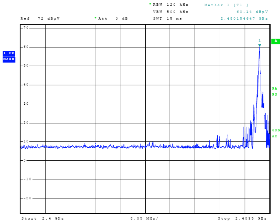
Figure Nine Transmitter Radiated Emissions Plot (High channel)
