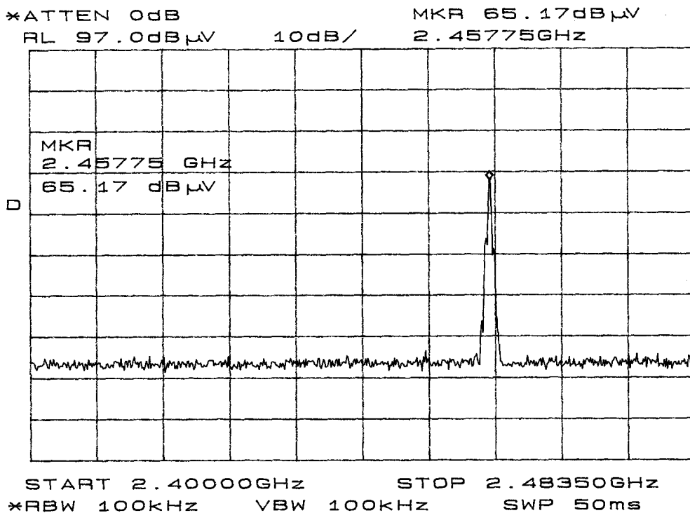
Figure eight Operation in Frequency Band
