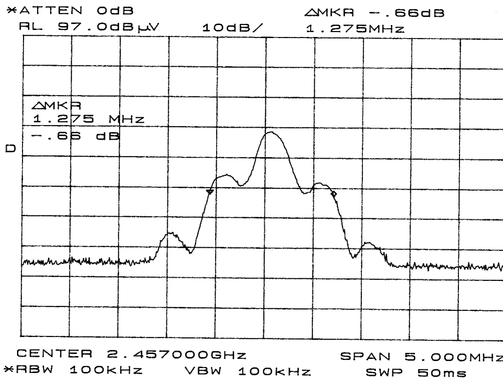
Figure nine Occupied Bandwidth
