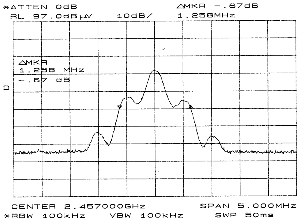
Figure nine Occupied Bandwidth
