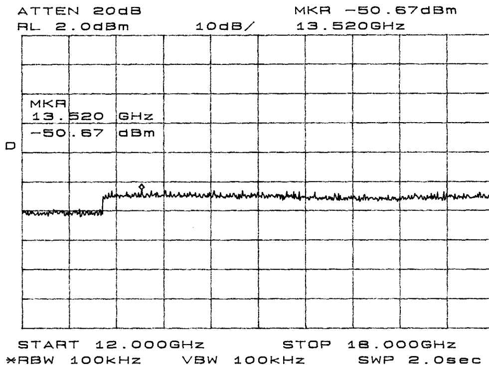
Figure Ten output measured at temporary antenna terminal
