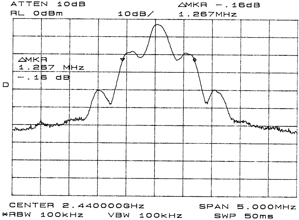
Figure Thirteen Occupied Bandwidth
