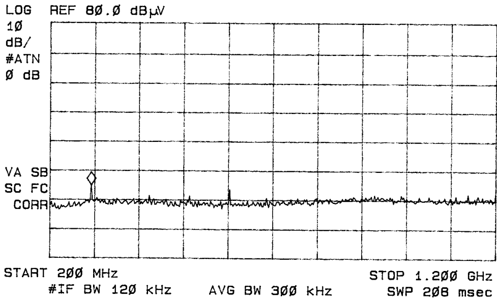
Figure Two Radiated Emissions in screen room
