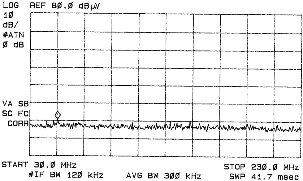
Figure One Radiated Emissions in screen room
