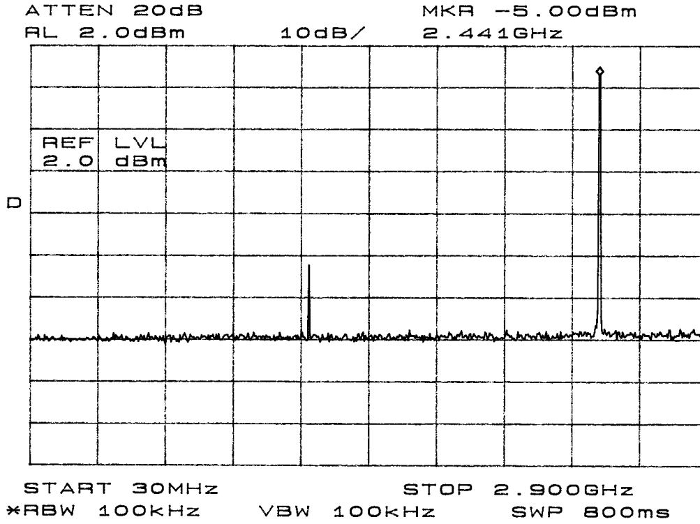
Figure Seven output measured at temporary antenna terminal
