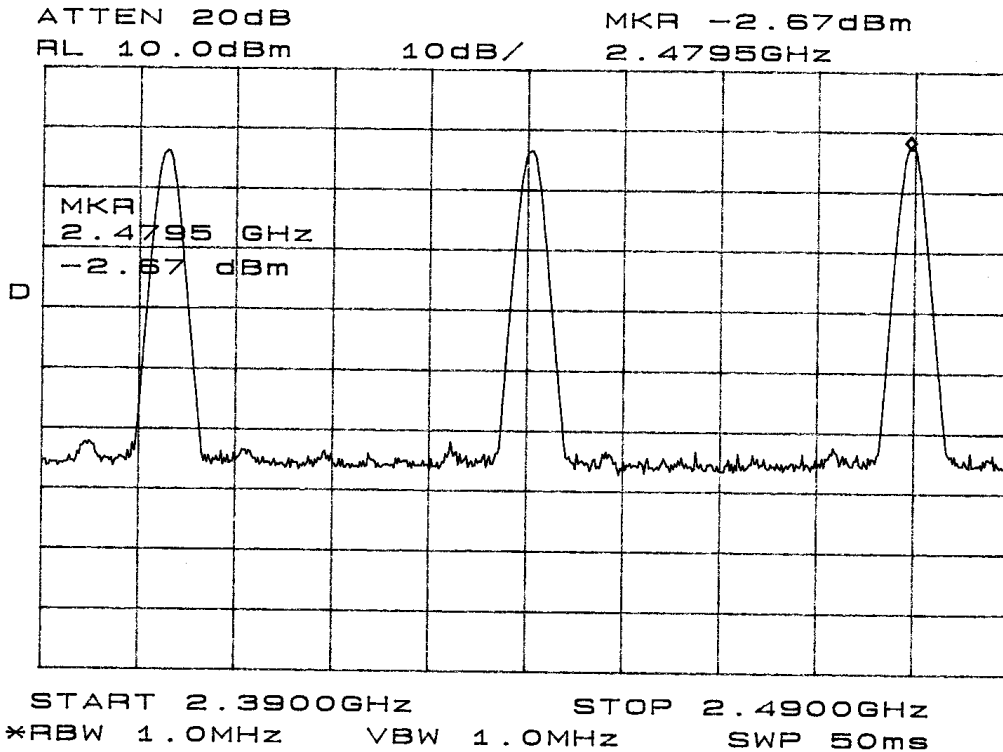
Figure Eleven output measured at temporary antenna terminal
