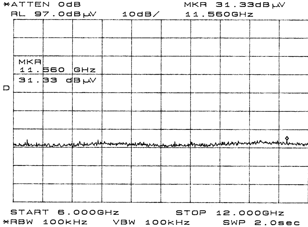
Figure Five Radiated Emissions in screen room
