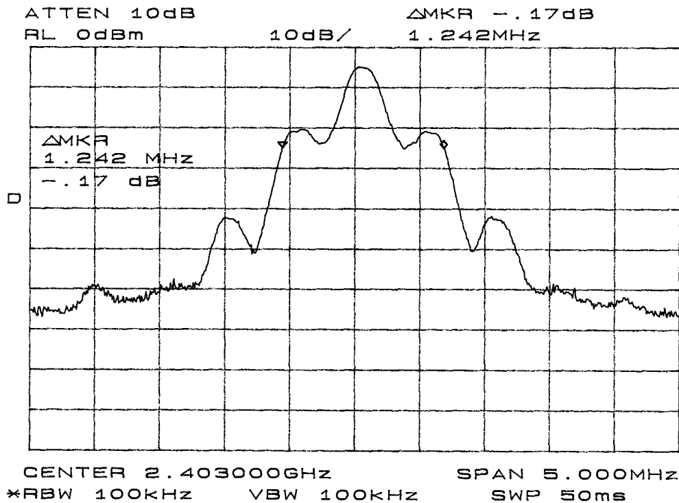
Figure Twelve Occupied Bandwidth
