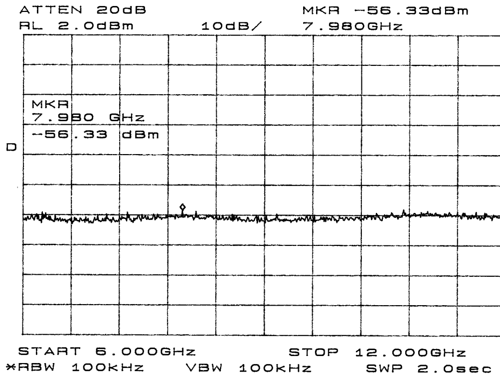
Figure Nine output measured at temporary antenna terminal
