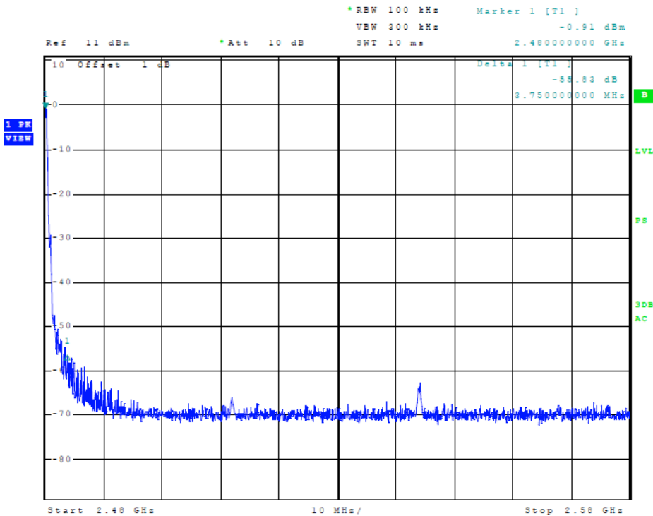
Figure 14 Plot of Transmitter Emissions (BLE High Band Edge)
