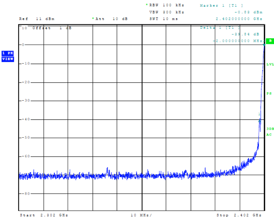
Figure 9 Plot of Transmitter Emissions (ANT 2Mb Low Band Edge)
