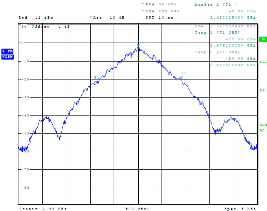
Figure 8 Plot of Transmitter Emissions (ANT 2Mb 99% Occupied Bandwidth)
