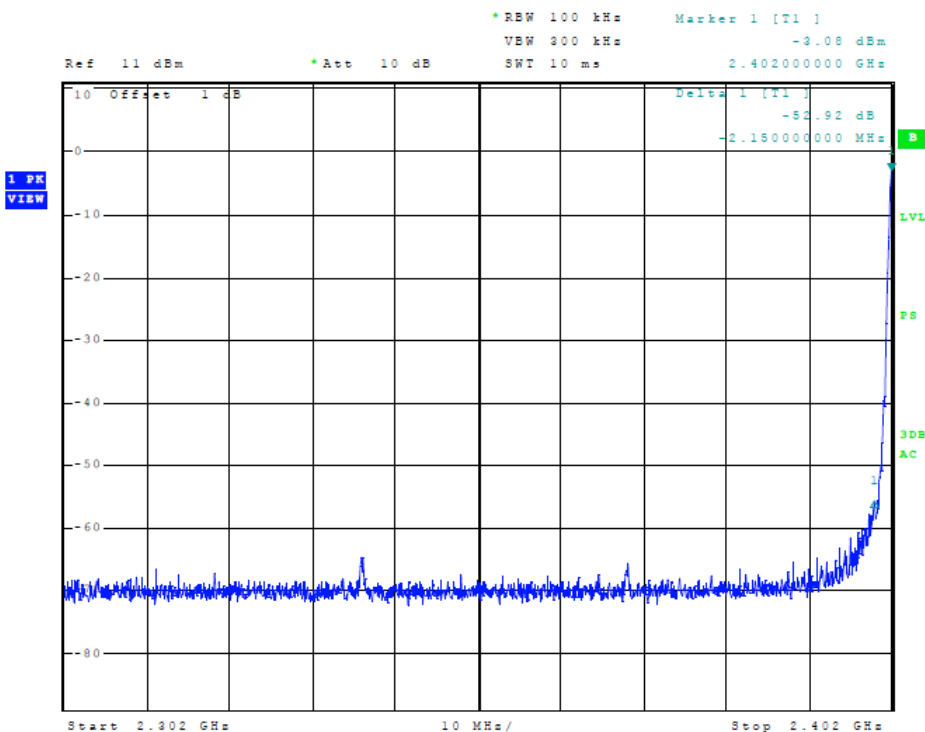
Figure 5 Plot of Transmitter Emissions (ANT 1Mb Low Band Edge)
