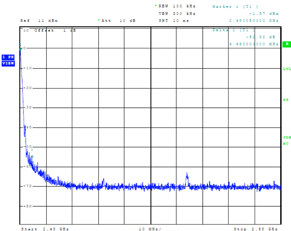
Figure 10 Plot of Transmitter Emissions (ANT 2Mb High Band Edge)
