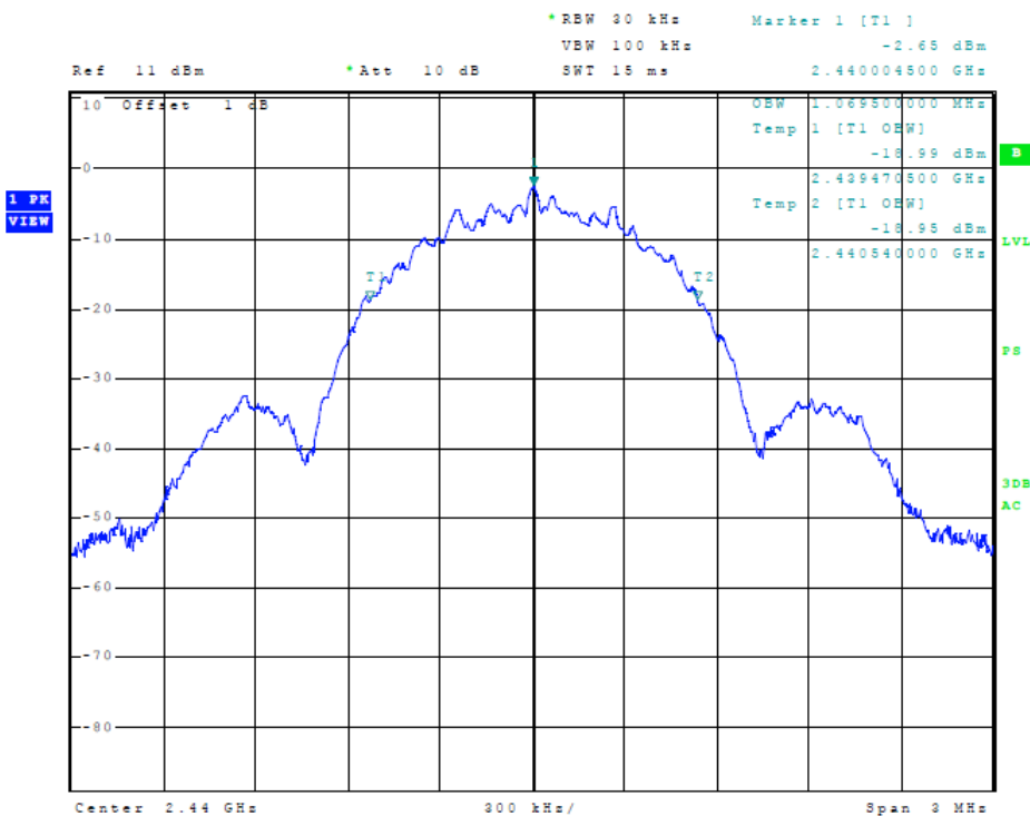
Figure 12 Plot of Transmitter Emissions (BLE 99% Occupied Bandwidth)
