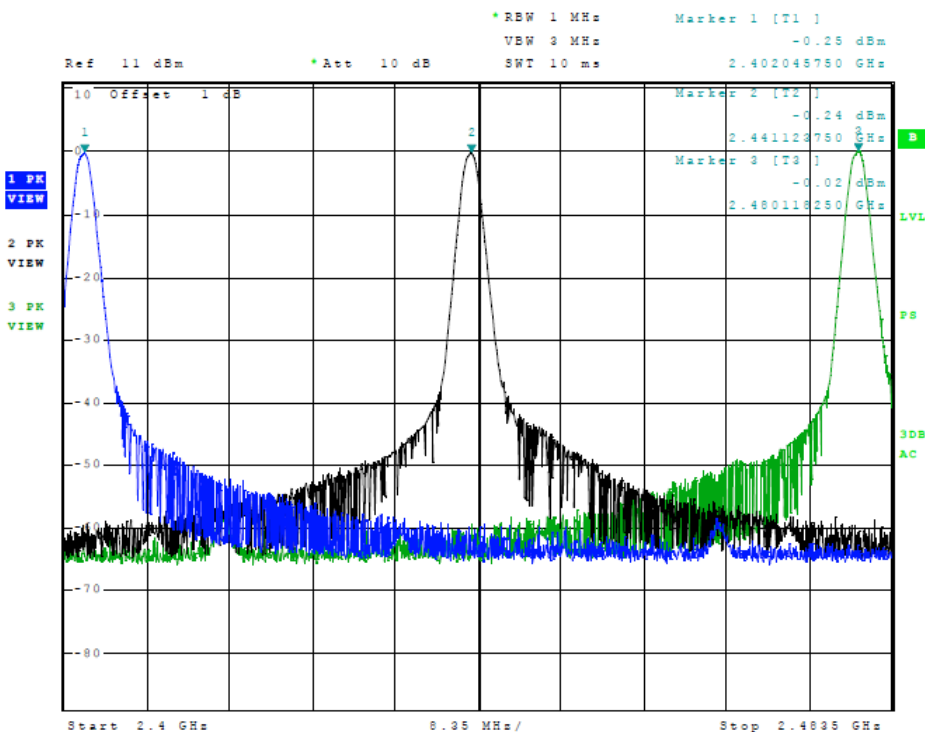
Figure 3 Plot of Transmitter Emissions (ANT 1Mb Operation in 2402-2480 MHz)
