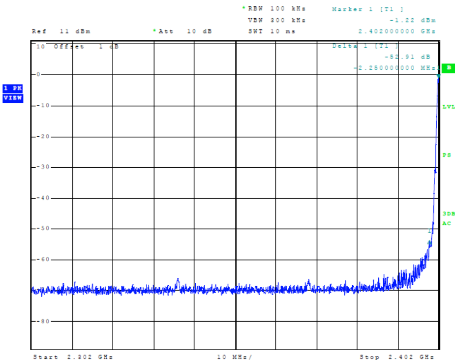
Figure 13 Plot of Transmitter Emissions (BLE Low Band Edge)
