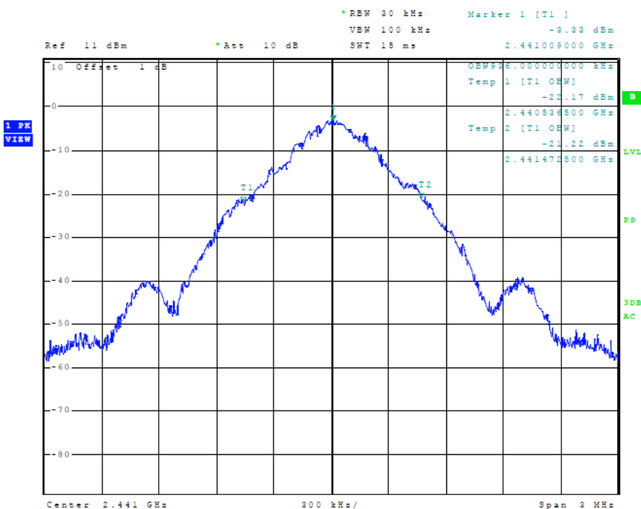
Figure 4 Plot of Transmitter Emissions (ANT 1Mb 99% Occupied Bandwidth)
