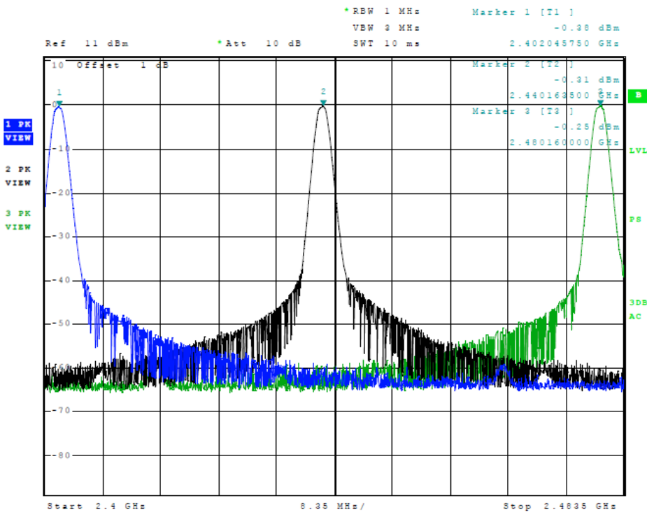
Figure 11 Plot of Transmitter Emissions (BLE Operation in 2402-2480 MHz)
