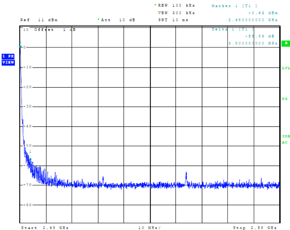
Figure 6 Plot of Transmitter Emissions (ANT 1Mb High Band Edge)
