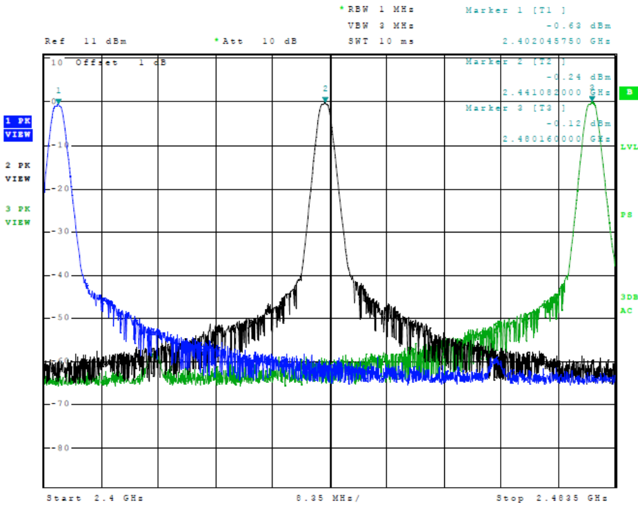
Figure 7 Plot of Transmitter Emissions (ANT 2Mb Operation in 2402-2480 MHz)
