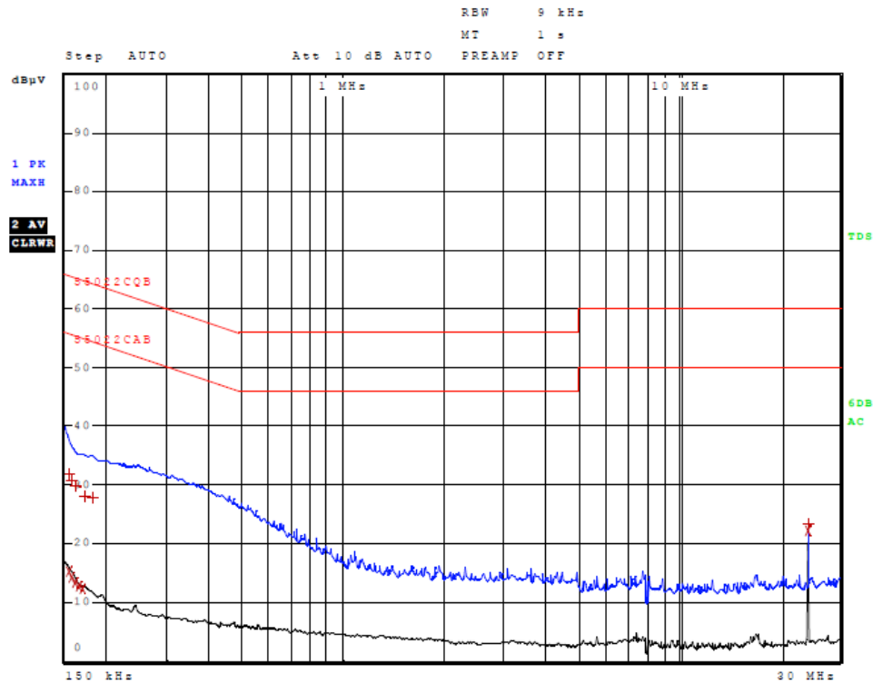
Figure 9 AC Line Conducted emissions of EUT line 1
