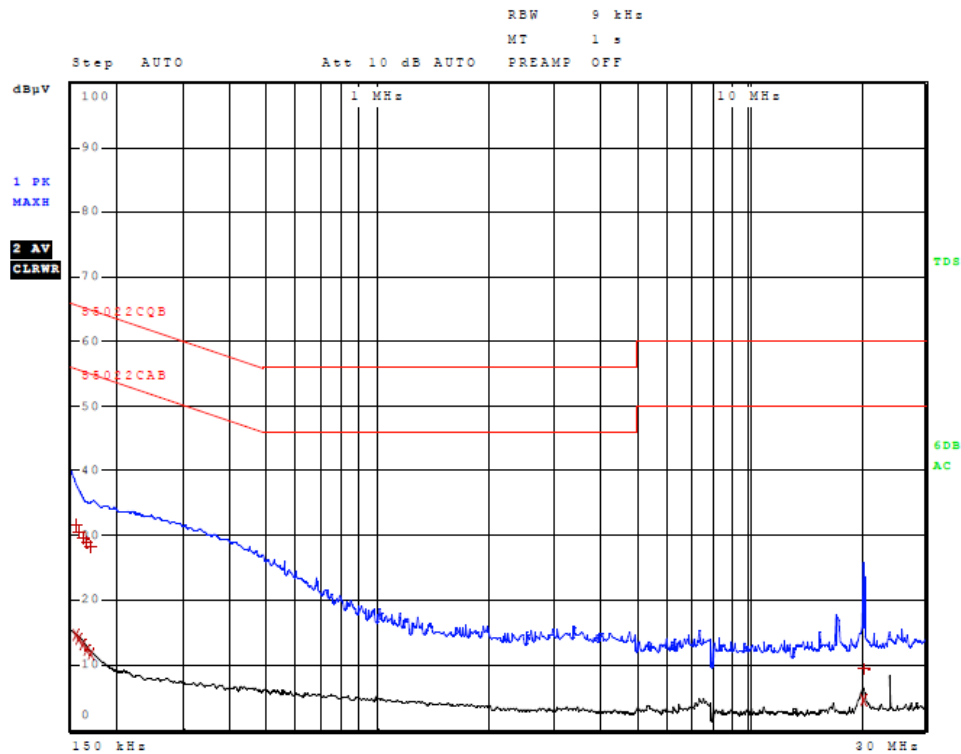
Figure 10 AC Line Conducted emissions of EUT line 2
