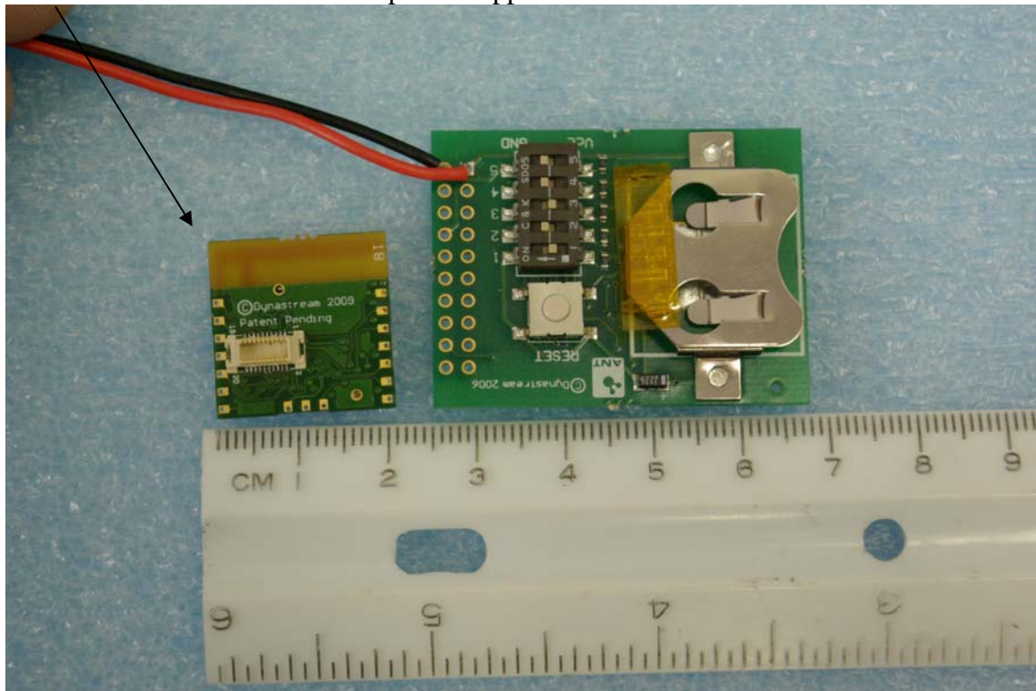
EUT Bottom side and test development support board
