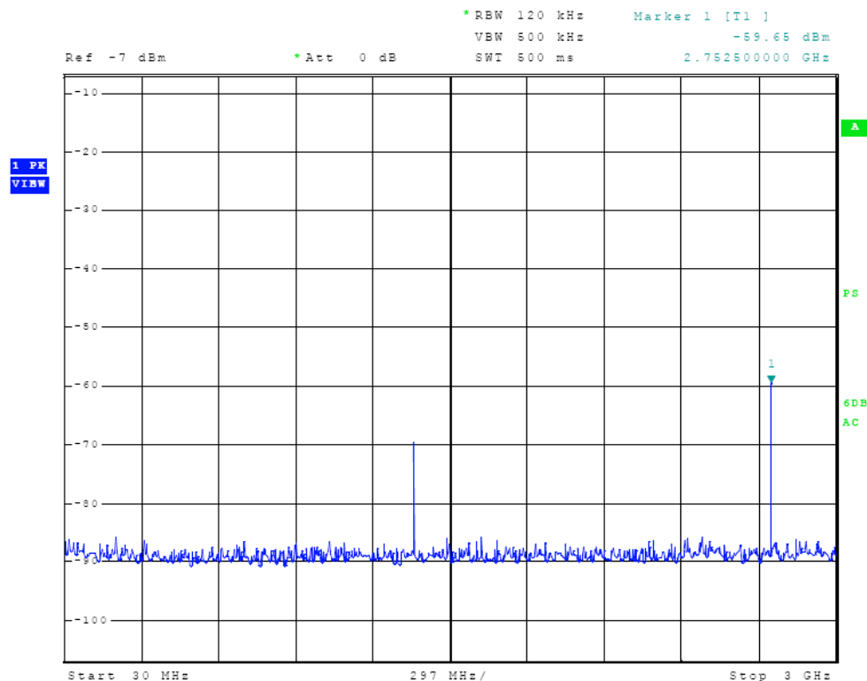
Figure Six Receiver Antenna Port Conducted Emissions
