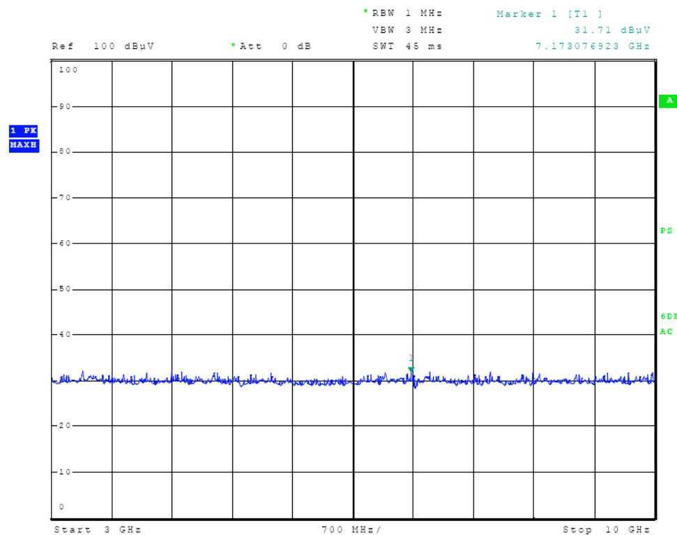
Figure Four Radiated Emissions Plot
