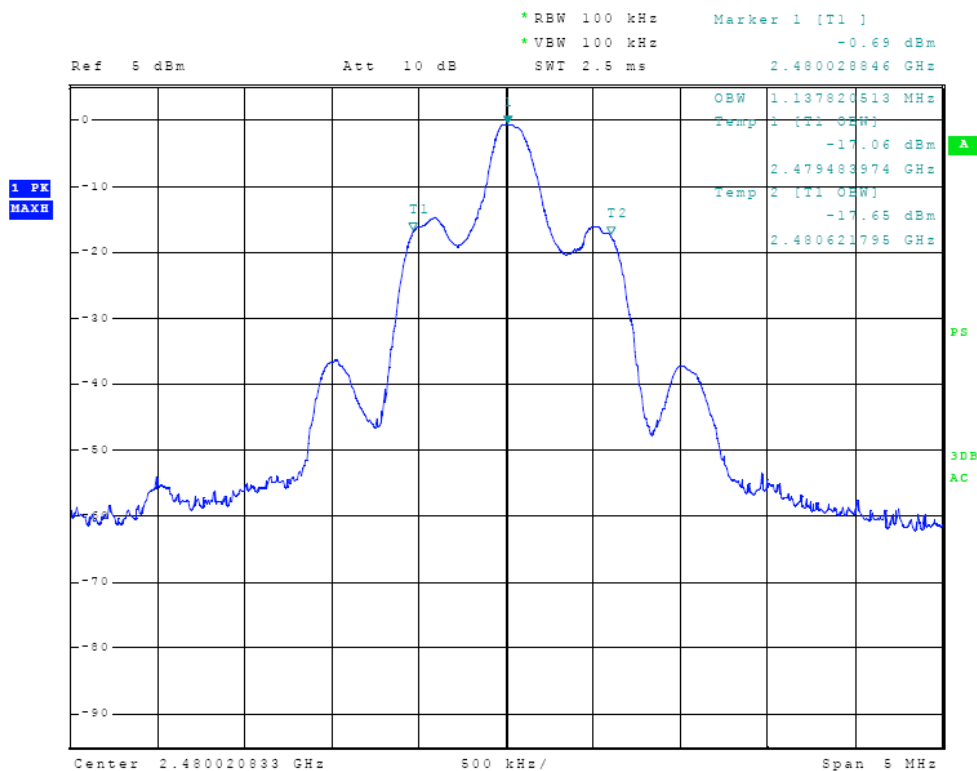
Figure Twelve Occupied Bandwidth
