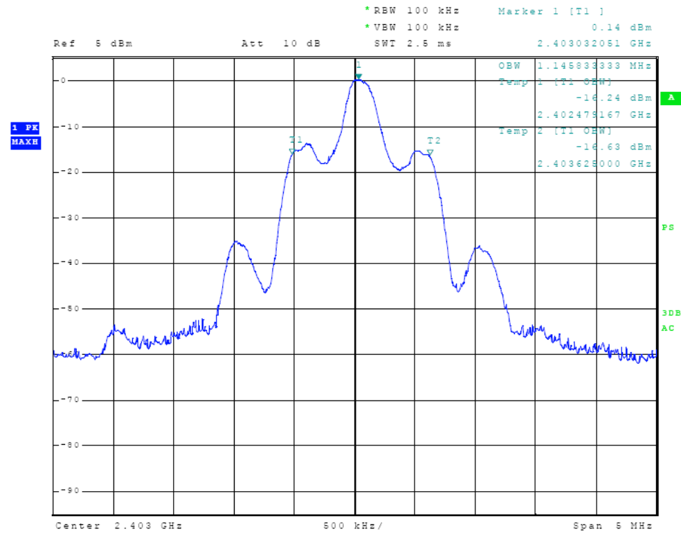
Figure Ten Occupied Bandwidth
