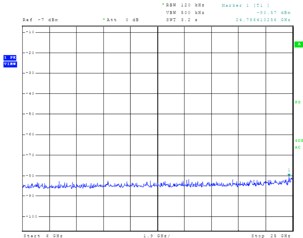
Figure Eight Receiver Antenna Port Conducted Emissions
