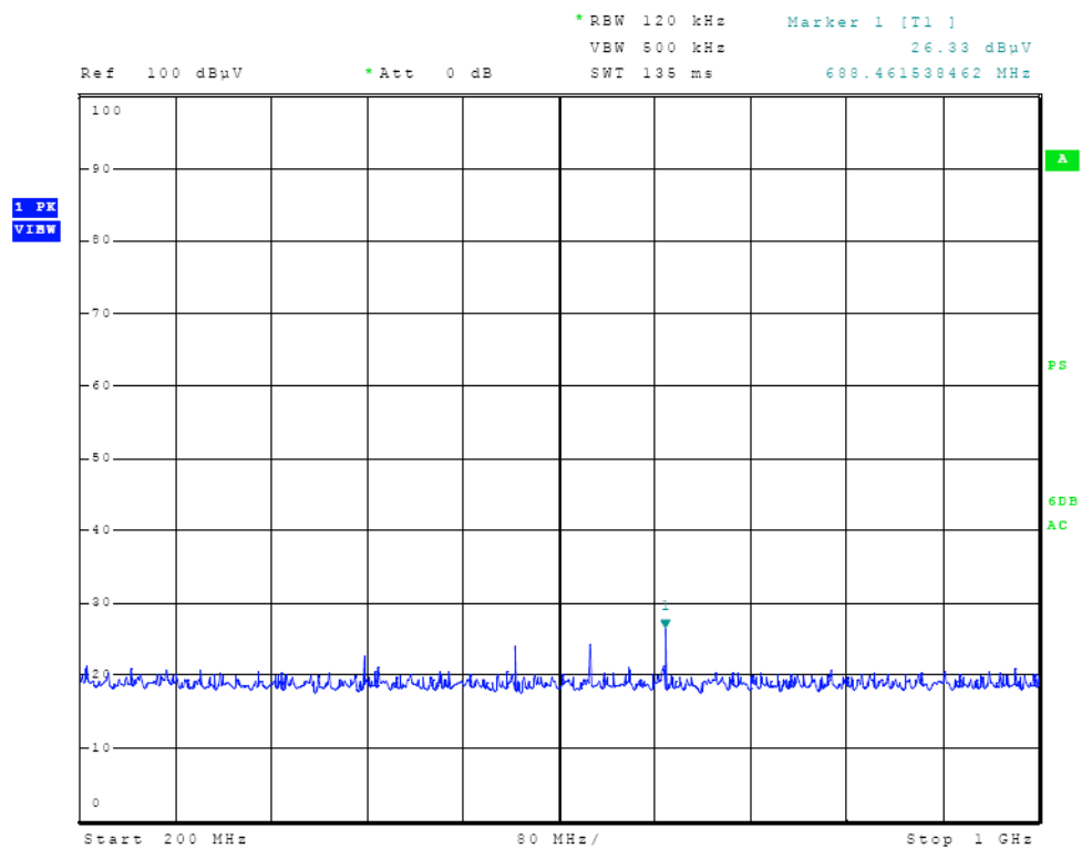
Figure Two Radiated Emissions Plot
