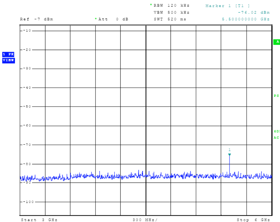
Figure Seven Receiver Antenna Port Conducted Emissions
