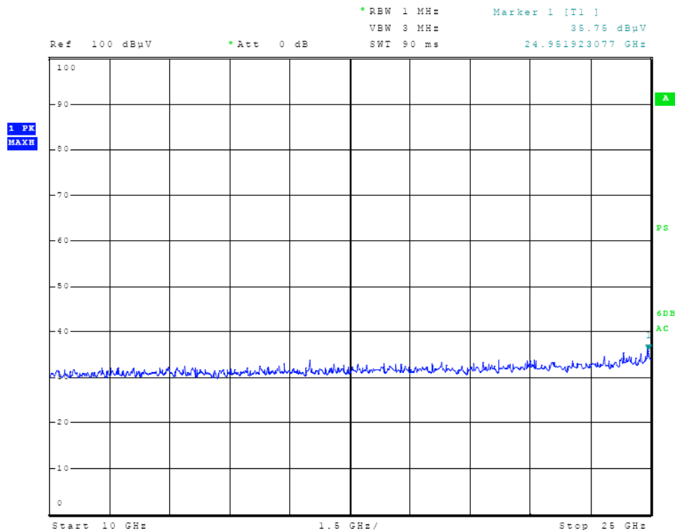
Figure Five Radiated Emissions Plot
