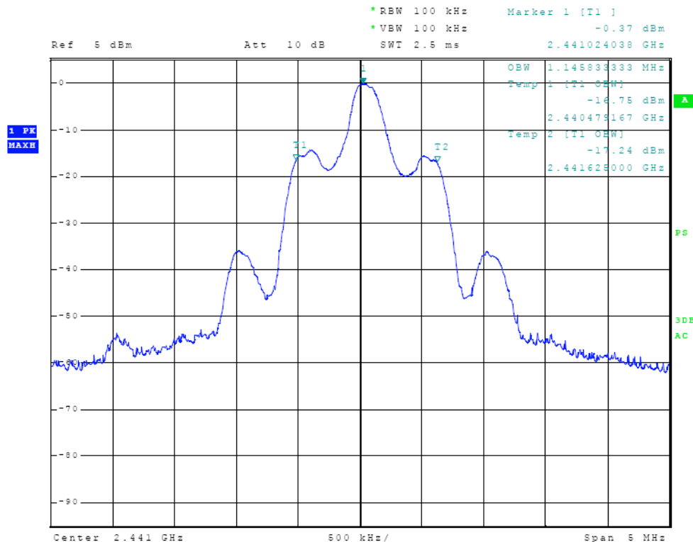
Figure Eleven Occupied Bandwidth
