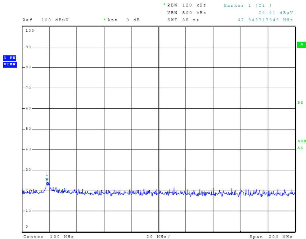
Figure One Radiated Emissions Plot
