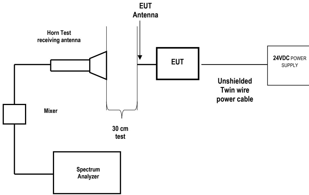
FIGURE 3-1: CONFIGURATION OF TESTED SYSTEM
