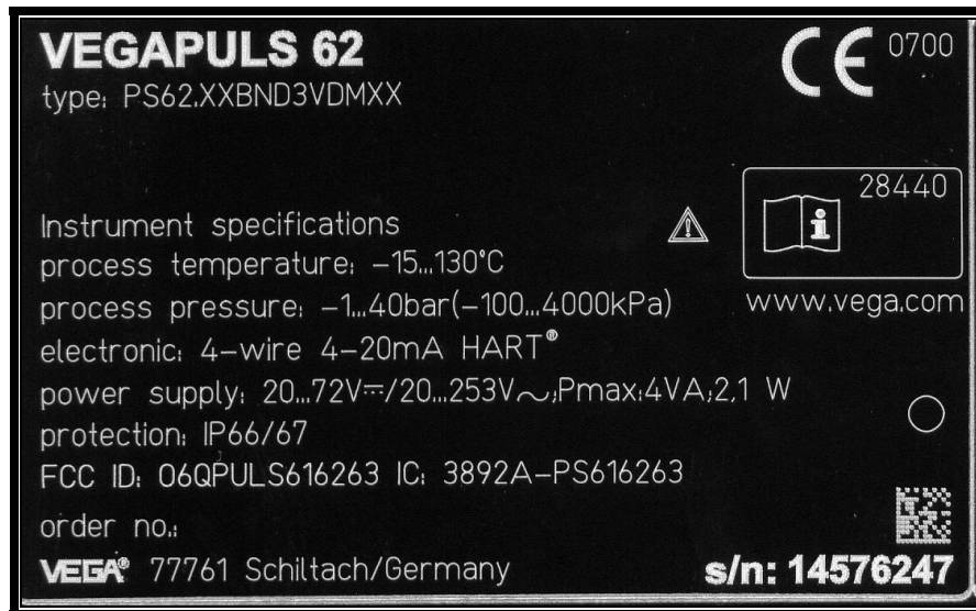
Photograph 2: FCC ID/IC ID Label Sample for Model VEGAPULS 62
