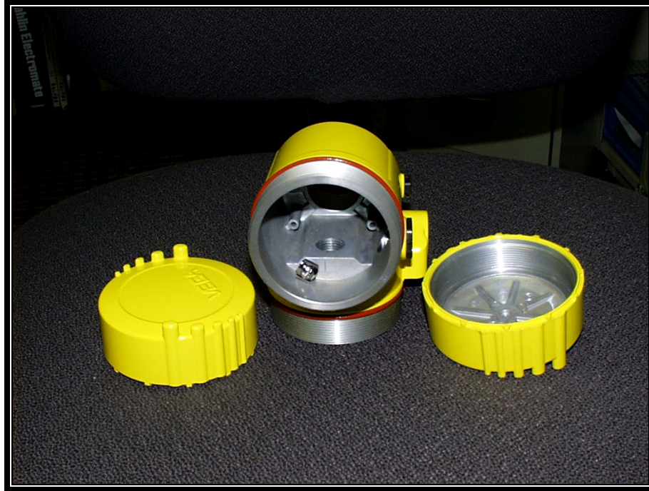
Photograph 23: EUT Double Aluminum Housing Fitting Front View
