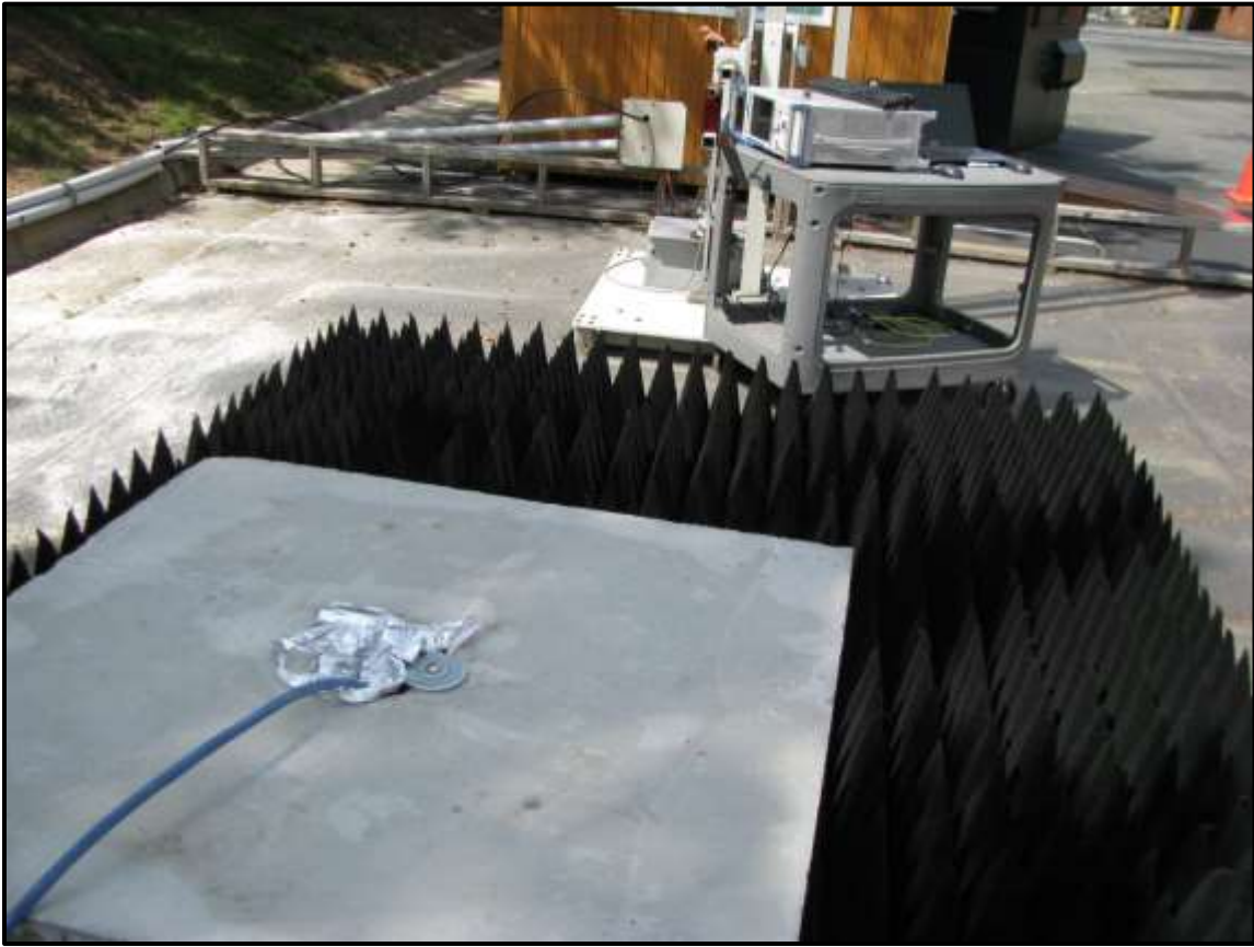
Photograph 23: Radiated Emissions – TC #2 Swivel; Concrete Container, Front View
