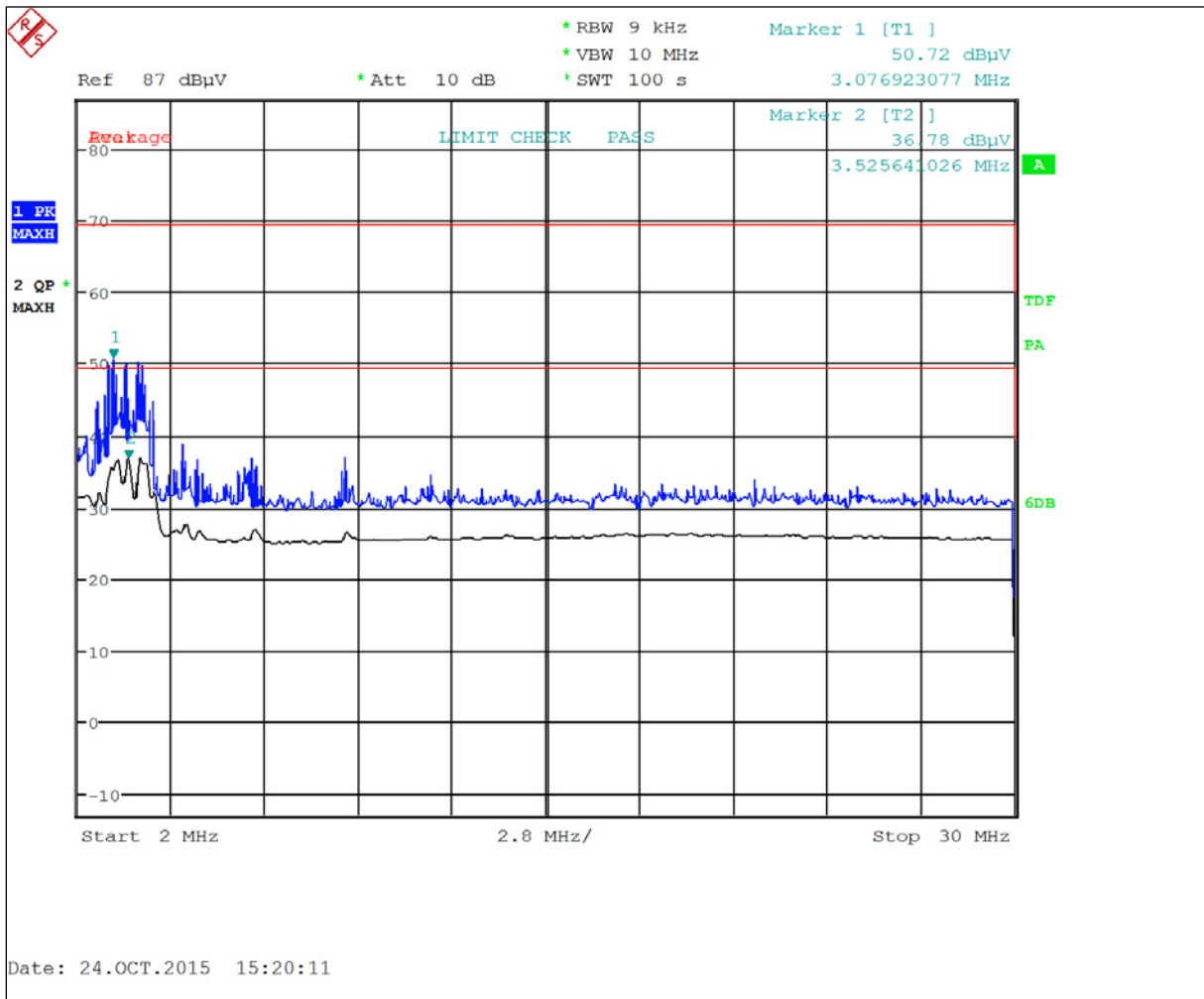
Plot 6-6: Radiated Emissions Transmit – 2 MHz – 30 MHz Horizontal Peak/Average
