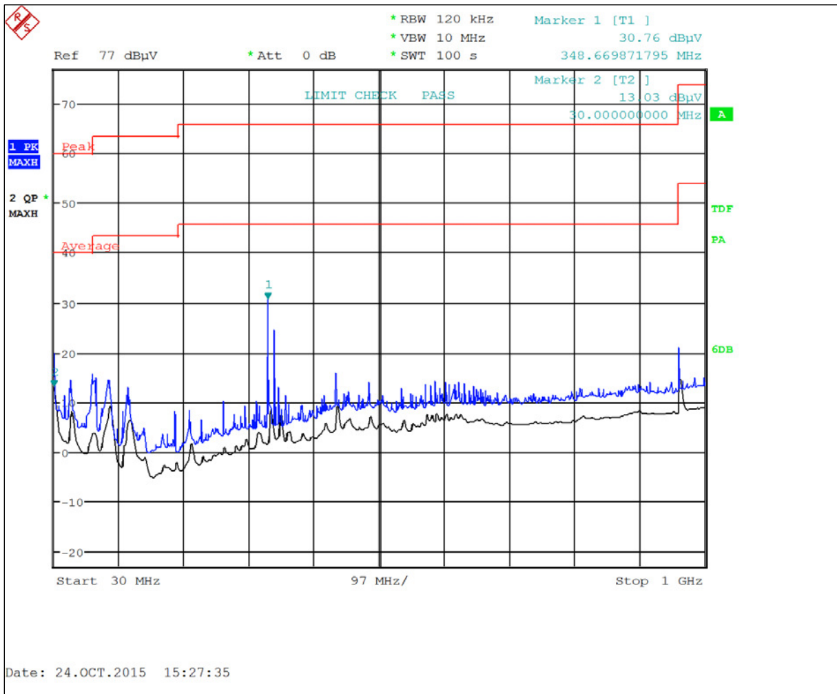
Plot 6-8: Radiated Emissions Transmit – 30 MHz – 1 GHz Horizontal Peak/Average
