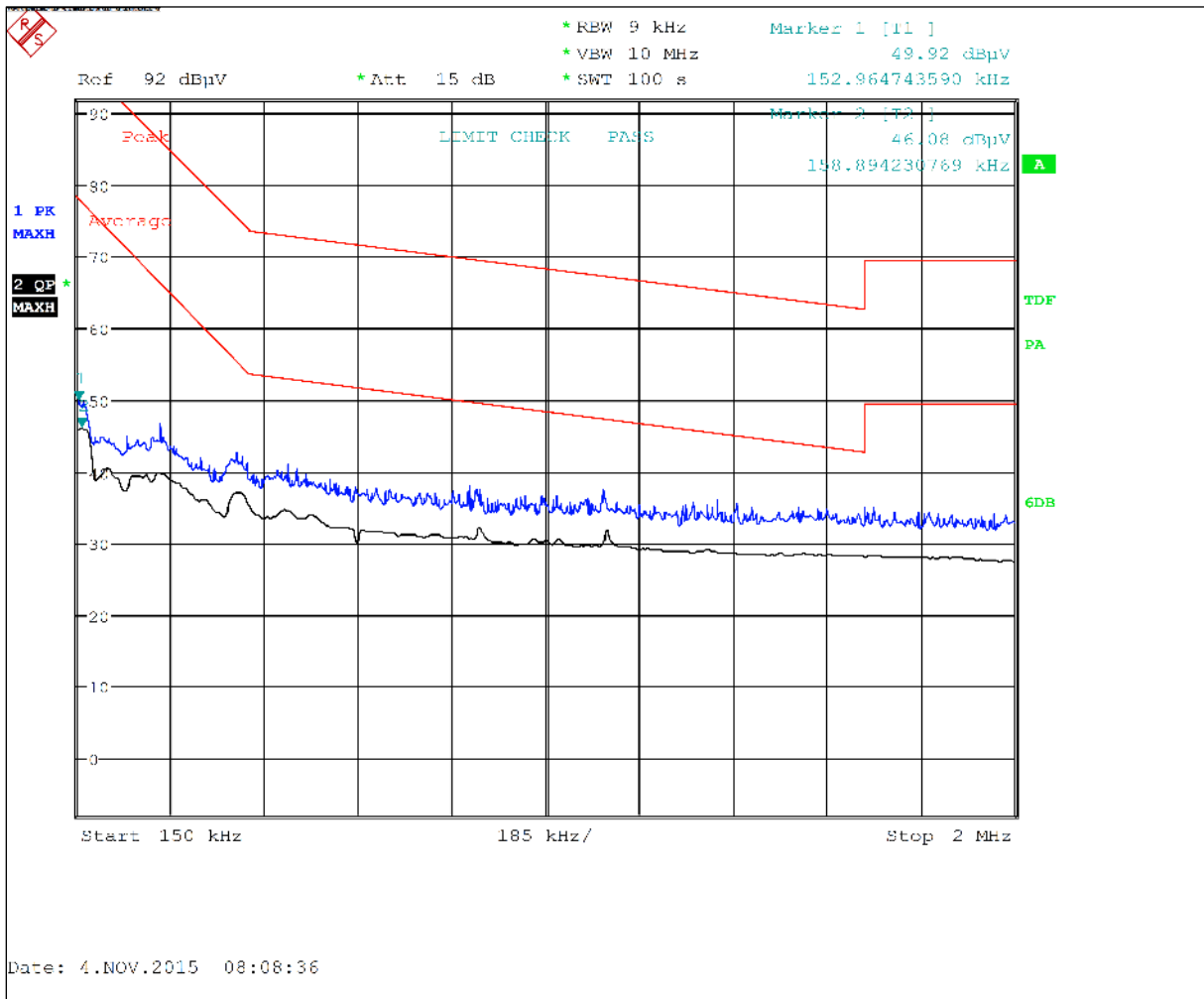
Plot 6-24: Radiated Emissions Transmit – 150 kHz – 2 MHz Vertical Peak/Average
