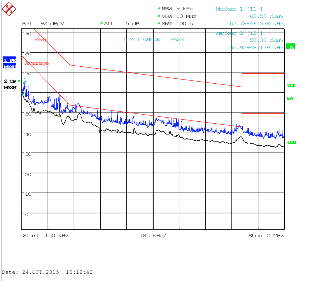
Plot 6-5: Radiated Emissions Transmit – 150 kHz – 2 MHz Vertical Peak/Average
