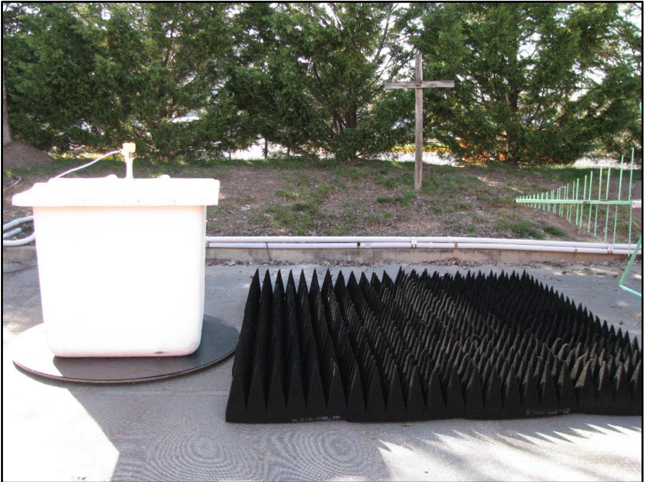
Photograph 66: Radiated Emissions – TC #9; Fiberglass Container, Rear View
