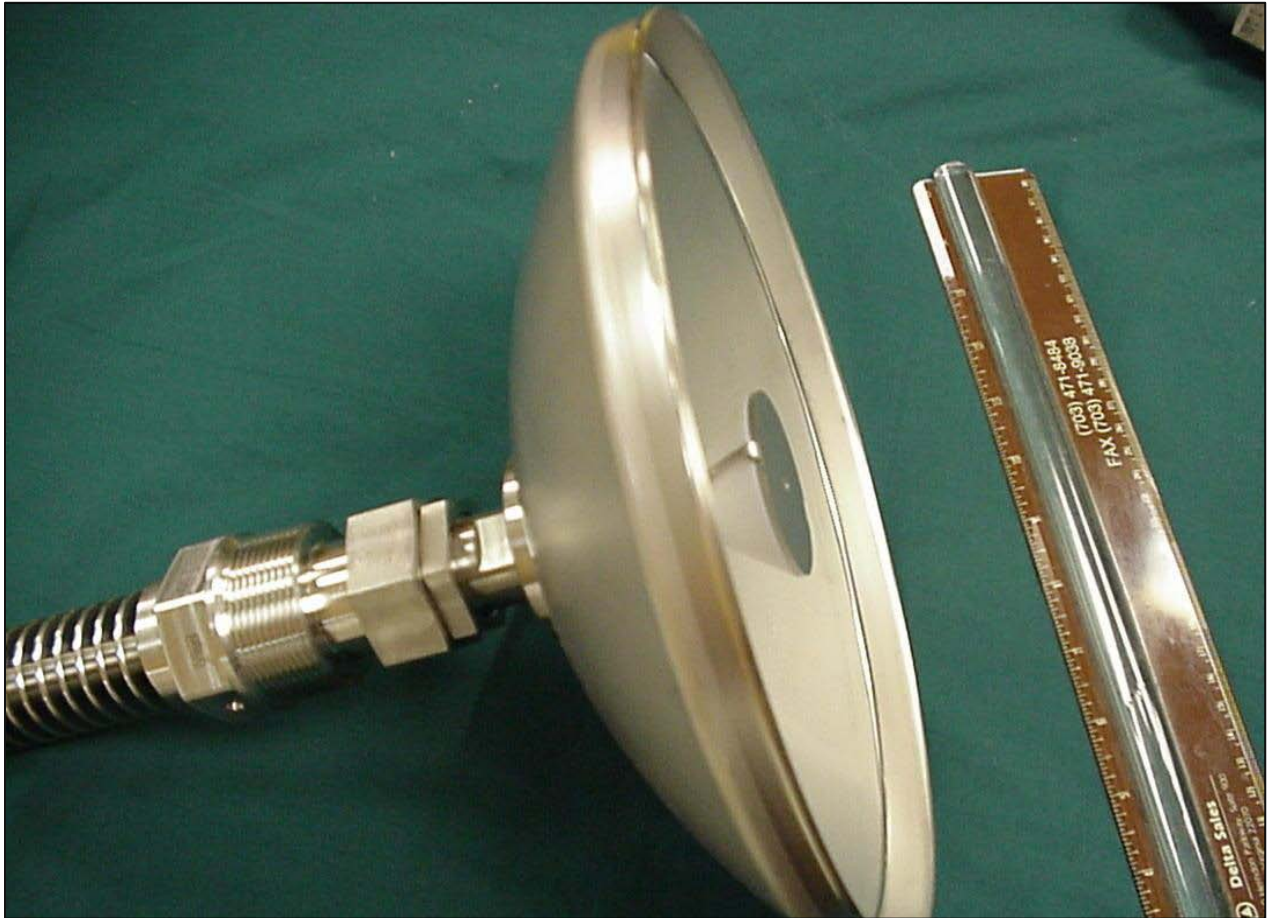
Photograph 1: 245-mm Parabolic Horn Antenna
