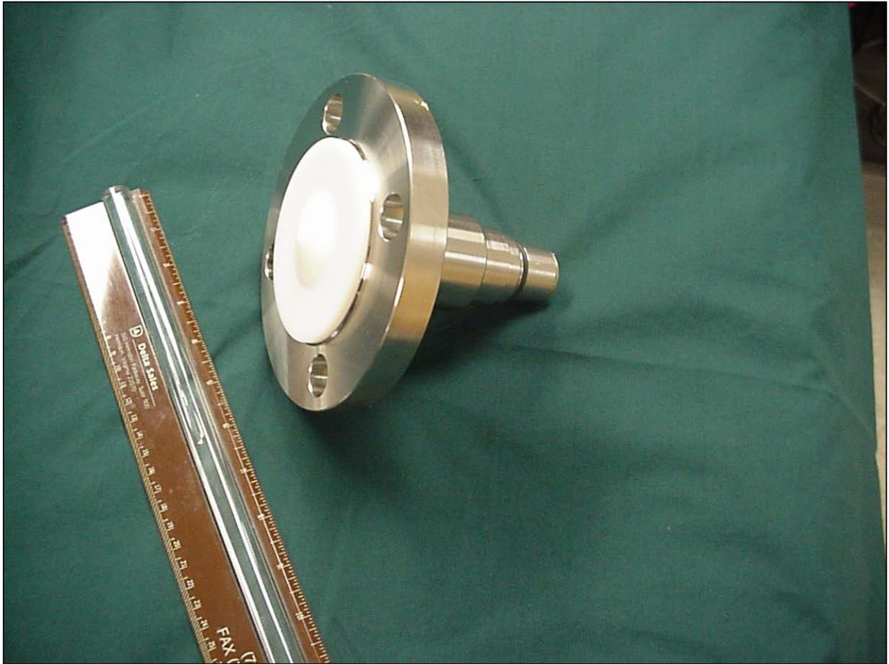
Photograph 8: 48-mm Metal Antenna
