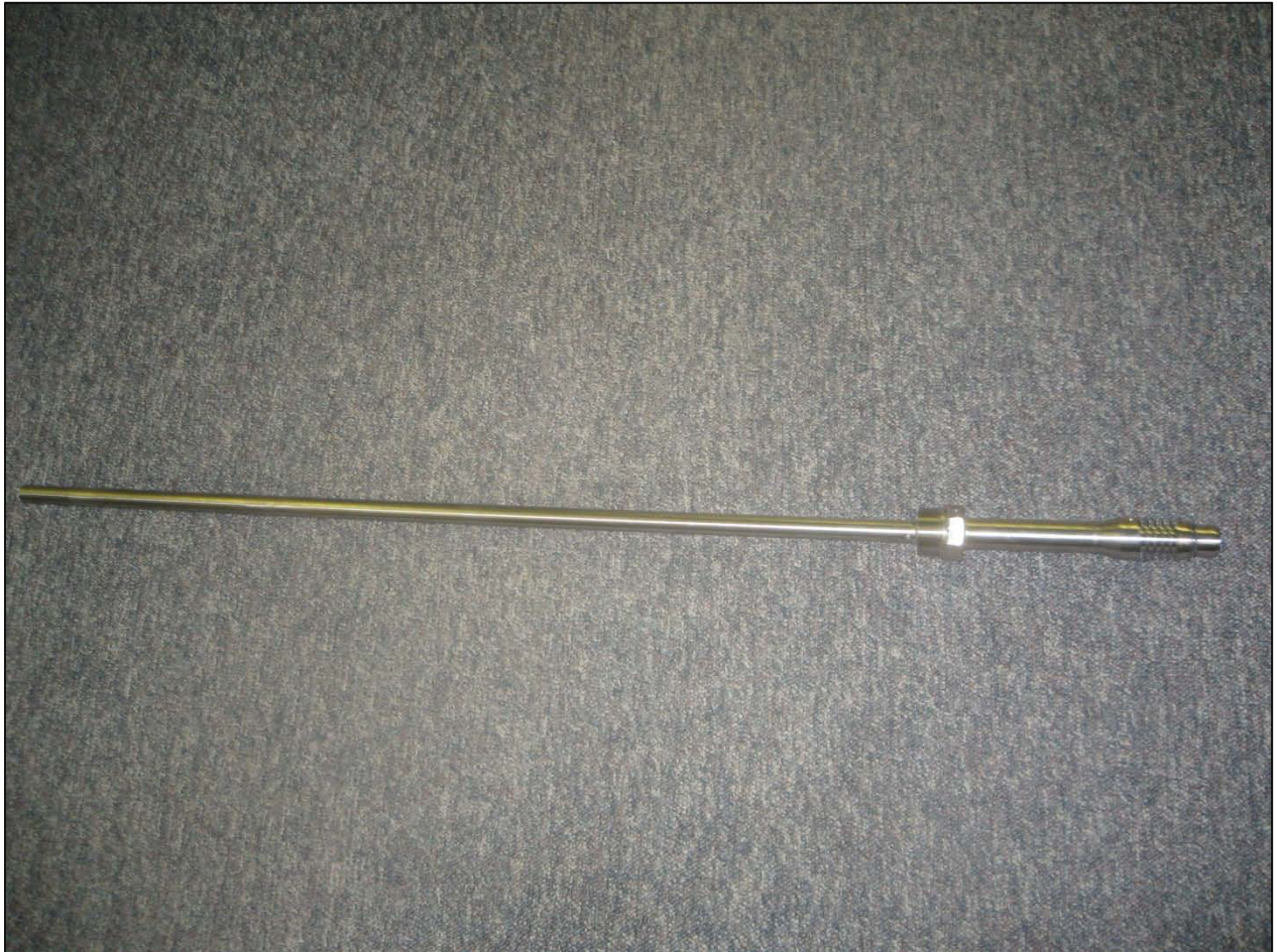
Photograph 10: 1/2" Standpipe Antenna
