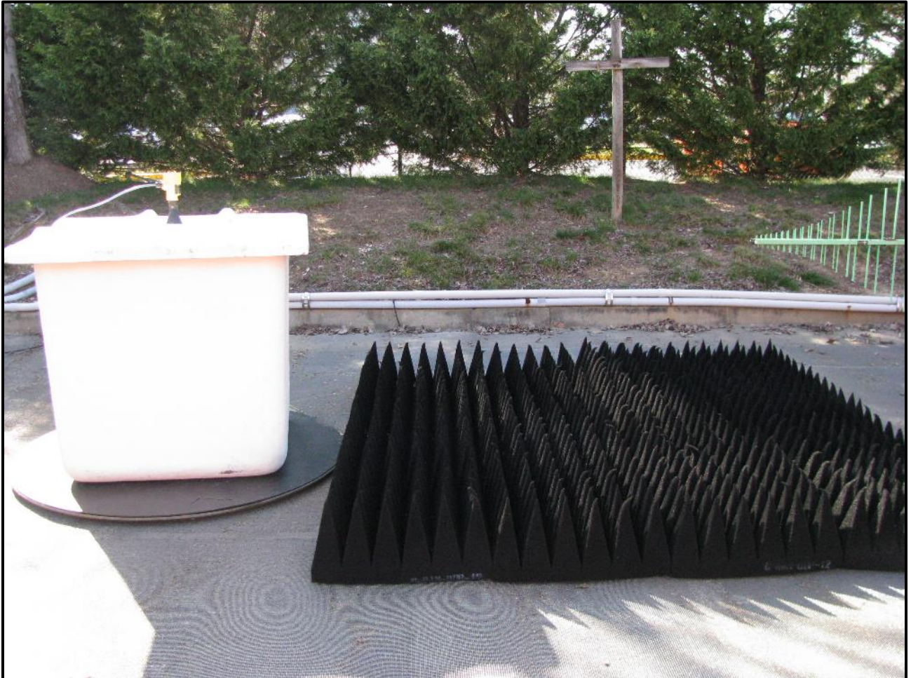
Photograph 50: Radiated Emissions – TC #1; Fiberglass Container, Rear View
