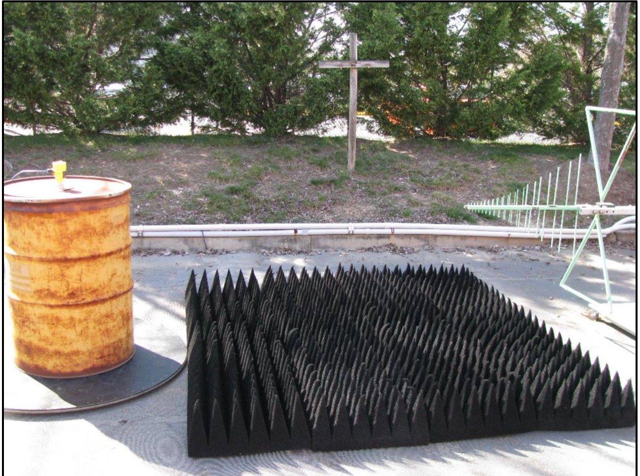
Photograph 20: Radiated Emissions – TC #4; Steel Container, Rear View
