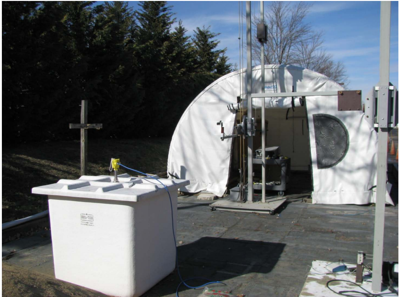
Photograph 50: 1/2" Standpipe Antenna Rear View Fiberglass Tank
