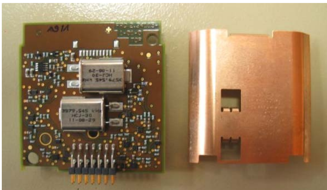
Photograph 7: Frequency Control Board (Component Side)
