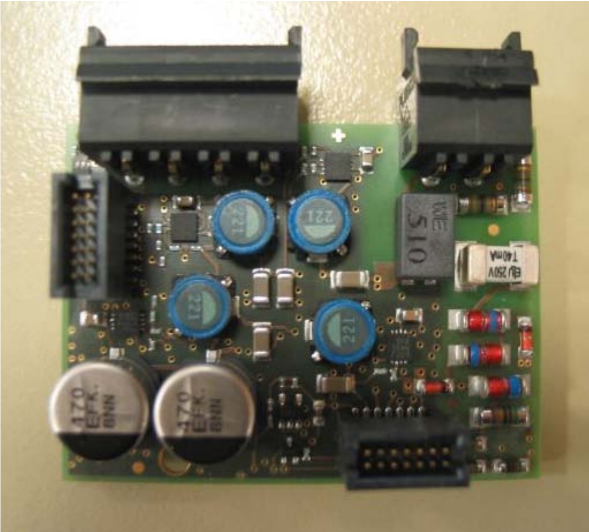
Photograph 3: Power Supply Board (Component Side)
