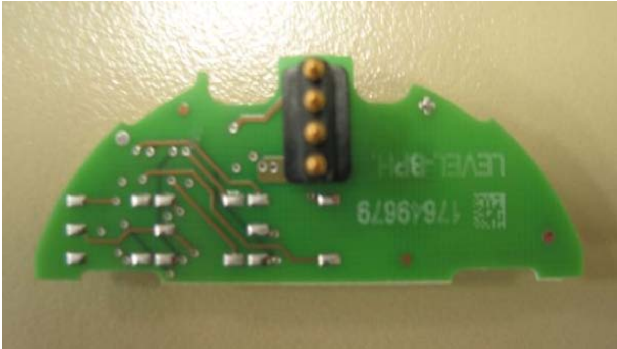
Photograph 1: Adjustment Board (Component Side)
