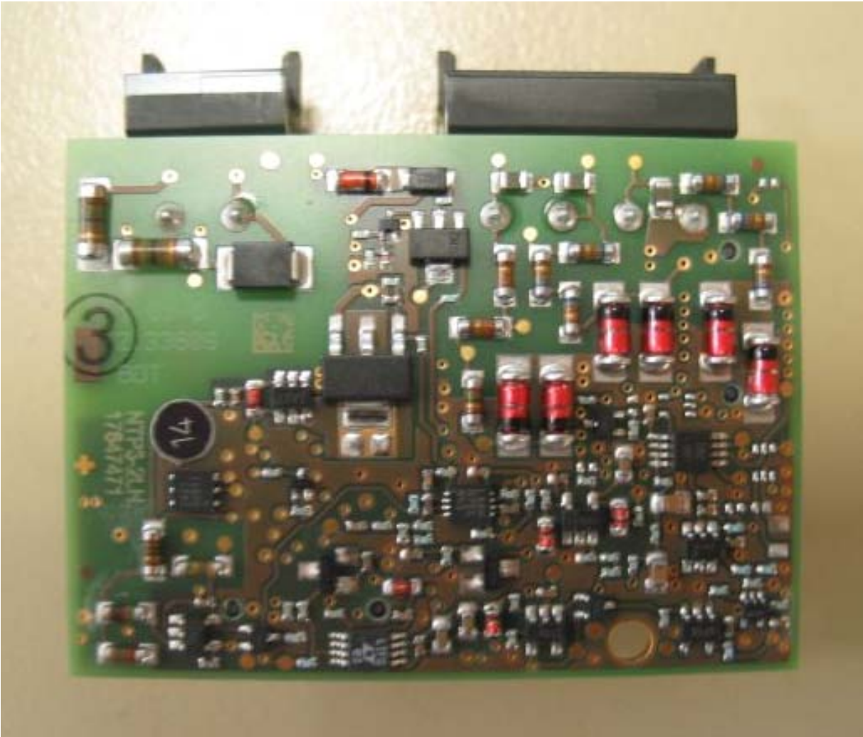
Photograph 4: Power Supply Board (Solder Side)
