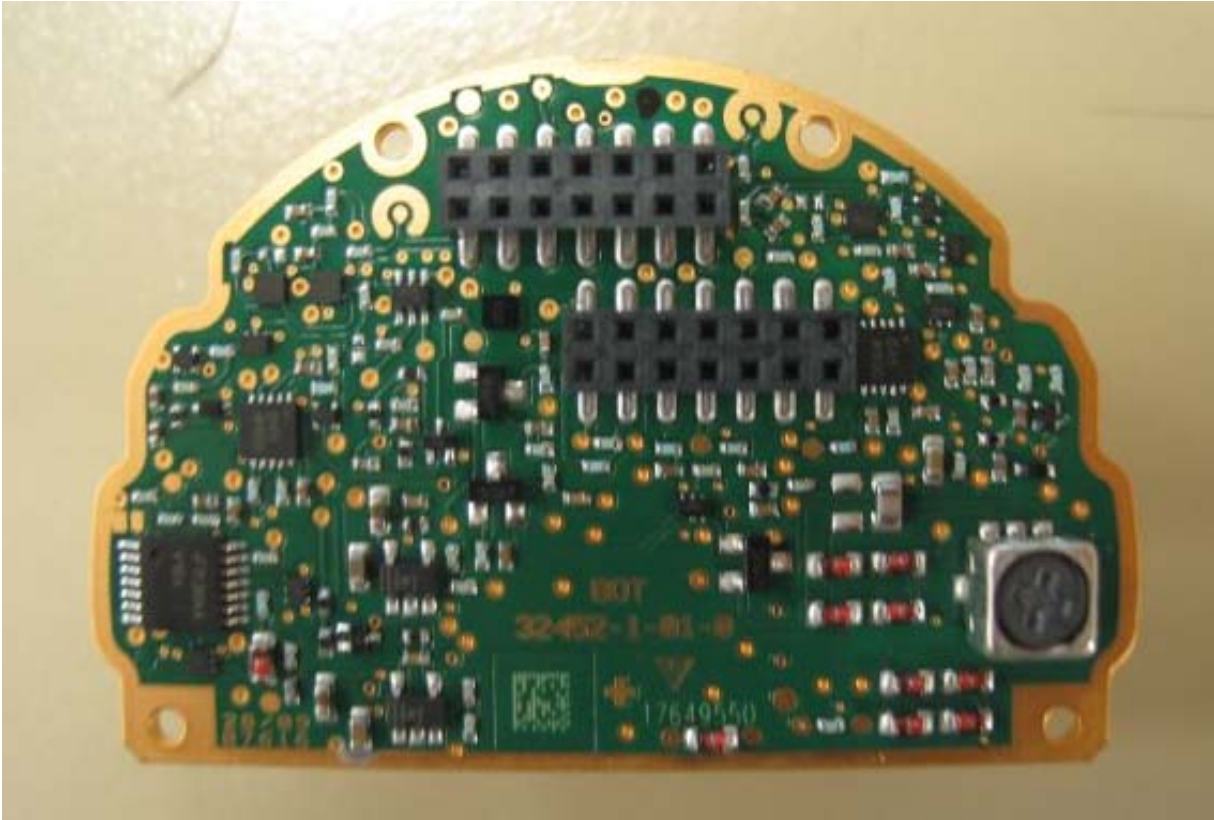
Photograph 10: Microwave Board (Component Side)
