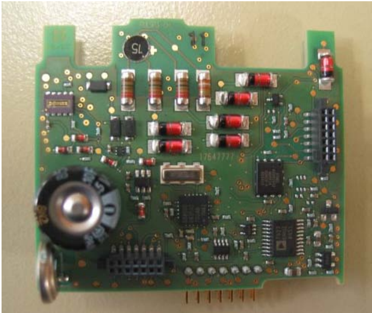
Photograph 6: CPU Board (Solder Side)
