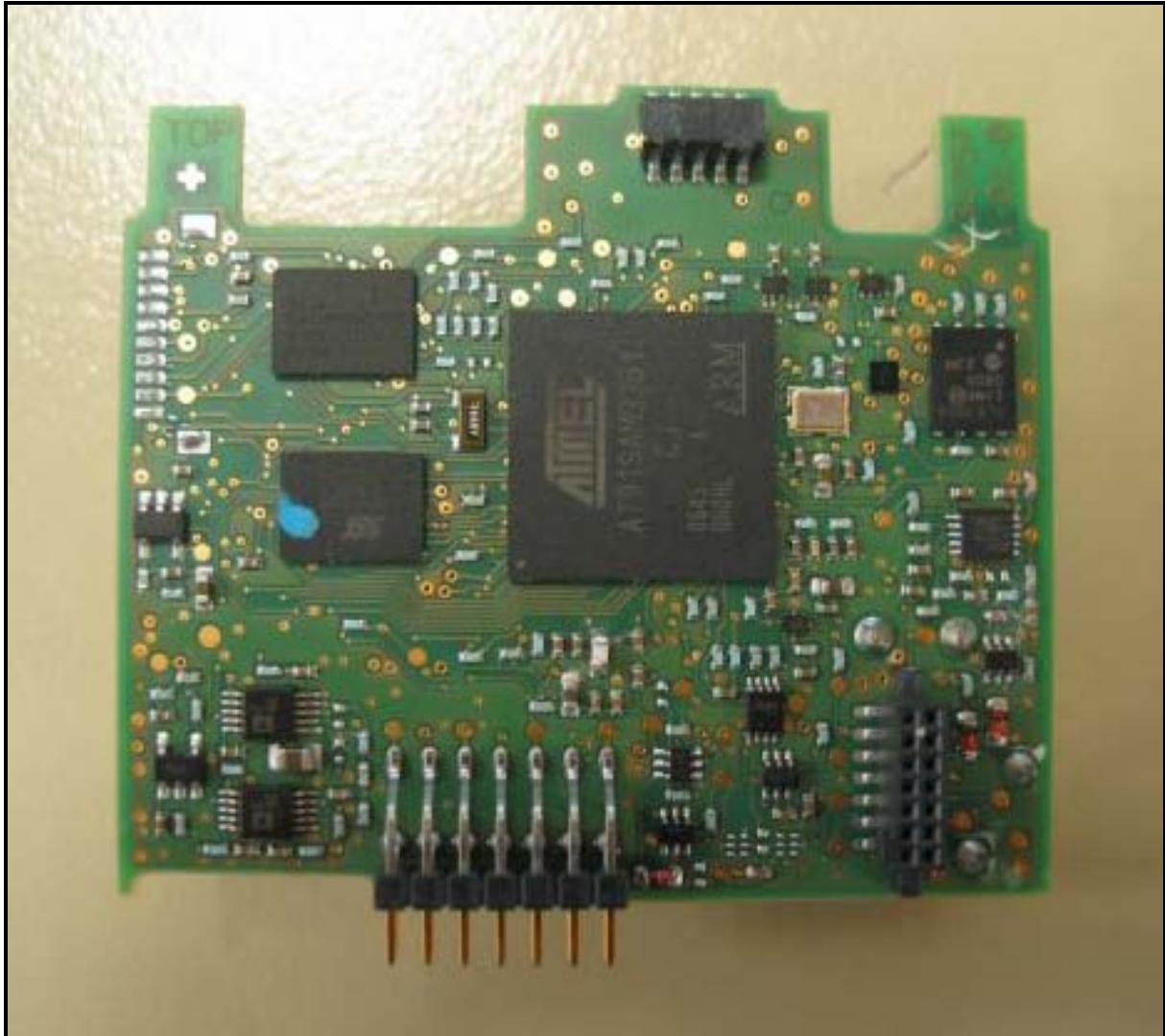
Photograph 5: CPU Board (Component Side)
