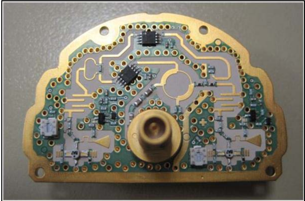
Photograph 12: Microwave Board (Solder Side)
