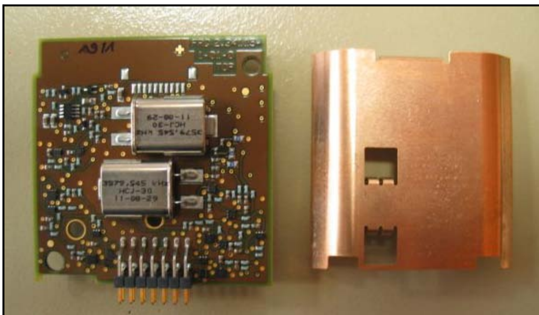
Photograph 7: Frequency Control Board (Component Side)
