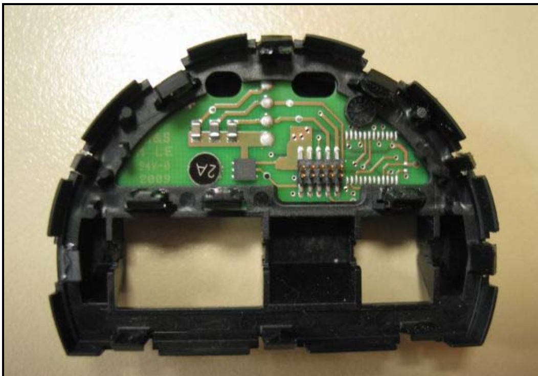
Photograph 16: Electronics Cover (Solid Side)
