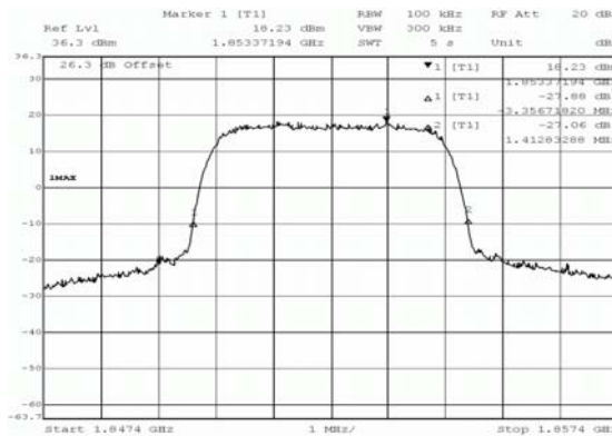
HSUPA FDD 2 Band
