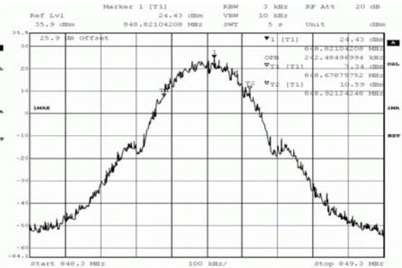
Title: bandwidth measurement Comment A1: DE1015003, G2008850, occupied bandwidth (99%), channel 251 (848.8MHz) Date: 14.JUL.2014 21:24:36
