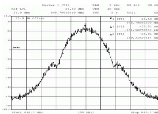
Title: bandwidth measurement Comment A1: DE1015003, E2008850, 26dB bandwidth, channel 251 (848.8MHz) Date: 14.JUL.2014 21:24:13
