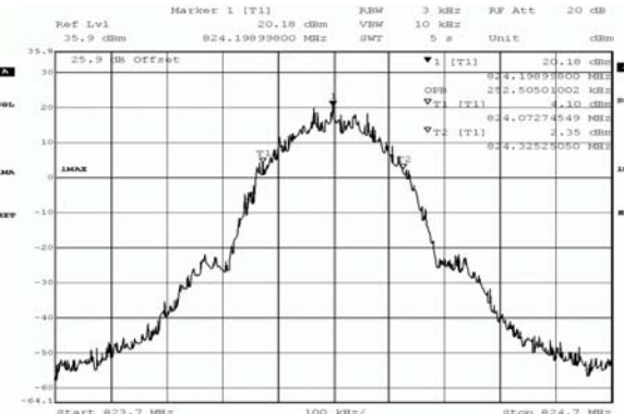
Title: bandwidth measurement Comment A1: DE1015003, E2008850, occupied bandwidth (99%), channel 129 (824.2MHz) Date: 15.JUL.2014 23:08:46
