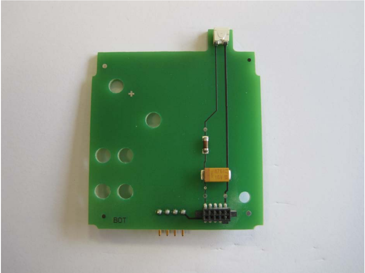
Adaptor Bottom
