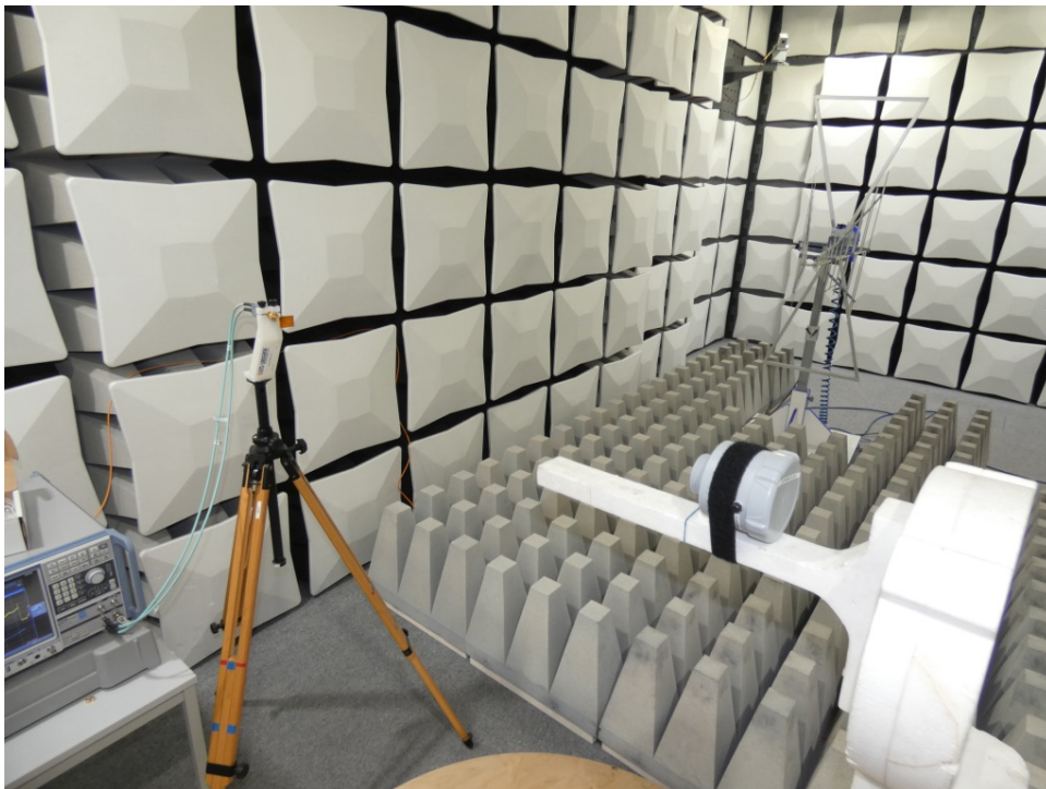
Photo 5-8: Test setup for radiated measurements (fully anechoic chamber, CFR 47 Part 15, Subpart B, Subpart C)
