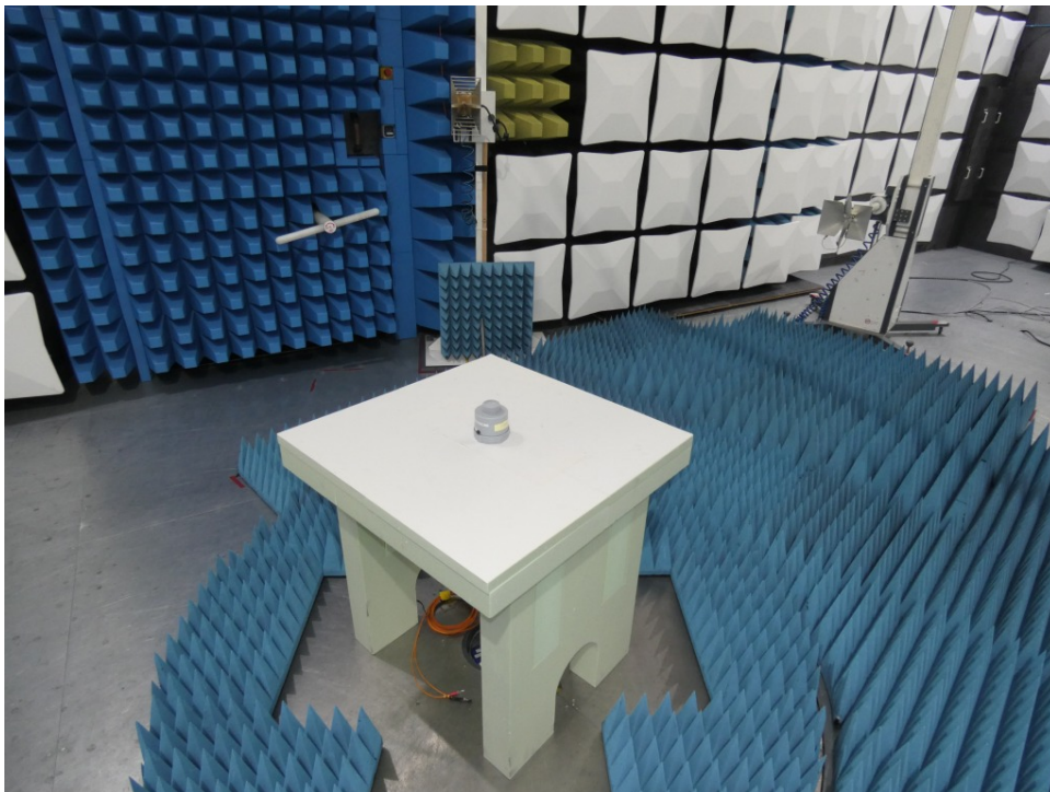
Photo 1 -4: Test setup for radiated measurements (semi anechoic chamber, CFR 47 Part 15, Subpart B, Subpart C)
