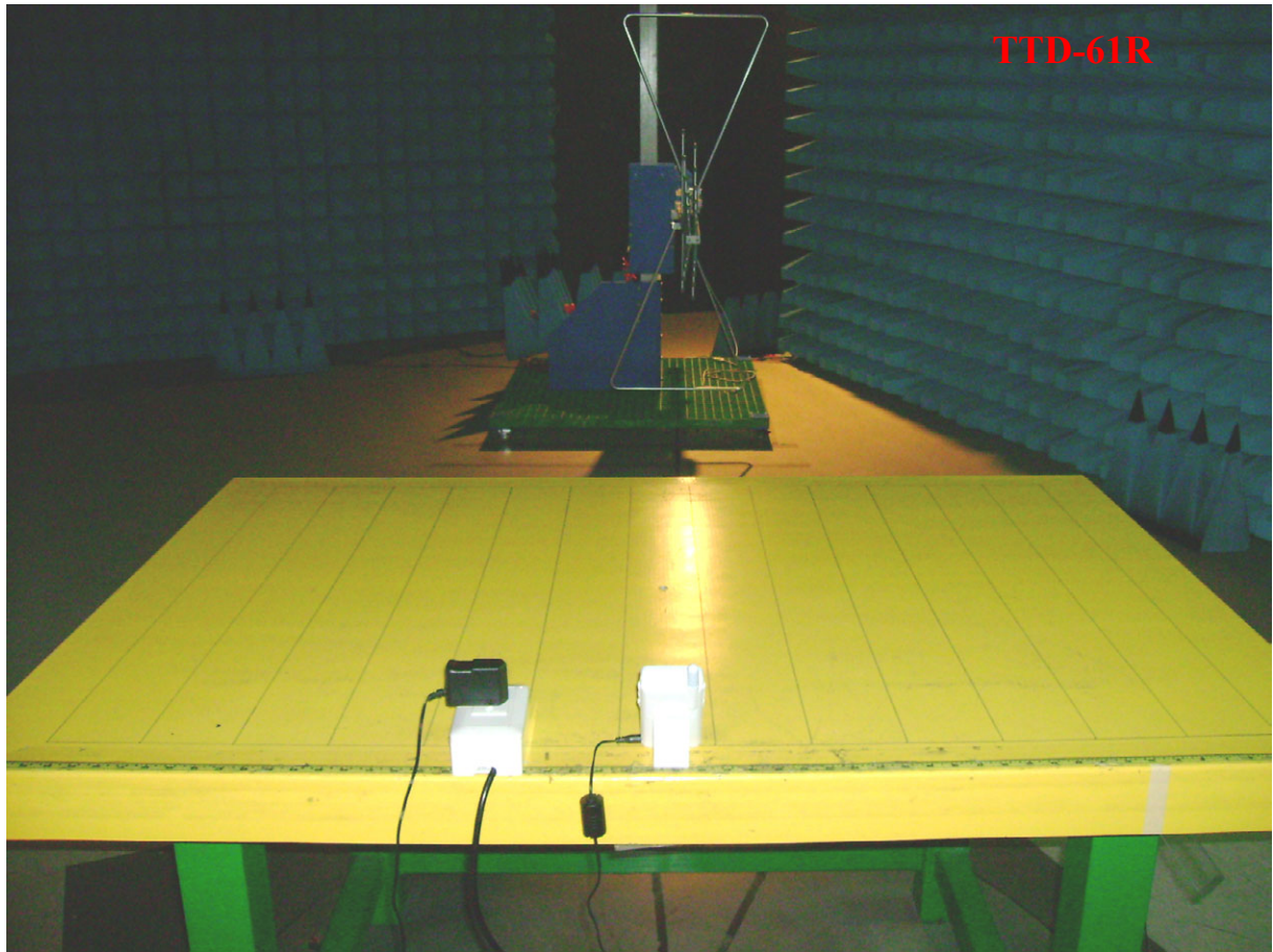
Photo 2: Radiated Emission Test set-up photo
