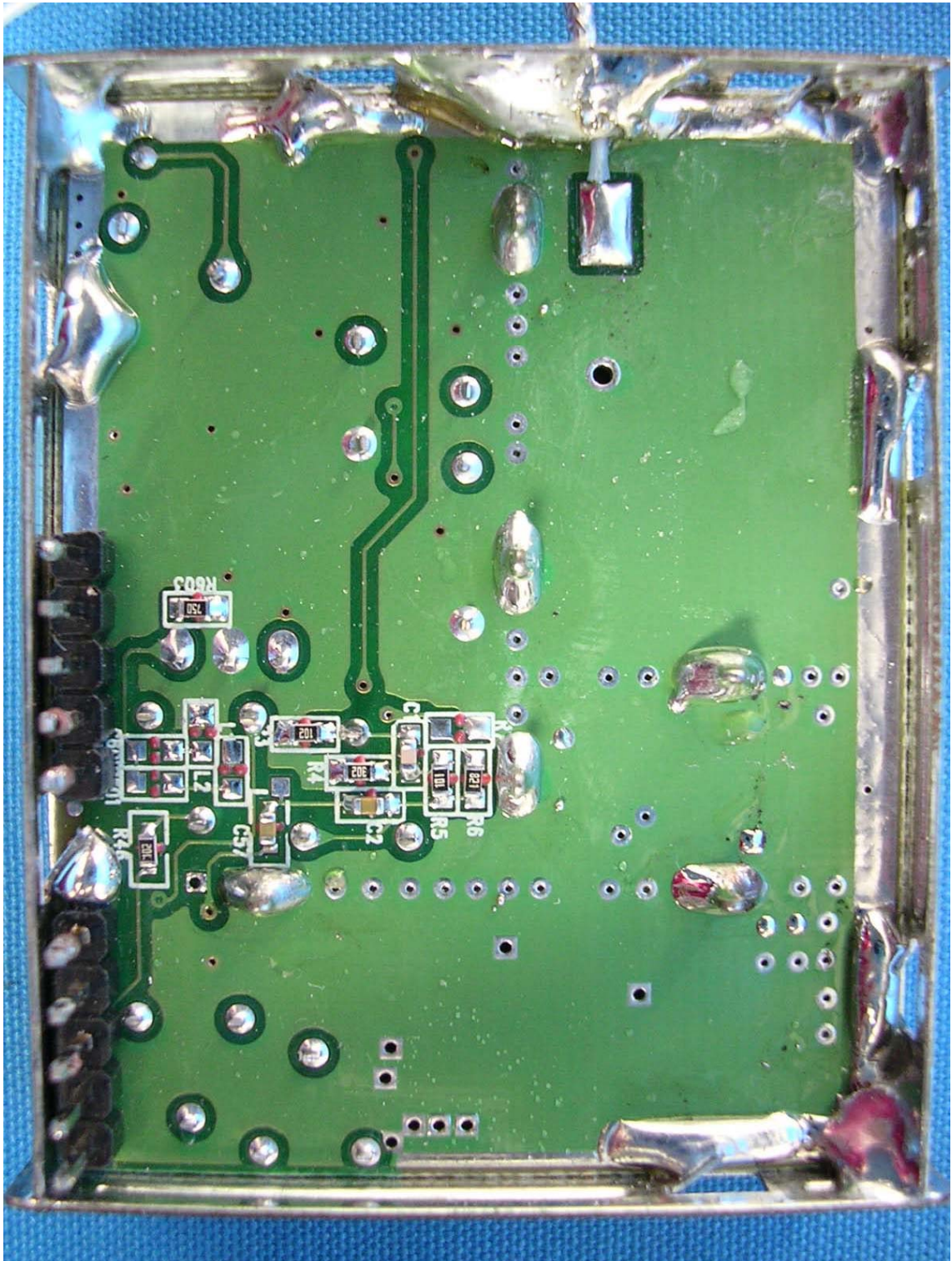
(23) EUT Photo
