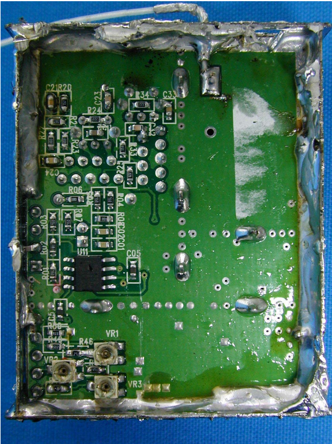
(22) EUT Photo—(Mode 1)
