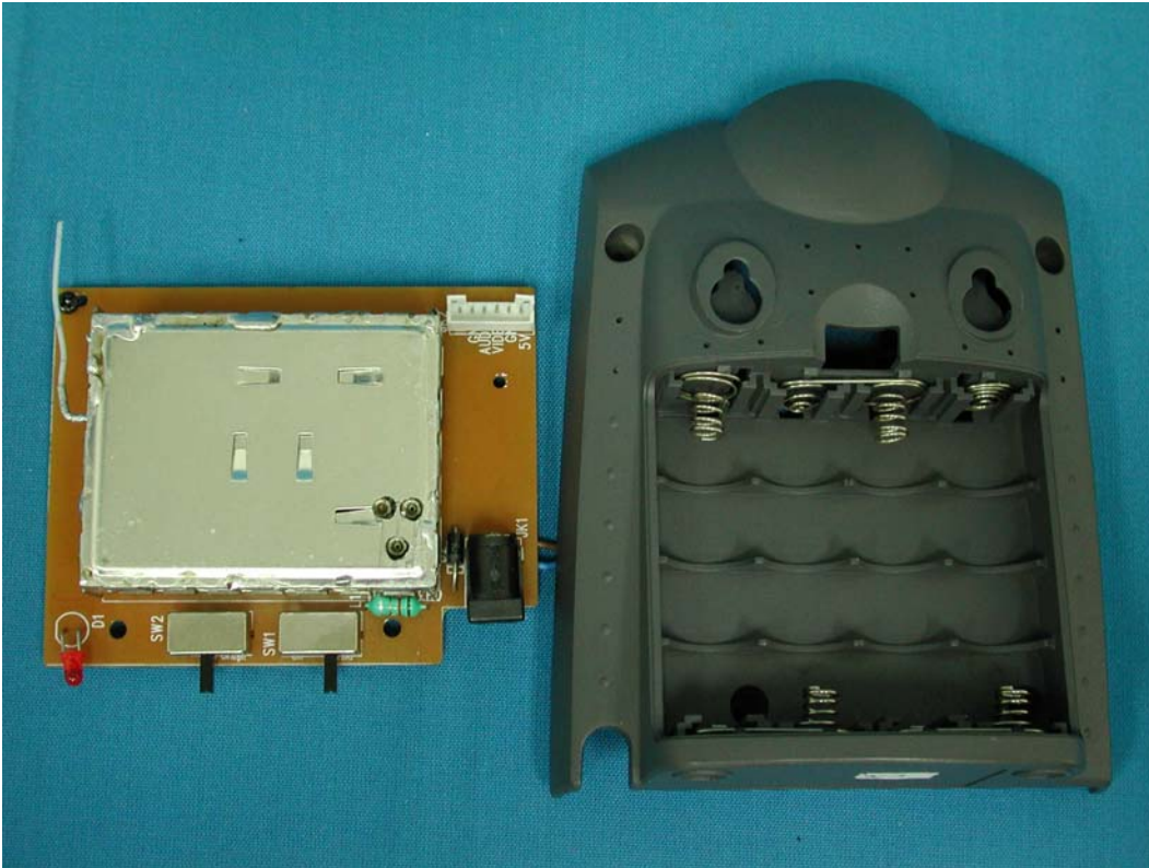
(37) EUT Photo—(Mode 2)
