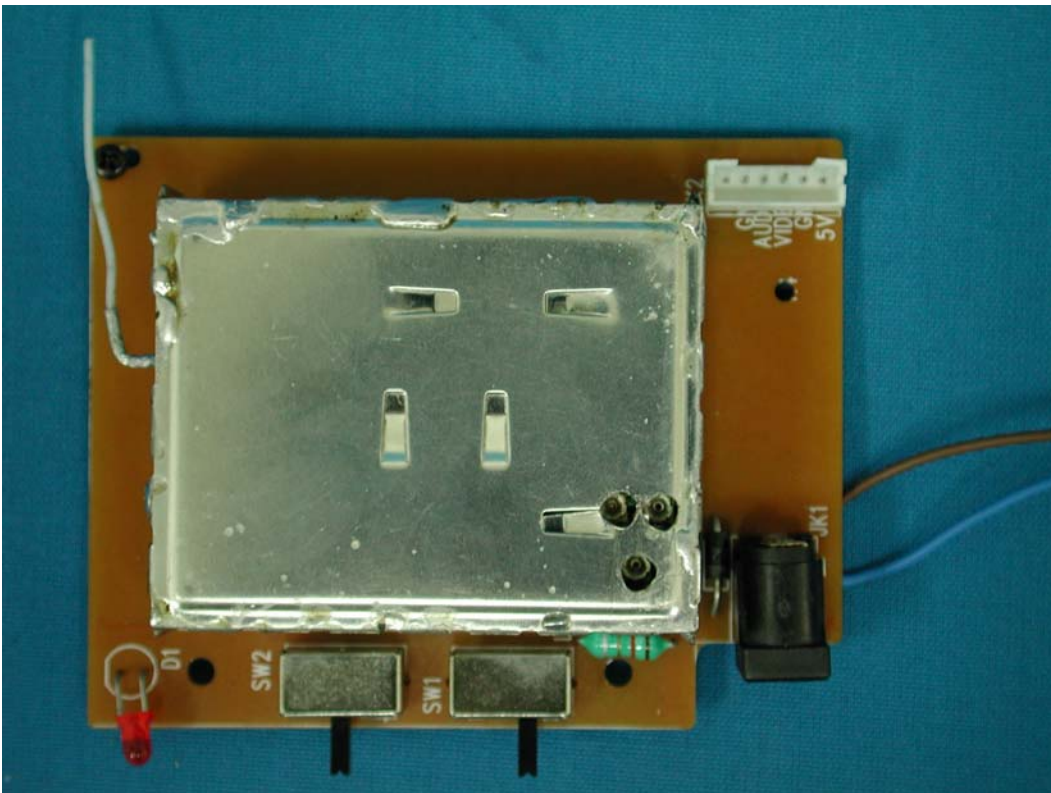
(37) EUT Photo—(Mode 2)
