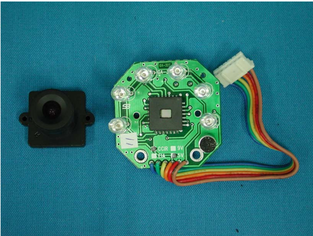
(33) EUT Photo—(Mode 2)
