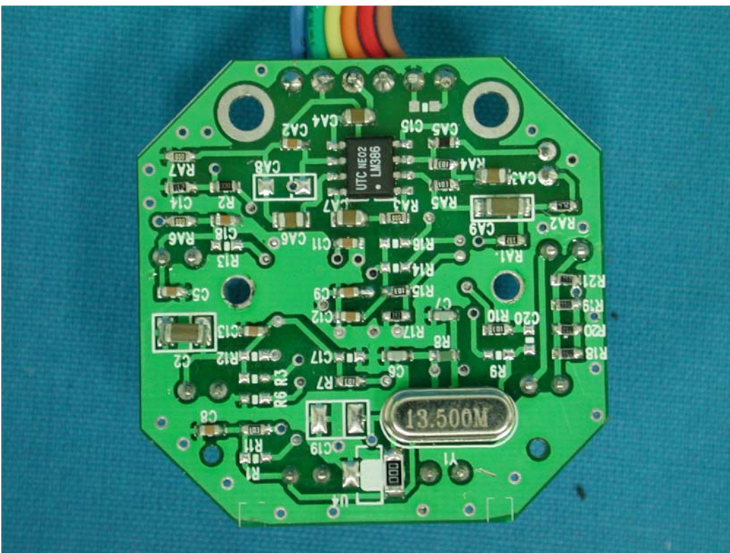
(14) EUT Photo—(Mode 1)
