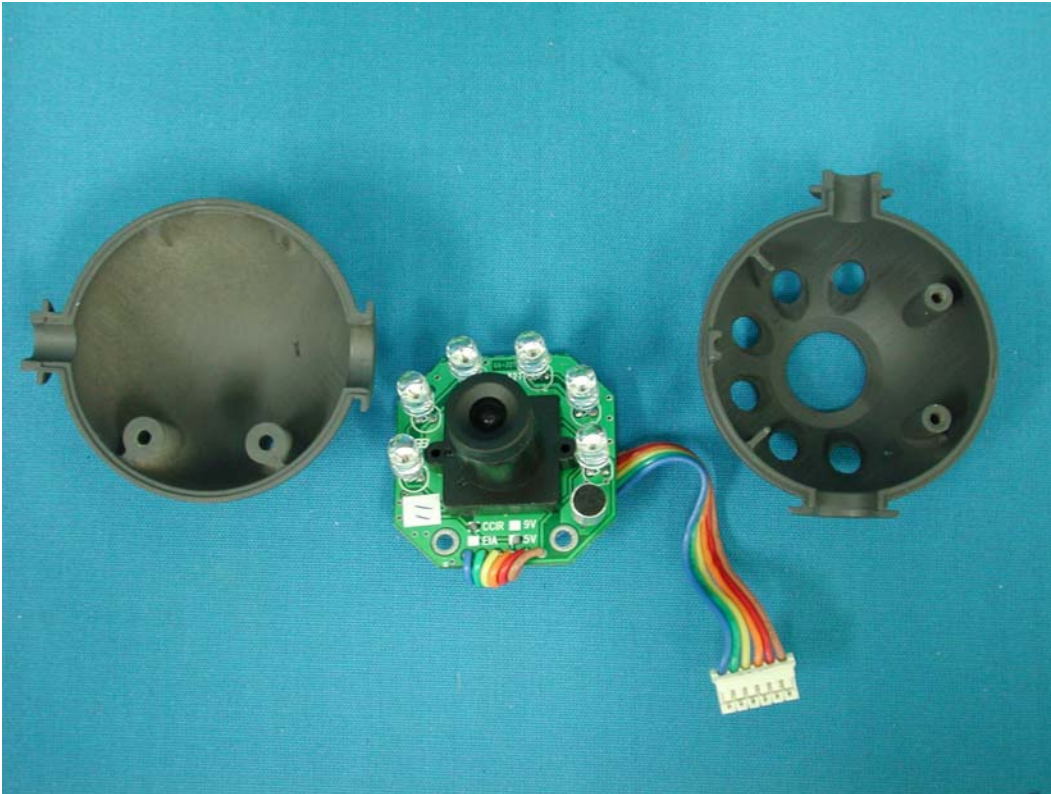
(12) EUT Photo—(Mode 1)
