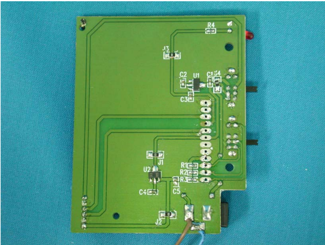
(20) EUT Photo—(Mode 1)
