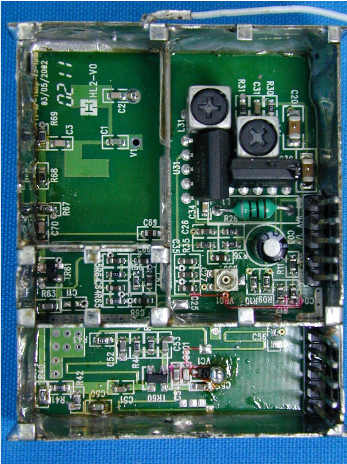
(21) EUT Photo—(Mode 1)
