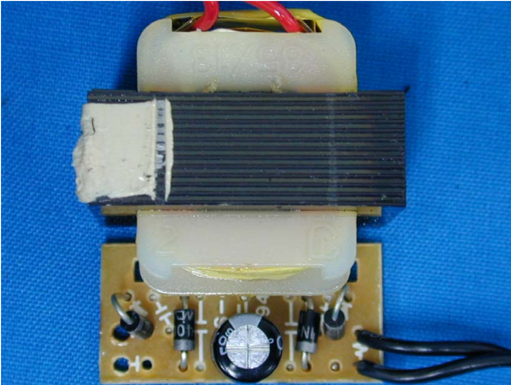
(8) EUT Photo—(Mode 1)
