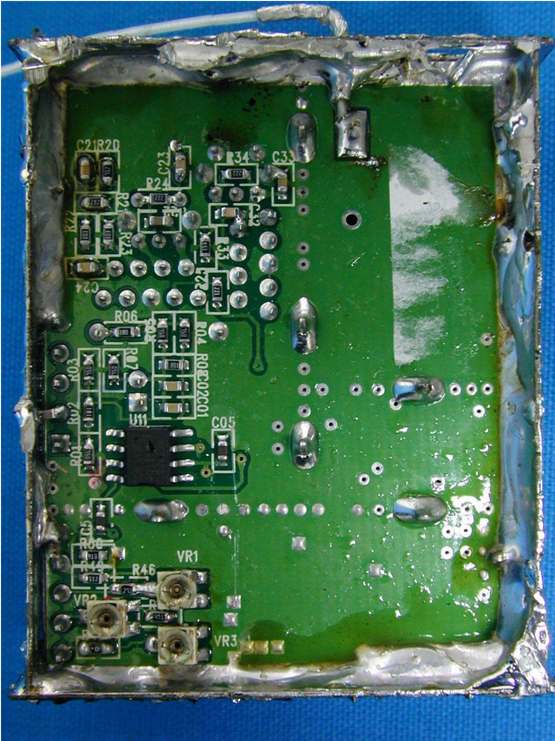
(22) EUT Photo—(Mode 1)
