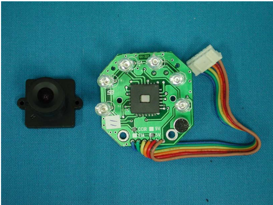
(12) EUT Photo—(Mode 1)
