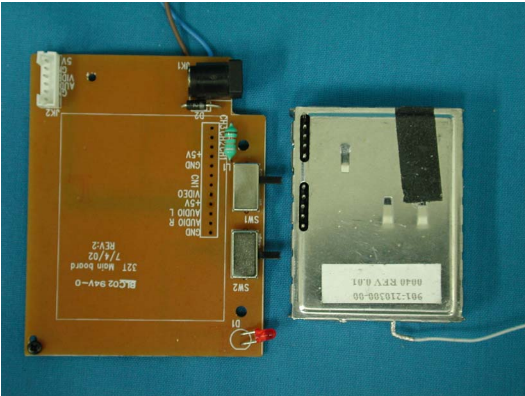
(18) EUT Photo—(Mode 1)
