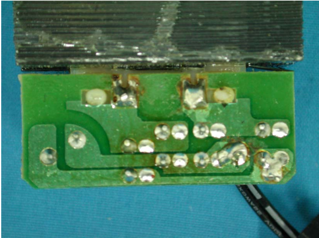
(27) EUT Photo—(Mode 2)
