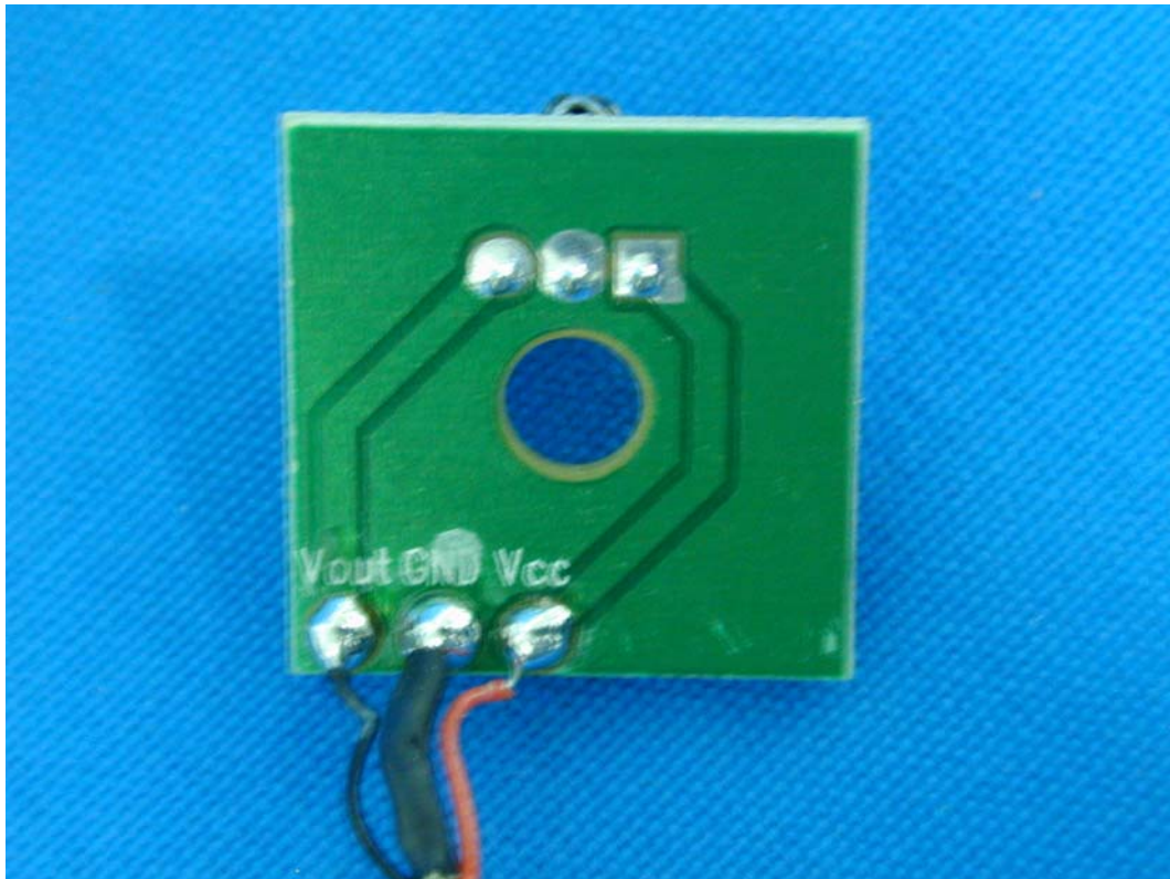
(18) EUT Photo—(Mode 1)
