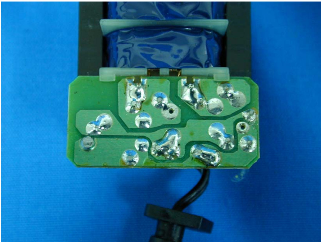
(20) EUT Photo—(Mode 1)
