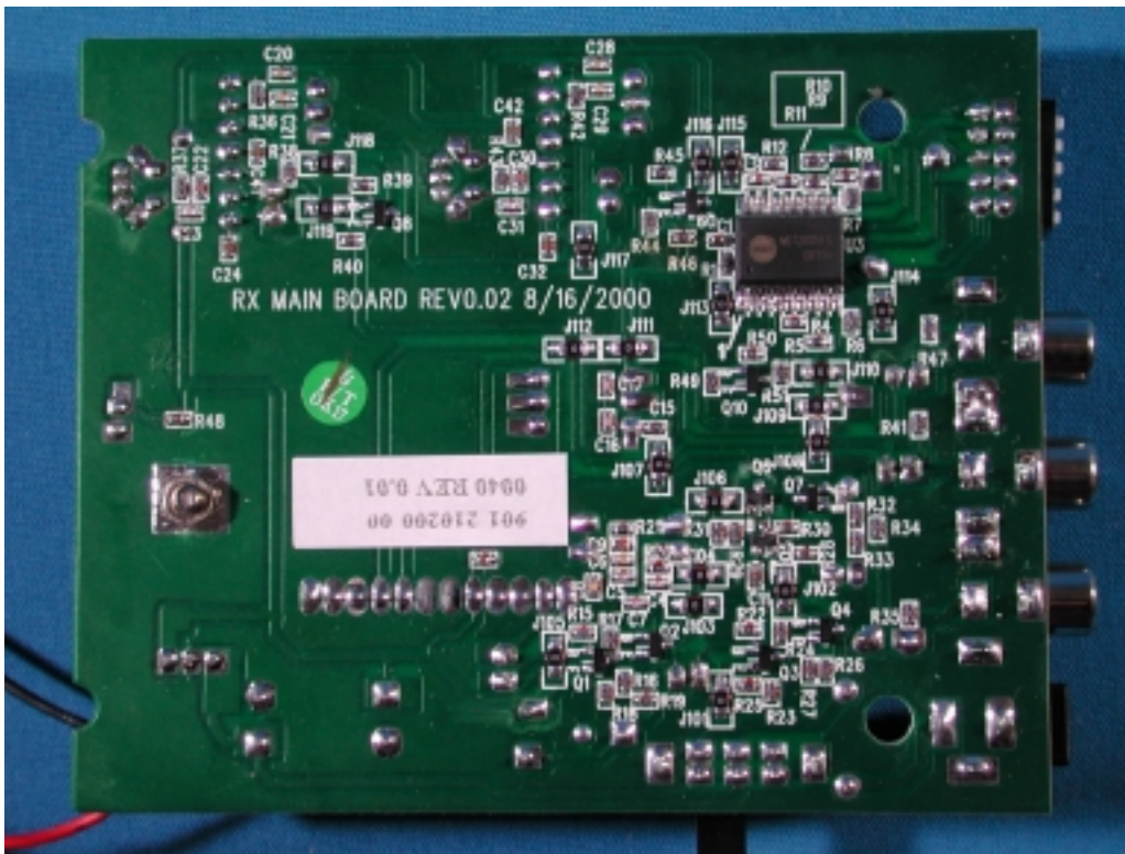
(11) EUT Photo
