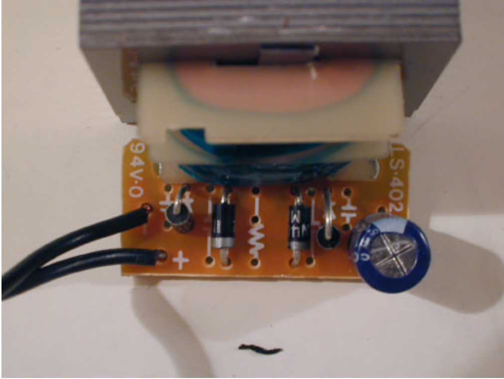
(22) Adapter Photo
